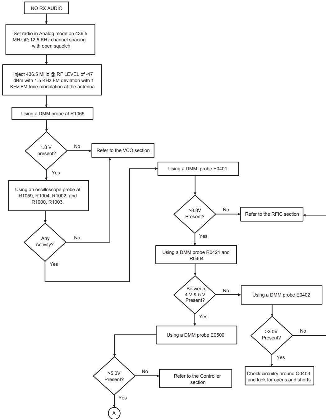
Figure 29: Troubleshooting Flow Chart for Receiver for 84012737001-A (Sheet 1 of 3)
