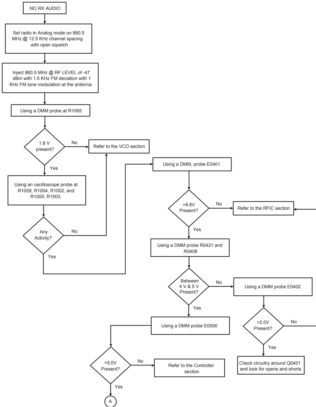
Figure 41: Troubleshooting Flow Chart for Receiver (Sheet 1 of 3)
