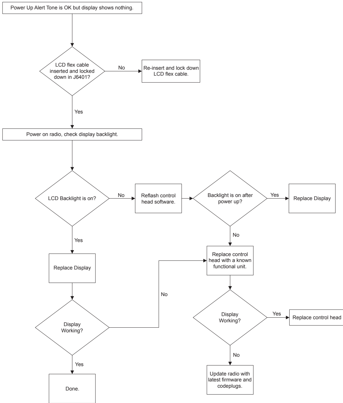
Figure 9: Troubleshooting Flow Chart for Display
