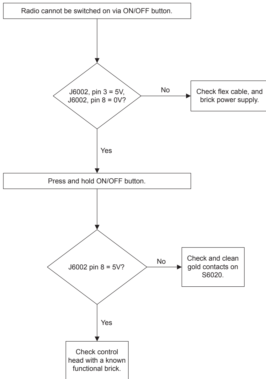
Figure 7: Troubleshooting Flow Chart for On/Off
