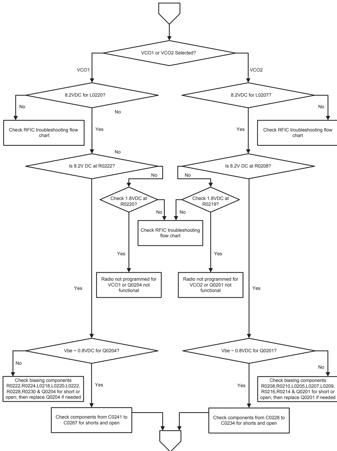
Figure 80: Troubleshooting Flow Chart for Rx VCO (Sheet 2 of 3)
