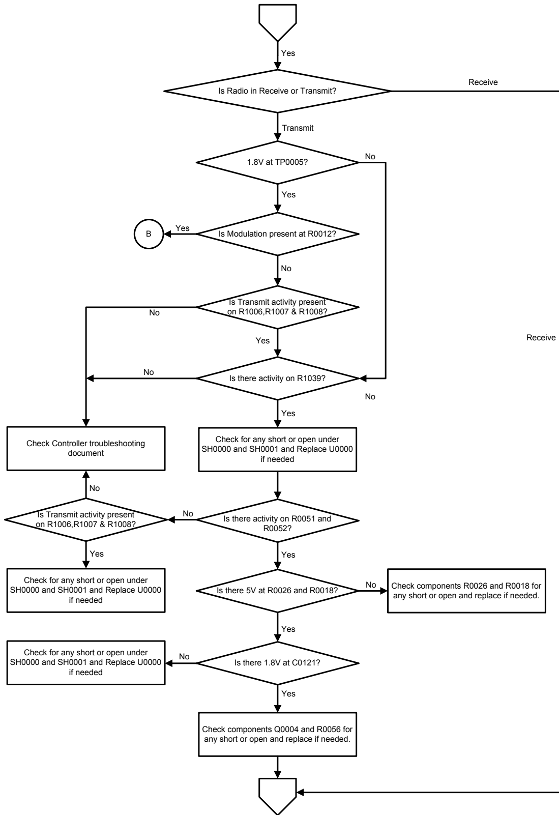
Figure 58: Troubleshooting Flow Chart for RFIC (Sheet 3 of 5)
