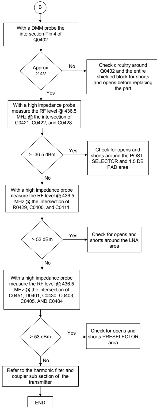
Figure 34: Troubleshooting Flow Chart for Receiver for 84012737003-C (Sheet 3 of 3)
