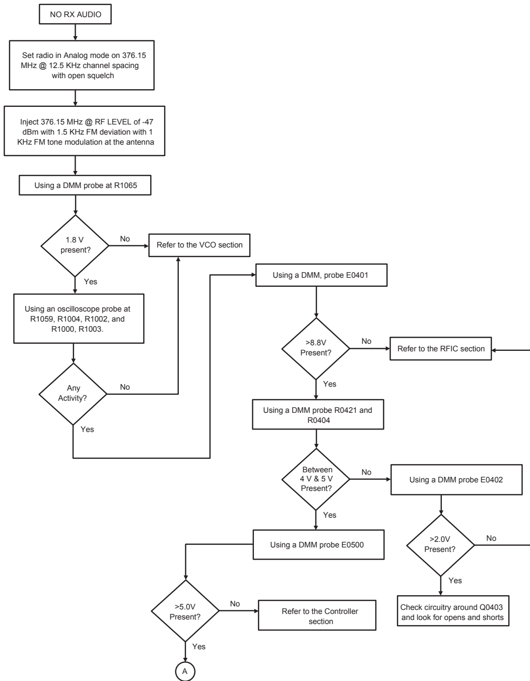
Figure 38: Troubleshooting Flow Chart for Receiver for 84012728003-C (Sheet 1 of 3)
