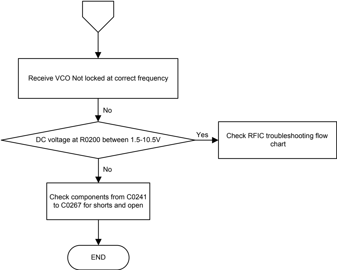
Figure 78: Troubleshooting Flow Chart for Rx VCO (Sheet 3 of 3)
