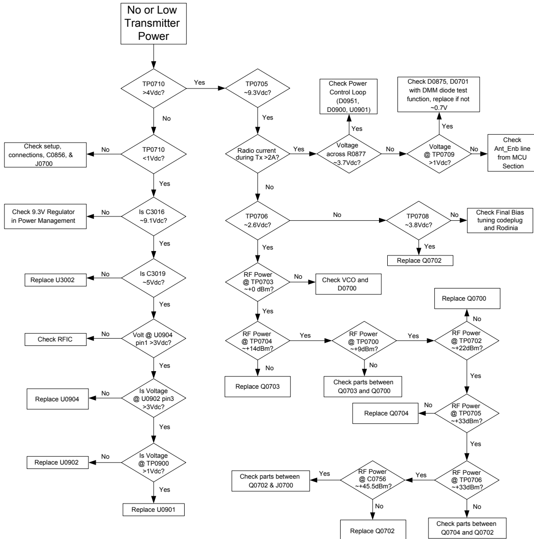
Figure 44: Troubleshooting Flow Chart for Transmitter
