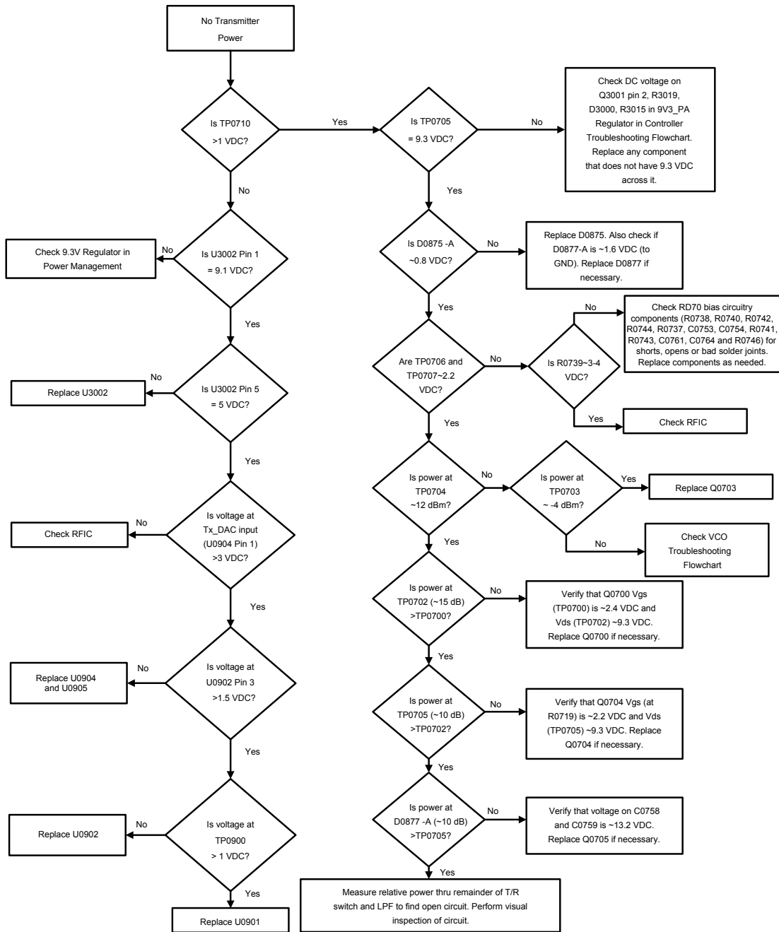
Figure 48: Troubleshooting Flow Chart for Transmitter
