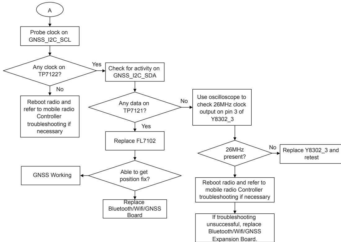
Figure 97: Troubleshooting Flow Chart for GNSS (Sheet 3 of 3)
