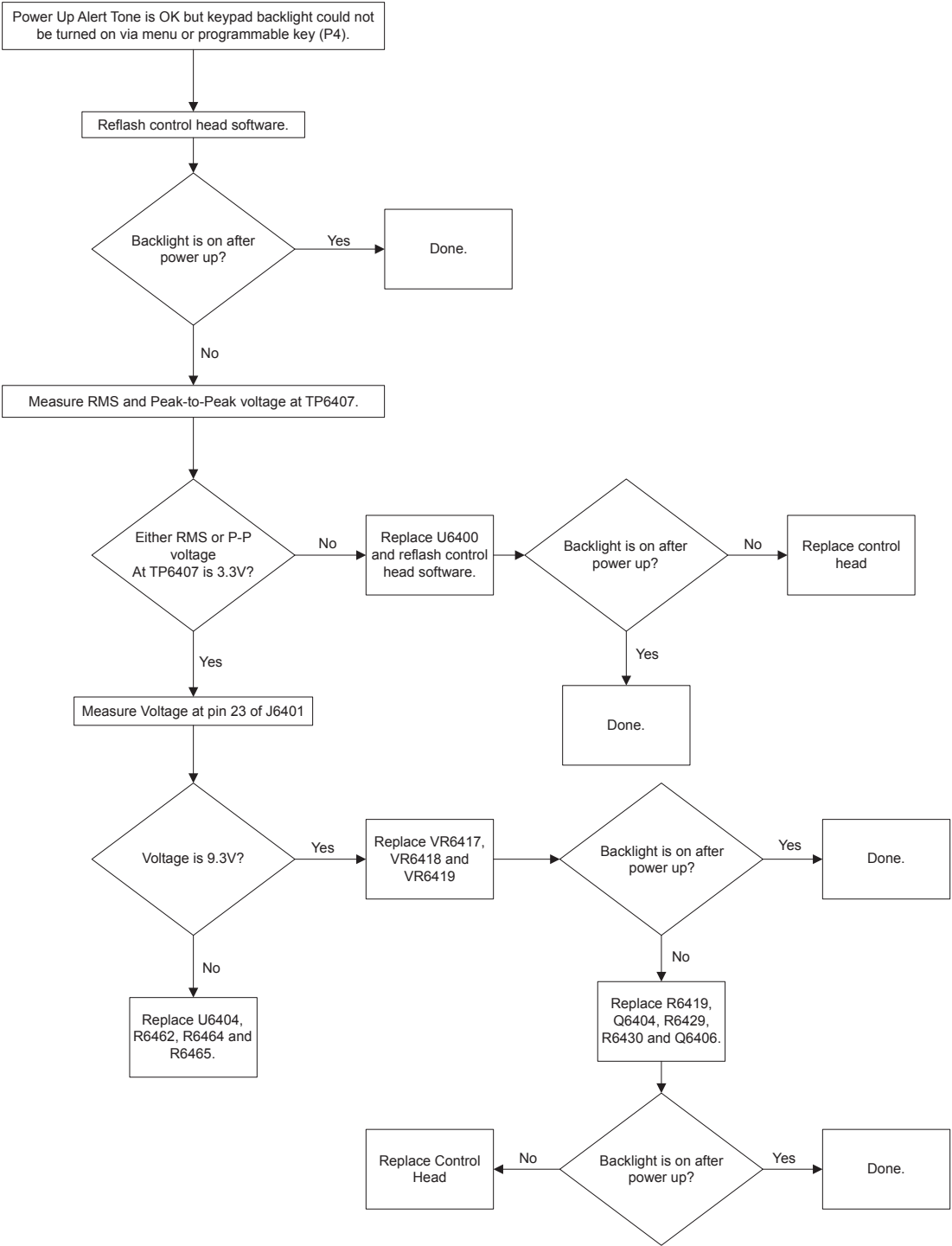
Figure 10: Troubleshooting Flow Chart for Backlight
