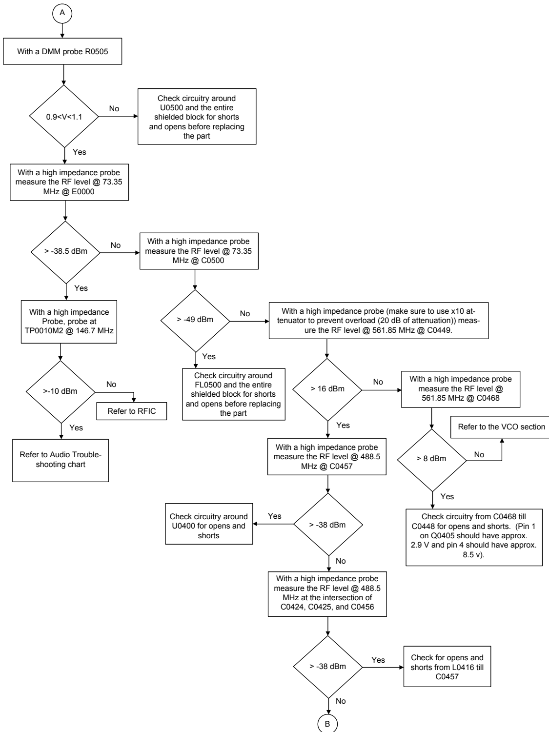
Figure 39: Troubleshooting Flow Chart for Receiver for 84012728003-C (Sheet 2 of 3)
