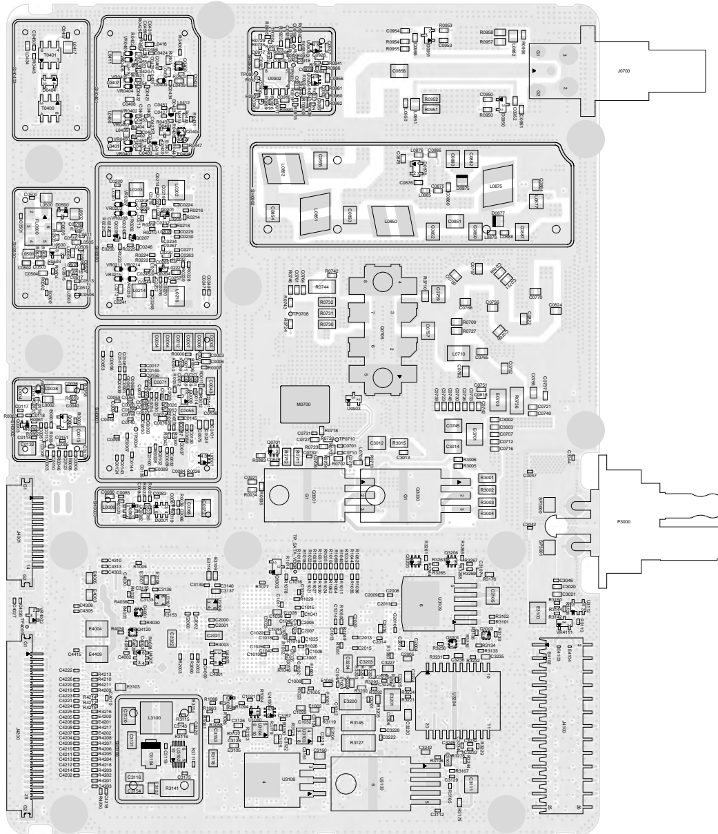
Figure 176: Main Board Top Side PCB No. 84012735001-A
