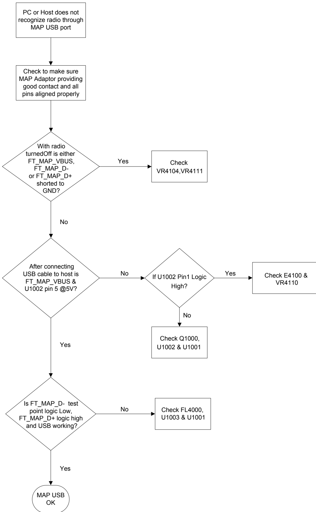
Figure 13: Troubleshooting Chart for MAP USB (Device Mode)
