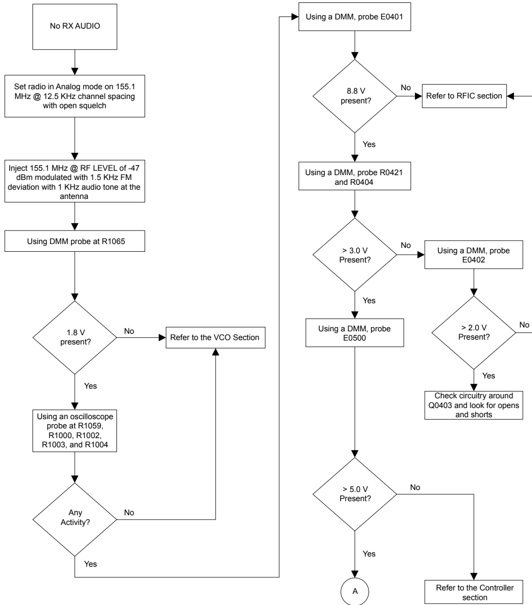
Figure 17: Troubleshooting Flow Chart for Receiver for 84012734001-A (Sheet 1 of 3)
