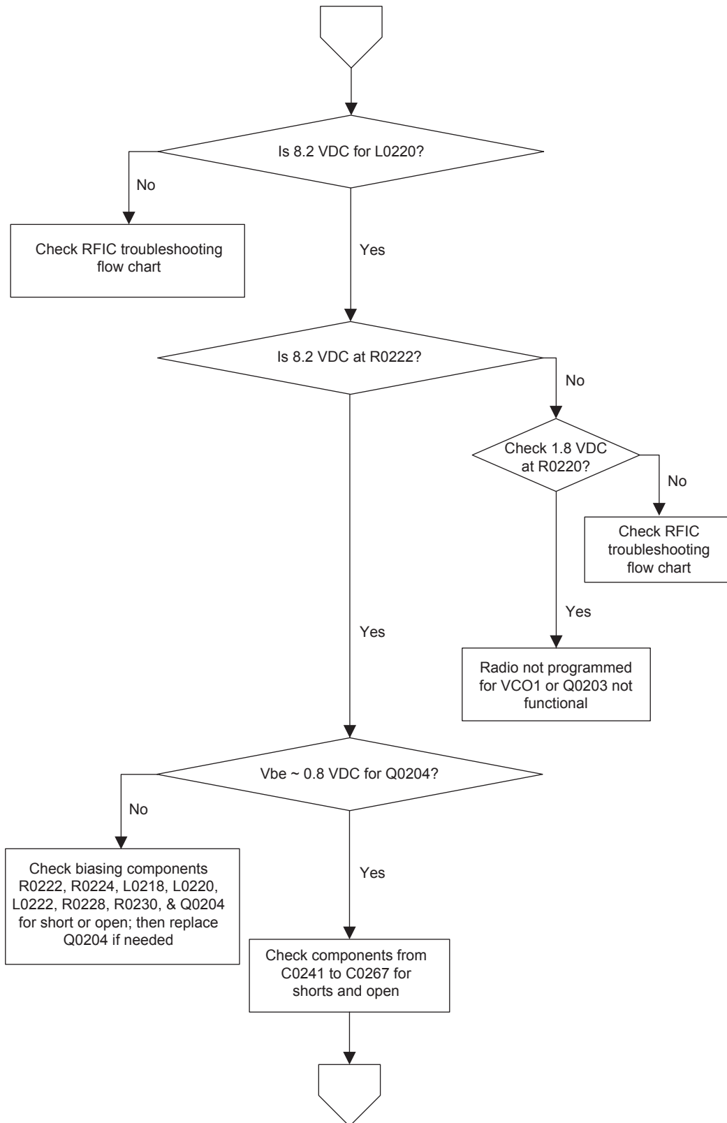
Figure 77: Troubleshooting Flow Chart for Rx VCO (Sheet 2 of 3)
