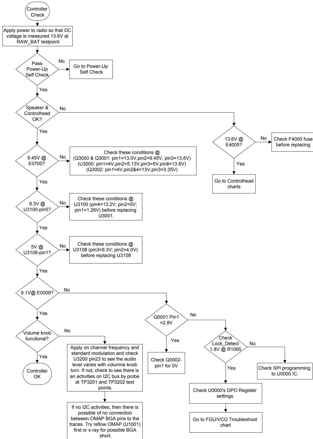
Figure 11: Troubleshooting Chart for Controller
