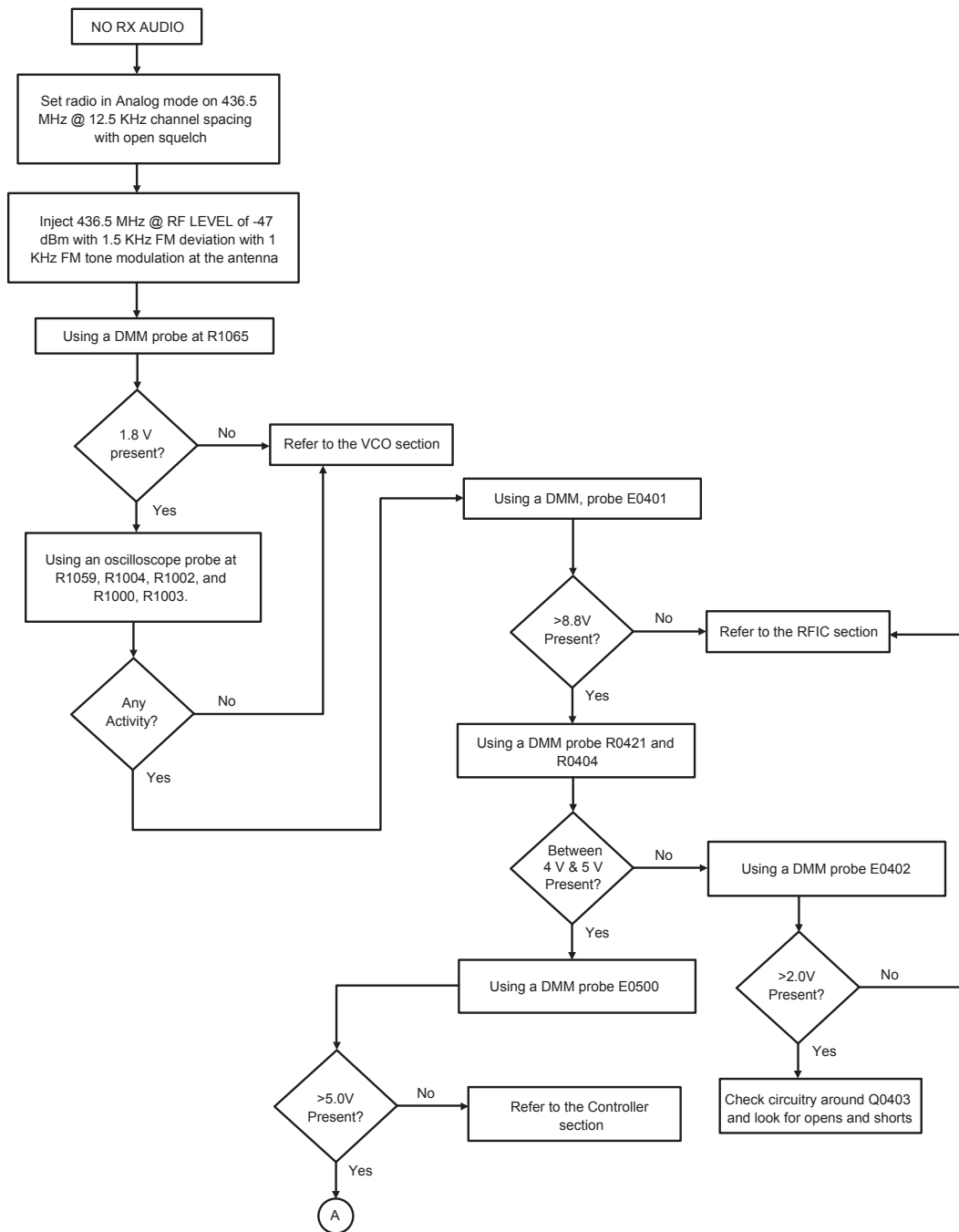
Figure 32: Troubleshooting Flow Chart for Receiver for 84012737003-C (Sheet 1 of 3)
