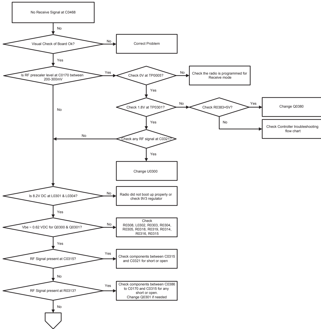
Figure 79: Troubleshooting Flow Chart for Rx VCO (Sheet 1 of 3)
