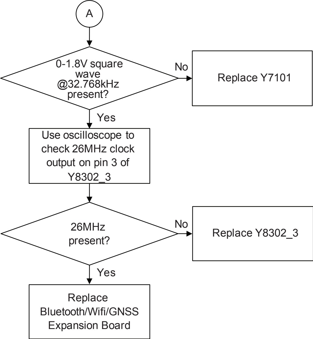
Figure 92: Troubleshooting Flow Chart for Bluetooth (Sheet 2 of 4)
