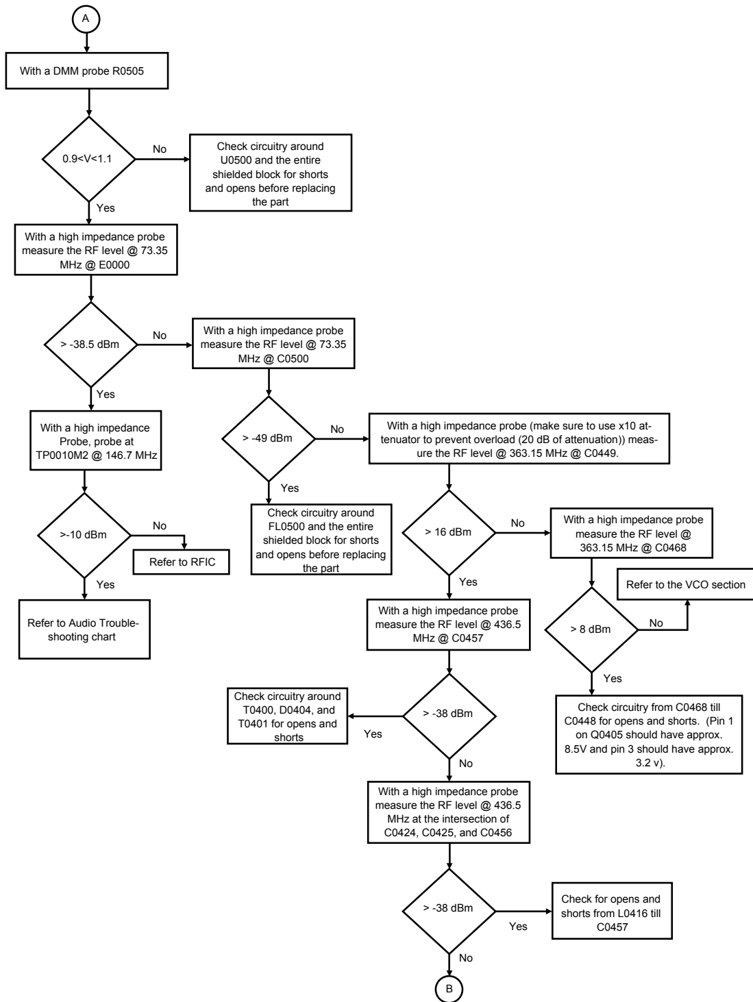
Figure 24: Troubleshooting Flow Chart for Receiver for 84012735001-A (Sheet 2 of 3)
