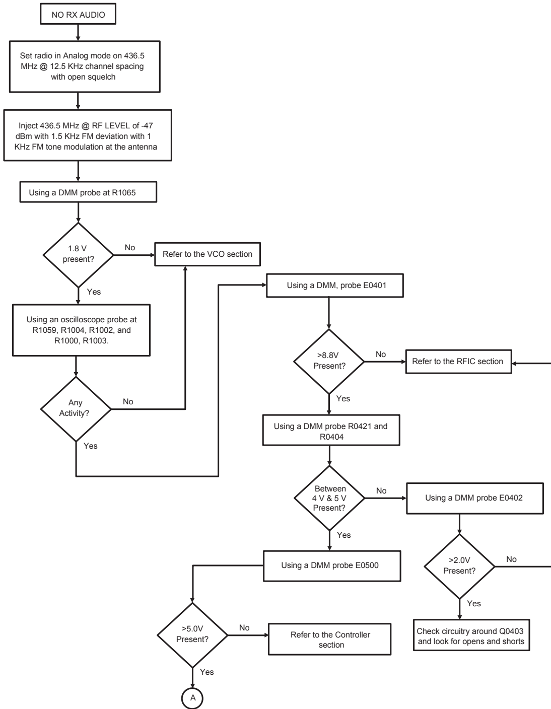
Figure 23: Troubleshooting Flow Chart for Receiver for 84012735001-A (Sheet 1 of 3)
