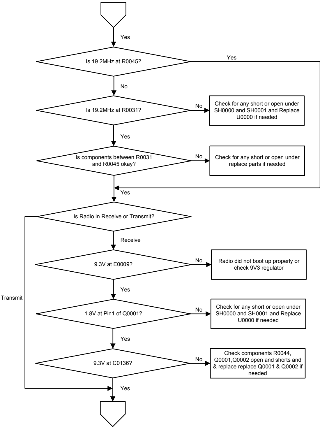
Figure 62: Troubleshooting Flow Chart for RFIC (Sheet 2 of 5)
