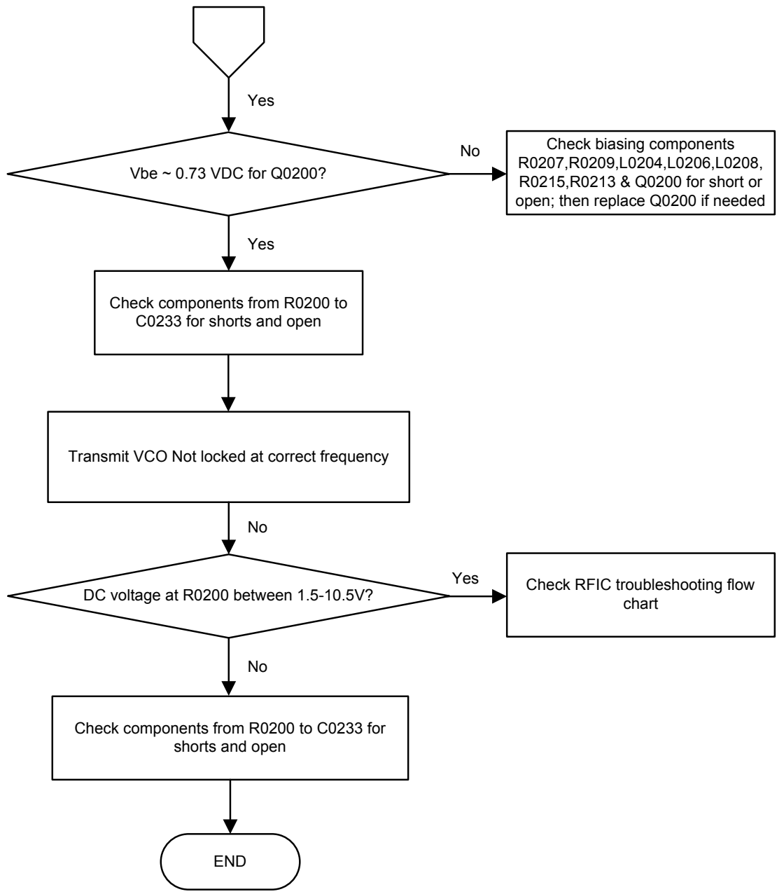
Figure 85: Troubleshooting Flow Chart for Tx VCO (Sheet 2 of 2)
