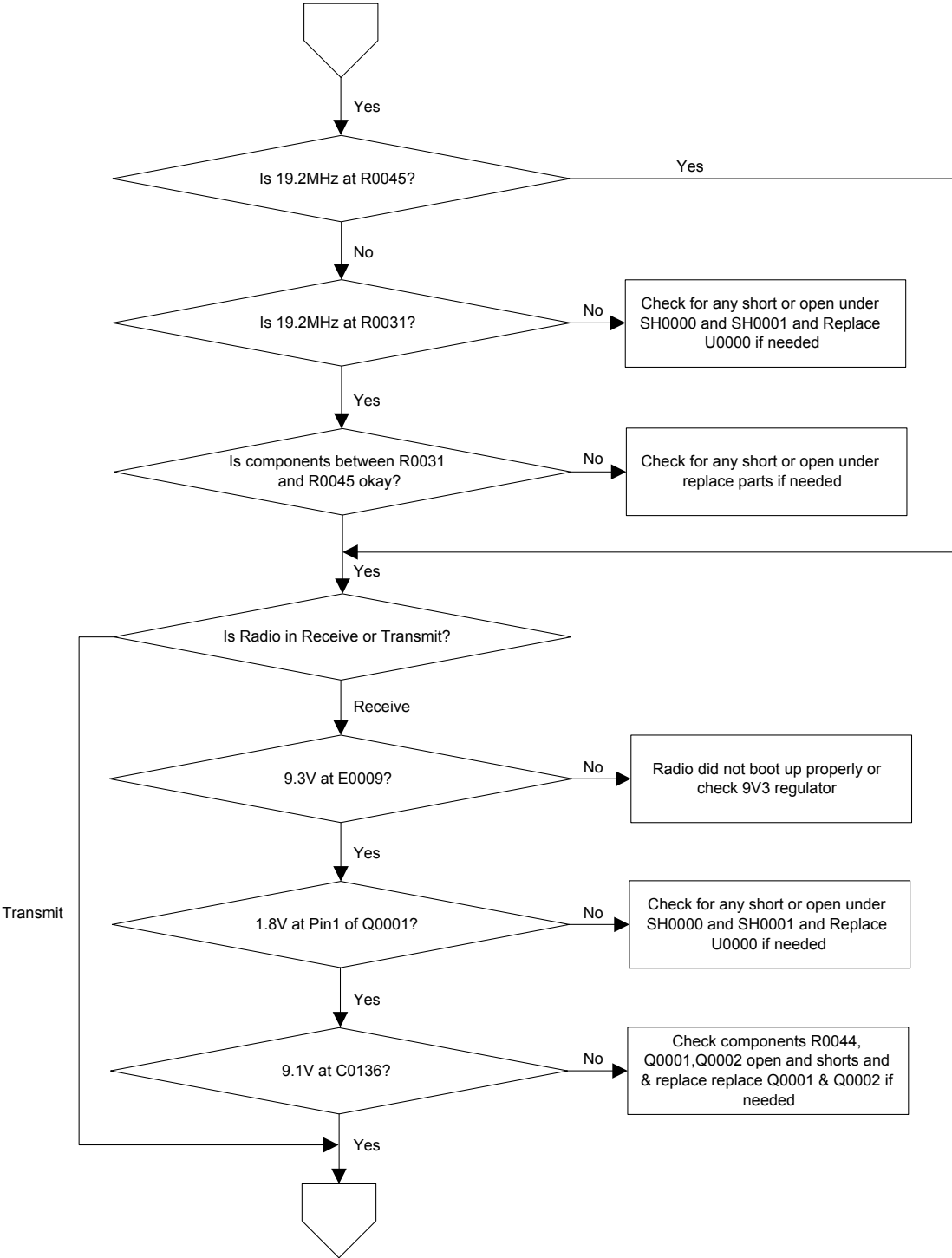
Figure 52: Troubleshooting Flow Chart for RFIC (Sheet 2 of 5)
