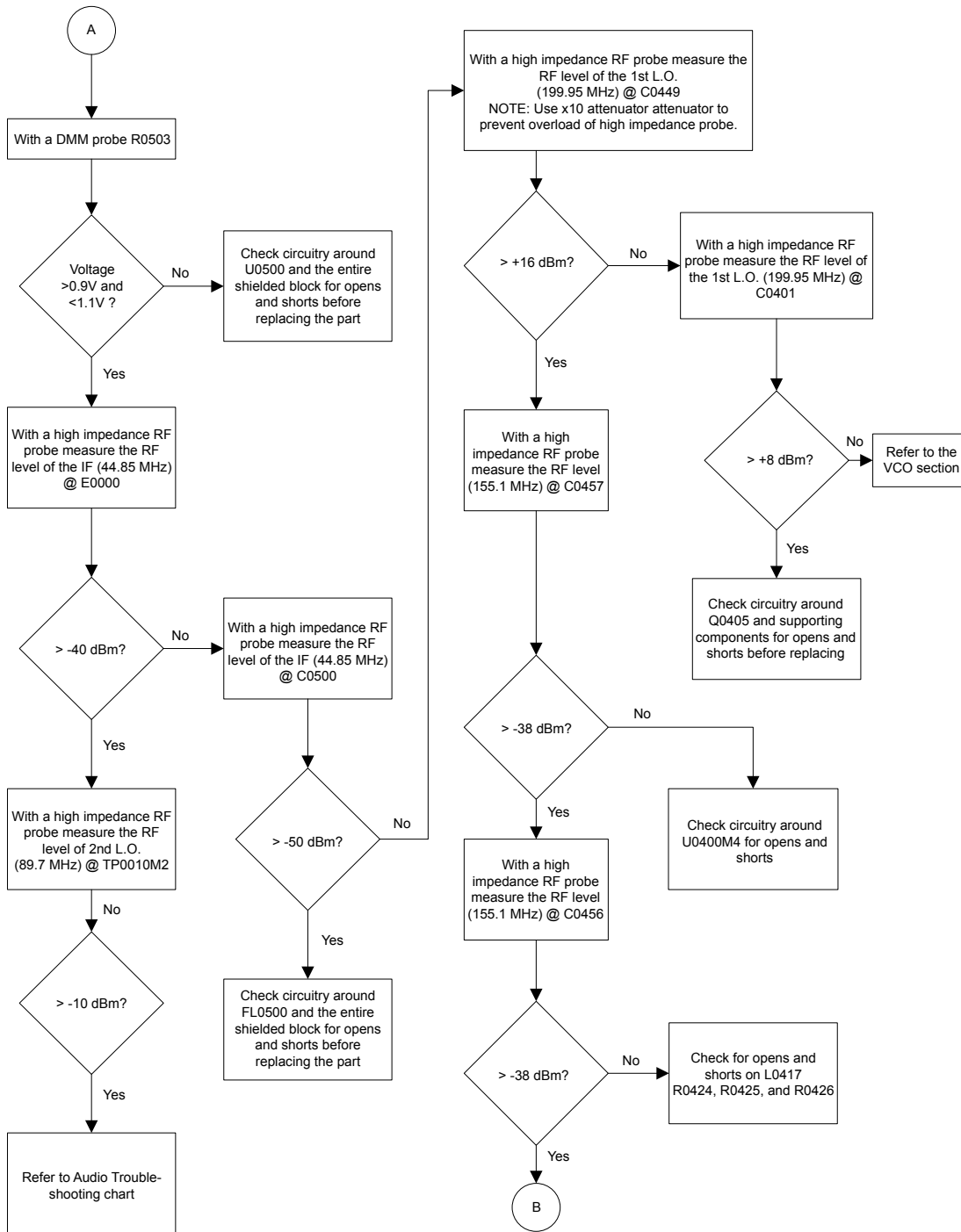
Figure 21: Troubleshooting Flow Chart for Receiver for 84012734002-B (Sheet 2 of 3)
