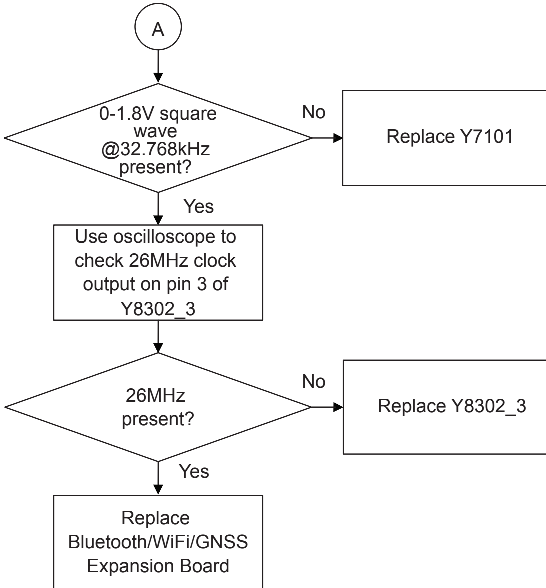
Figure 99: Troubleshooting Flow Chart for Wi-Fi (Sheet 2 of 2)
