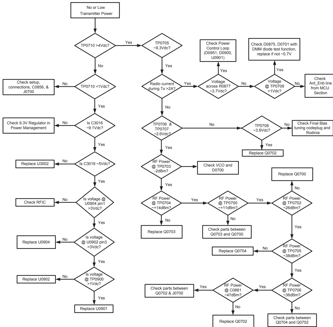
Figure 49: Troubleshooting Flow Chart for Transmitter
