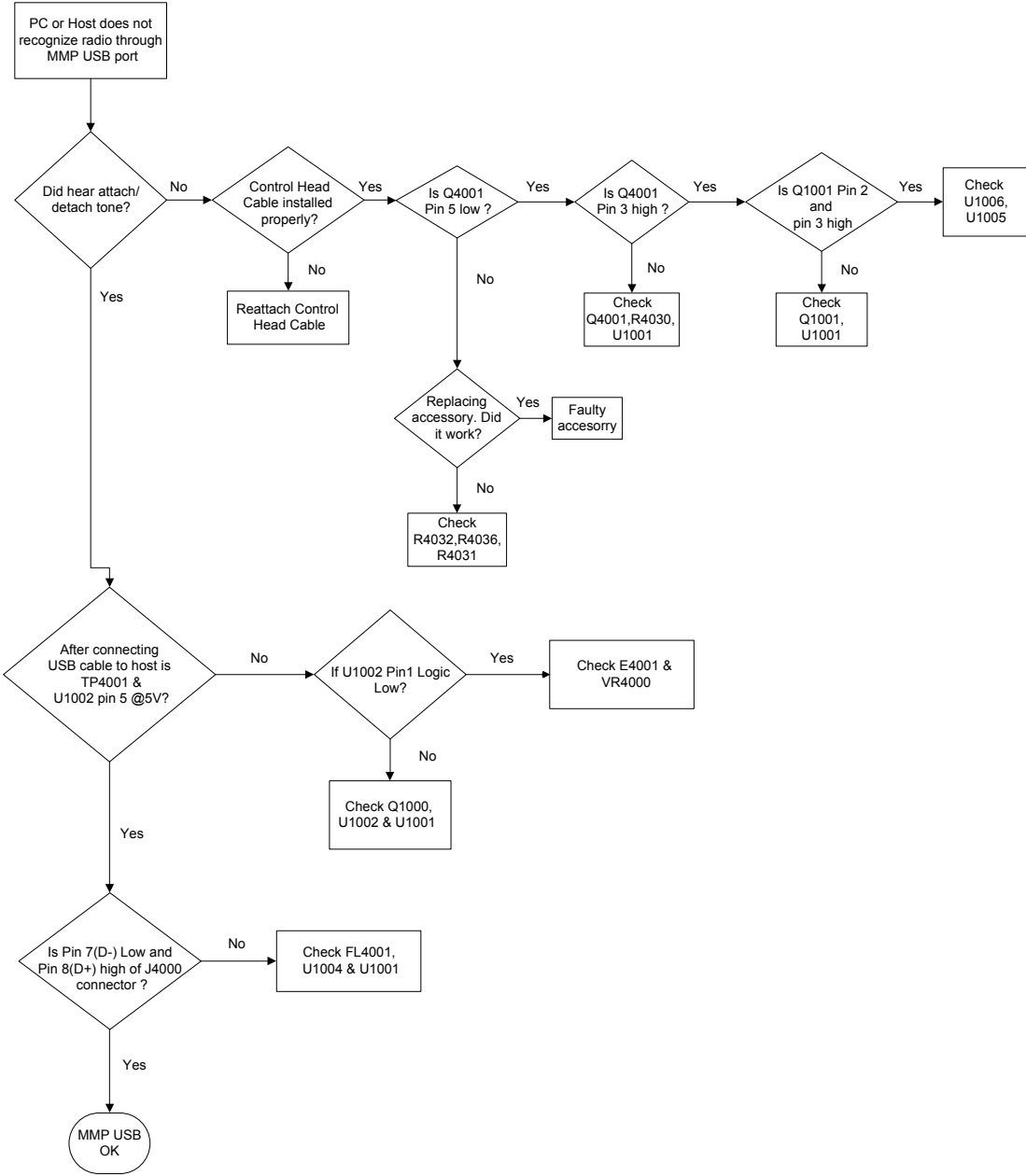
Figure 14: Troubleshooting Chart for MMP USB (Device Mode)
