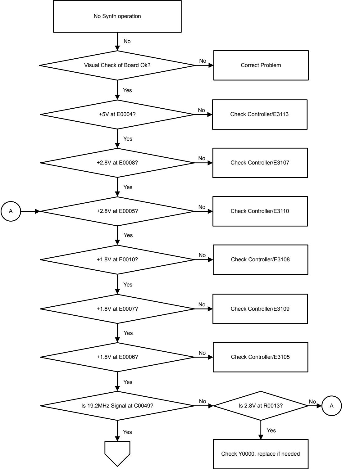
Figure 56: Troubleshooting Flow Chart for RFIC (Sheet 1 of 5)
