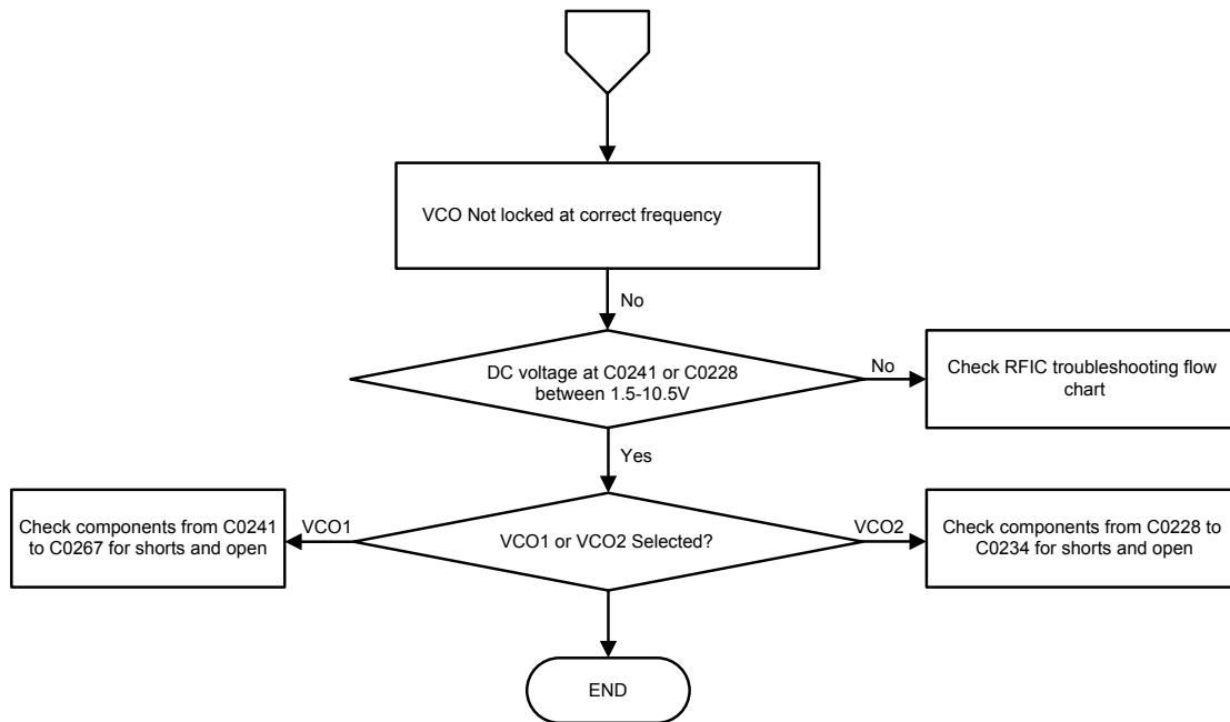
Figure 81: Troubleshooting Flow Chart for Rx VCO (Sheet 3 of 3)
