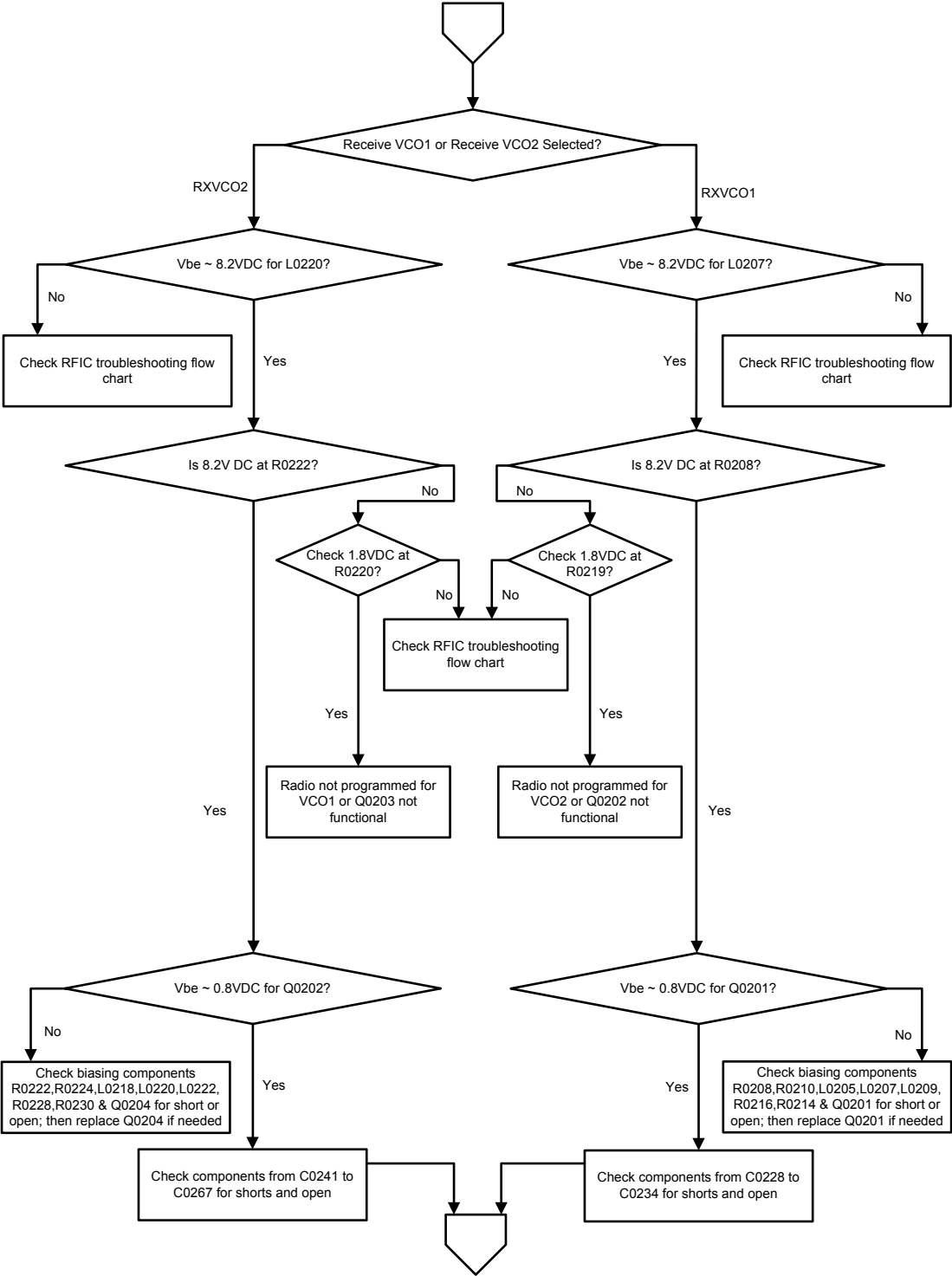
Figure 74: Troubleshooting Flow Chart for Rx VCO (Sheet 2 of 3)
