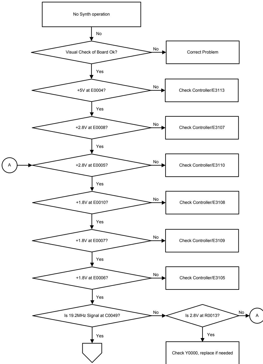
Figure 61: Troubleshooting Flow Chart for RFIC (Sheet 1 of 5)
