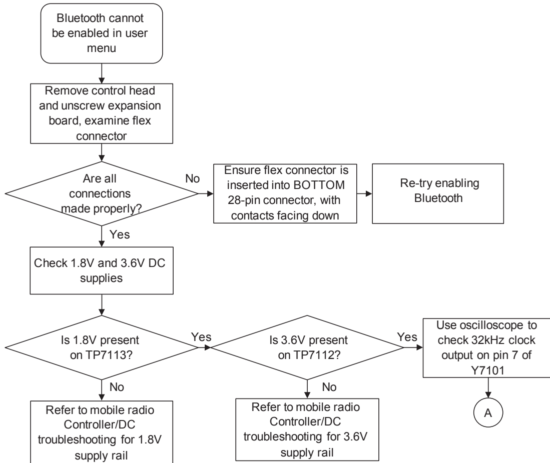
Figure 91: Troubleshooting Flow Chart for Bluetooth (Sheet 1 of 4)
