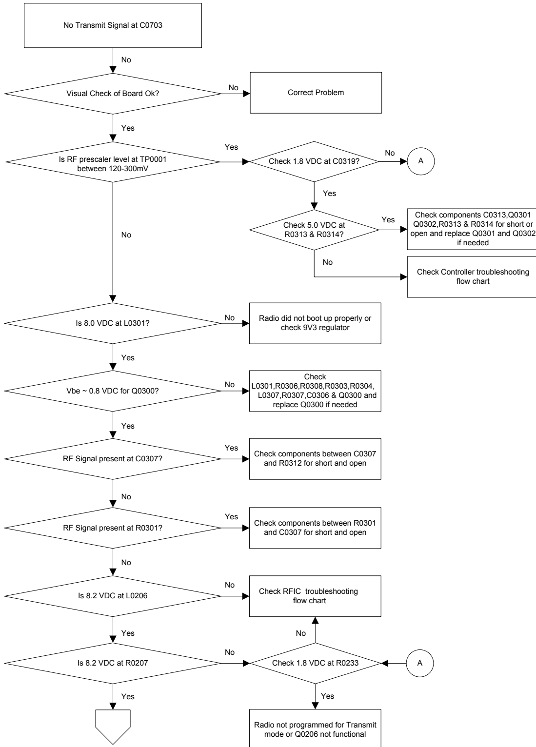
Figure 82: Troubleshooting Flow Chart for Tx VCO (Sheet 1 of 2)
