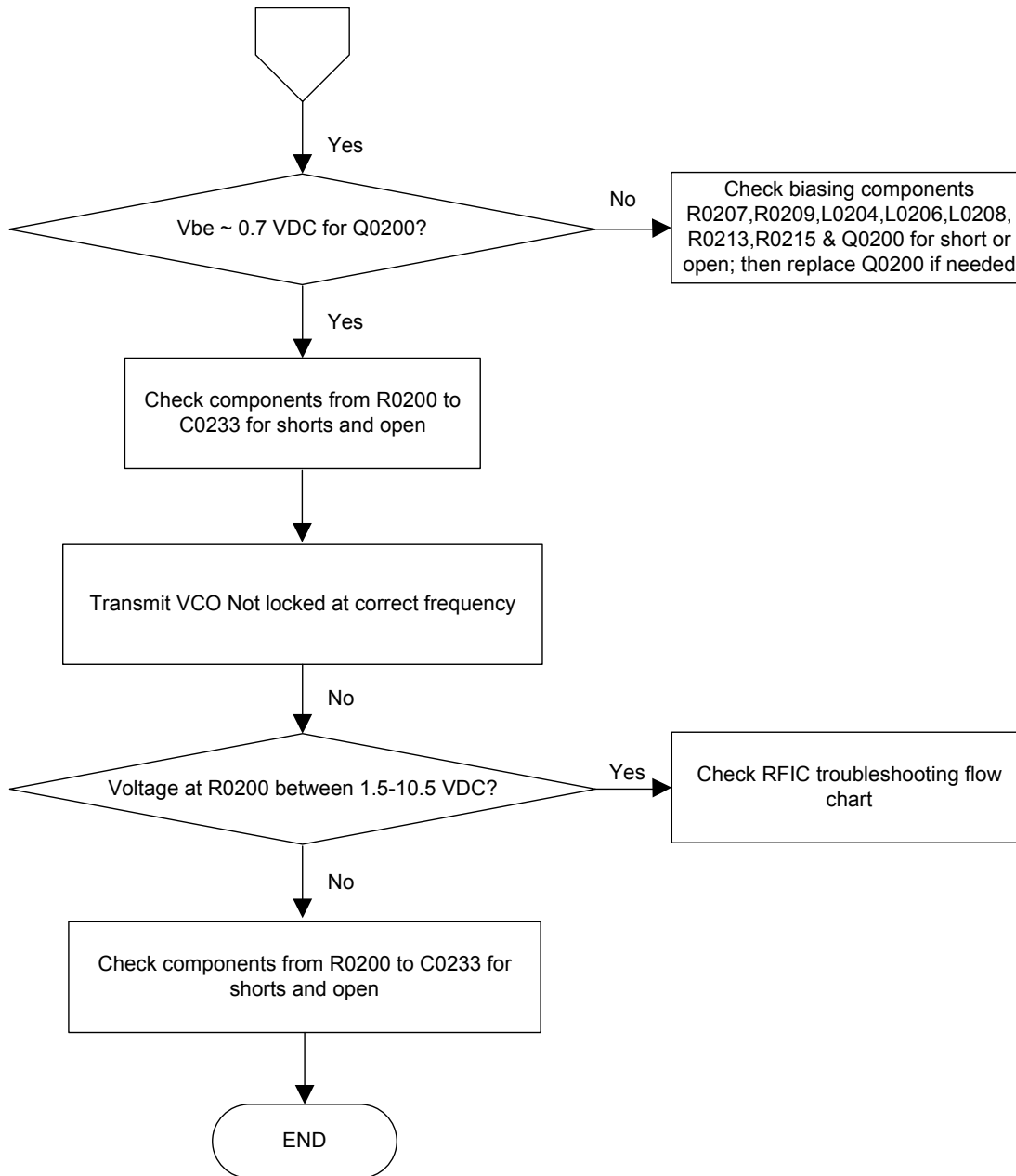
Figure 83: Troubleshooting Flow Chart for Tx VCO (Sheet 2 of 2)
