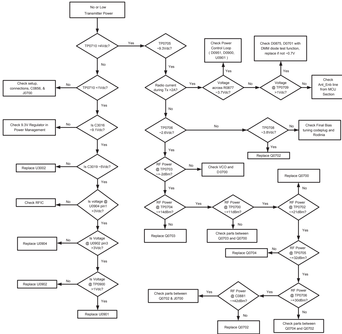
Figure 50: Troubleshooting Flow Chart for Transmitter
