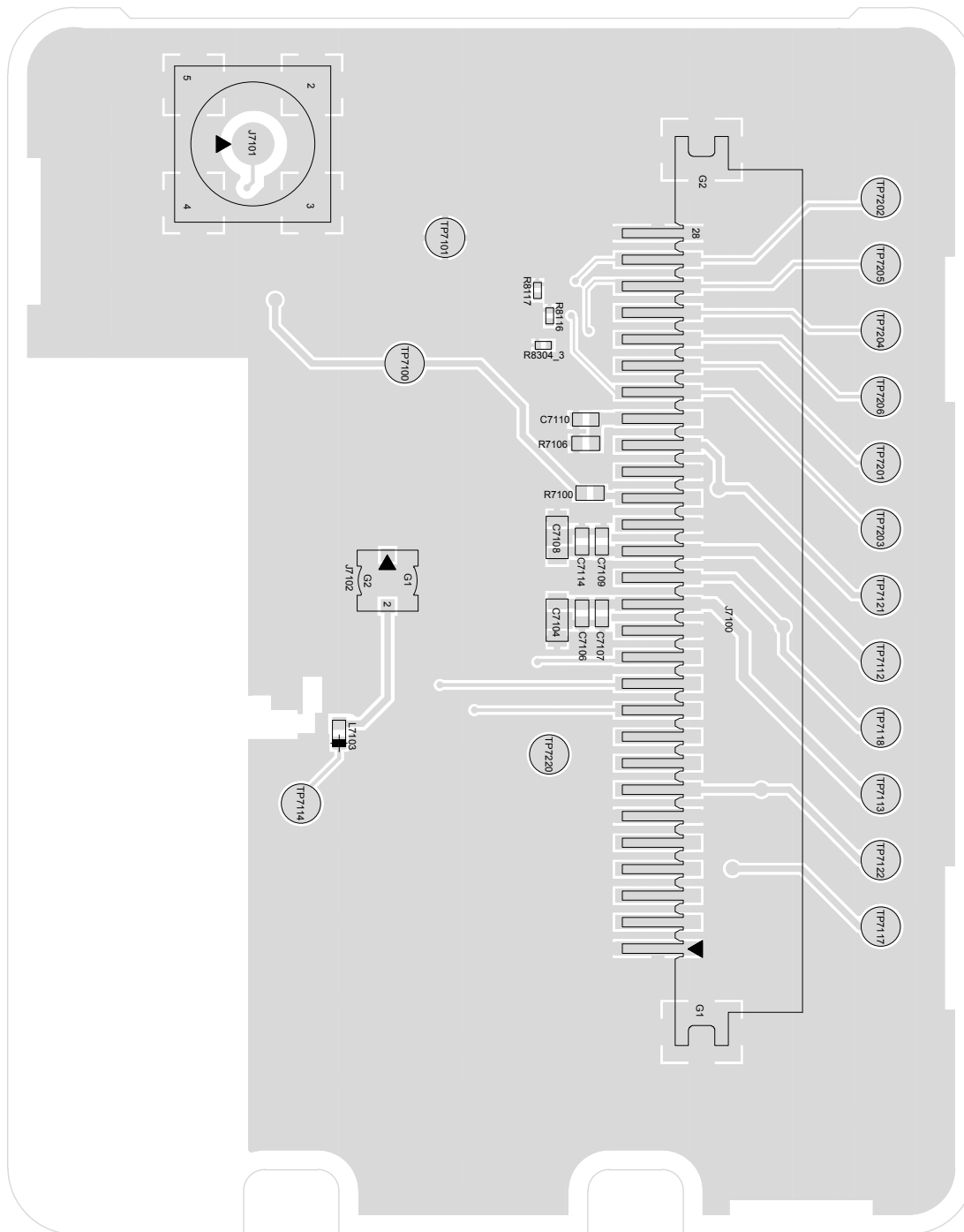
Figure 264: Expansion Board Bottom Side PCB No. PC000942A01-AA
