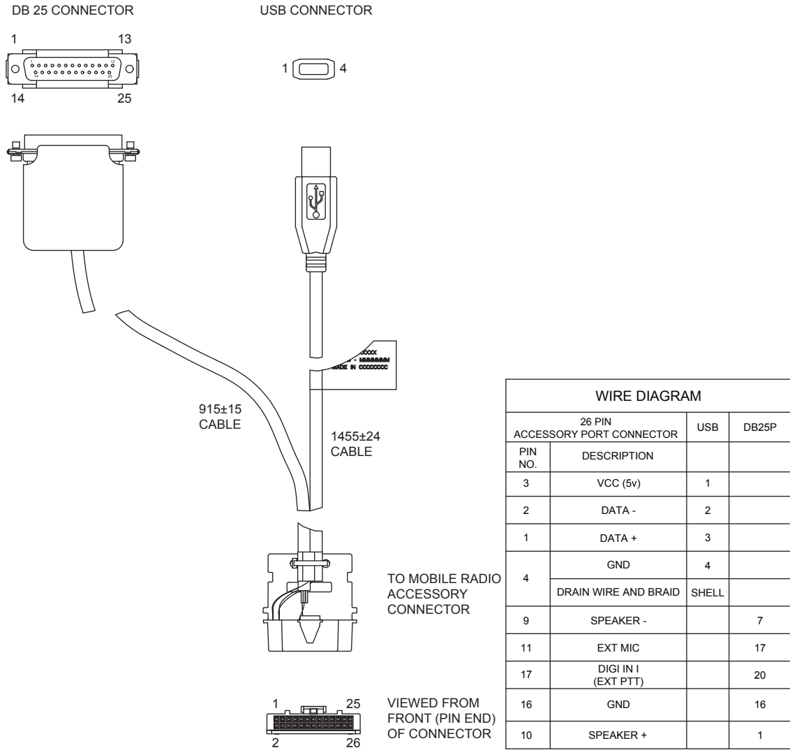
Figure 3: Mobile & Repeater Rear Accessory Programming and Test Cable PMKN4016_
