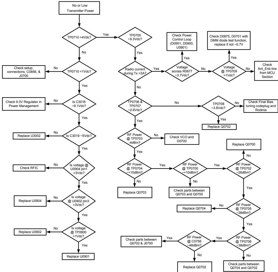
Figure 45: Troubleshooting Flow Chart for Transmitter
