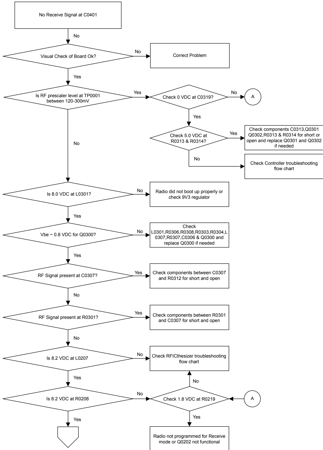
Figure 71: Troubleshooting Flow Chart for Rx VCO (Sheet 1 of 2)
