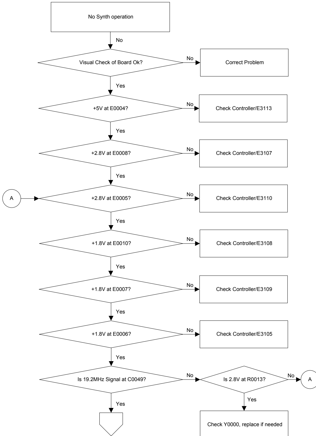
Figure 51: Troubleshooting Flow Chart for RFIC (Sheet 1 of 5)
