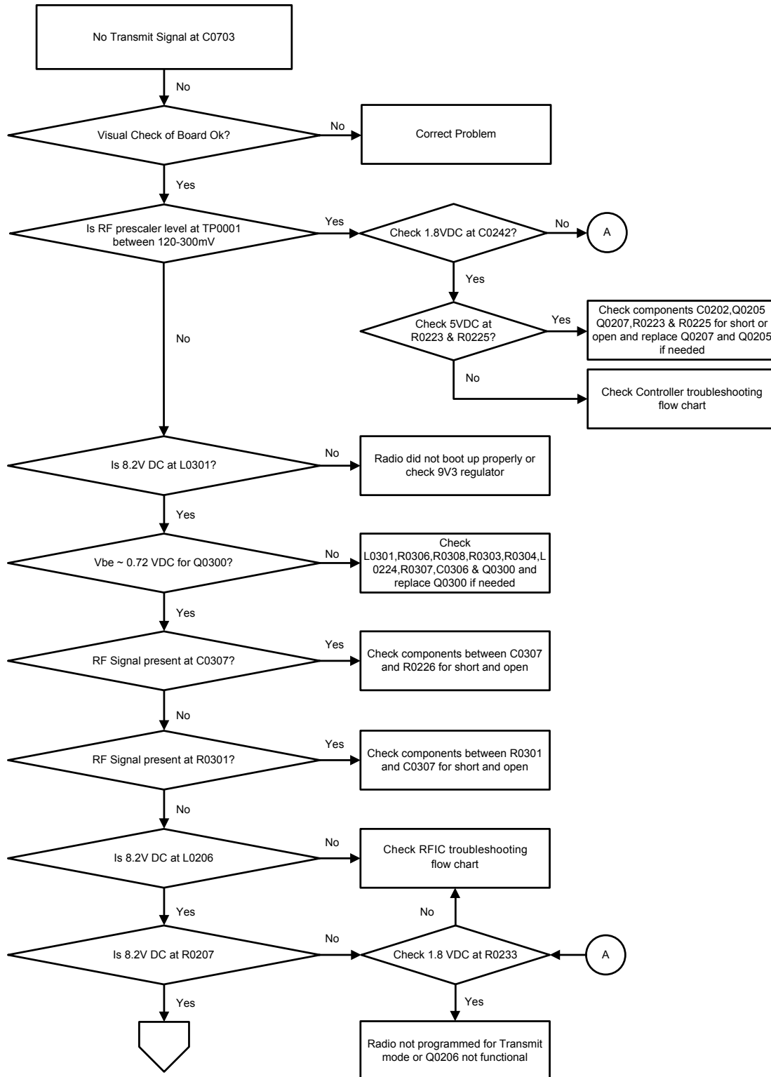
Figure 84: Troubleshooting Flow Chart for Tx VCO (Sheet 1 of 2)
