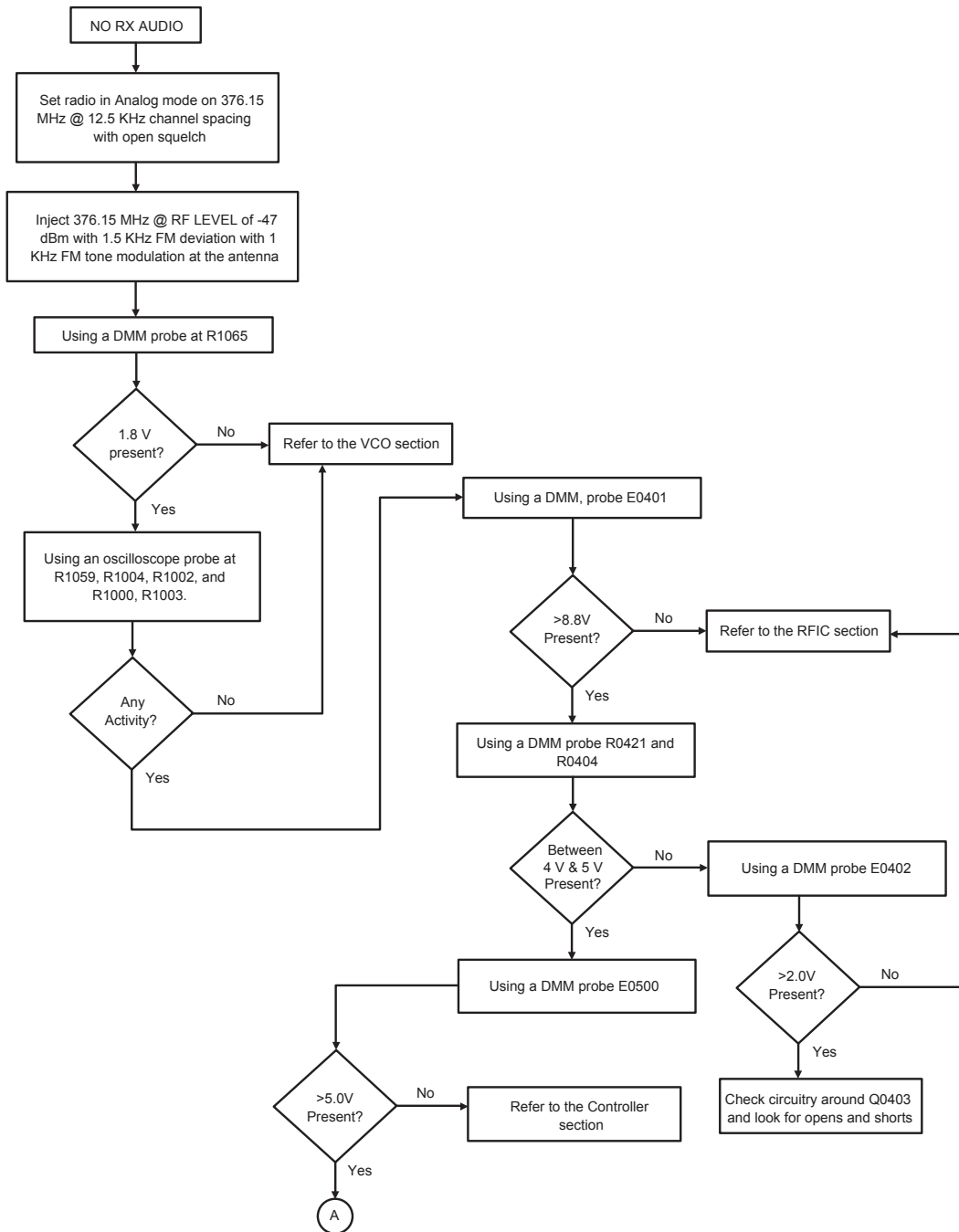
Figure 35: Troubleshooting Flow Chart for Receiver for 84012728001-A (Sheet 1 of 3)
