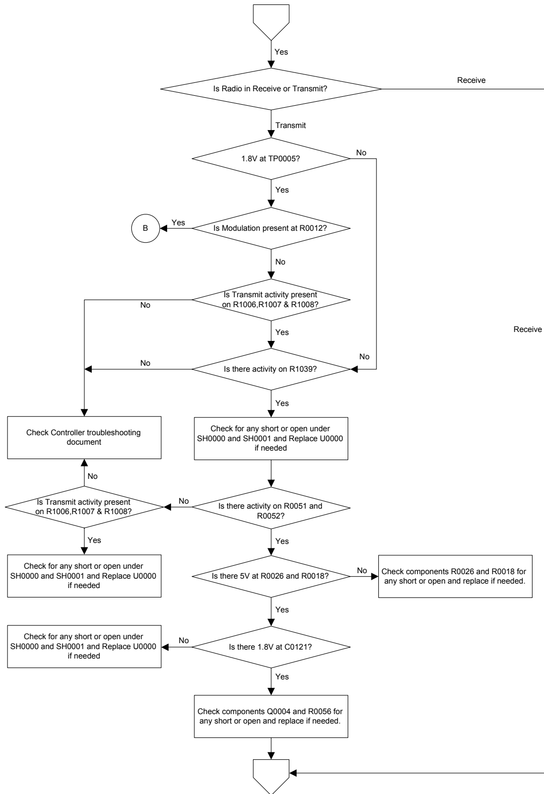
Figure 53: Troubleshooting Flow Chart for RFIC (Sheet 3 of 5)
