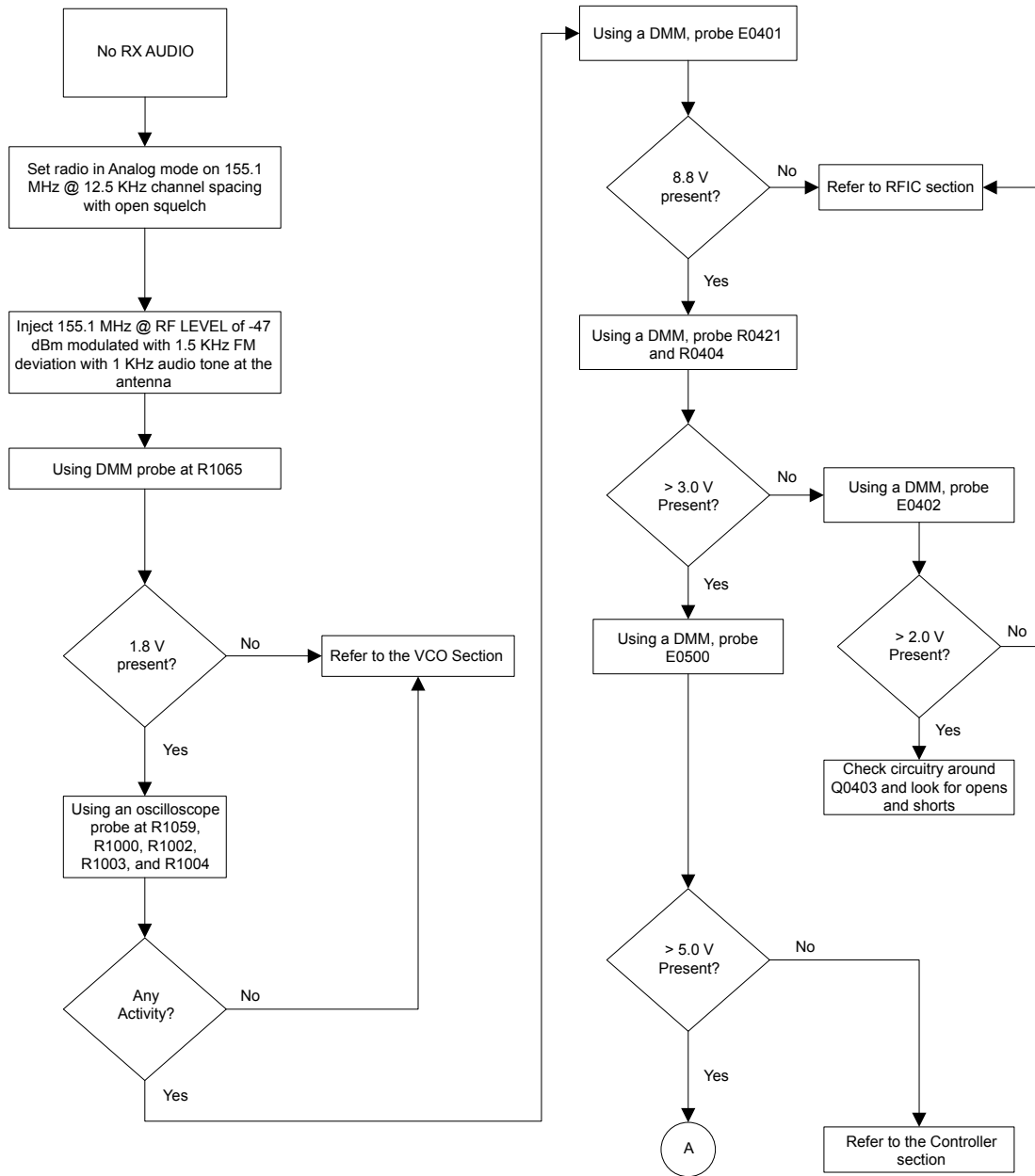
Figure 20: Troubleshooting Flow Chart for Receiver for 84012734002-B (Sheet 1 of 3)
