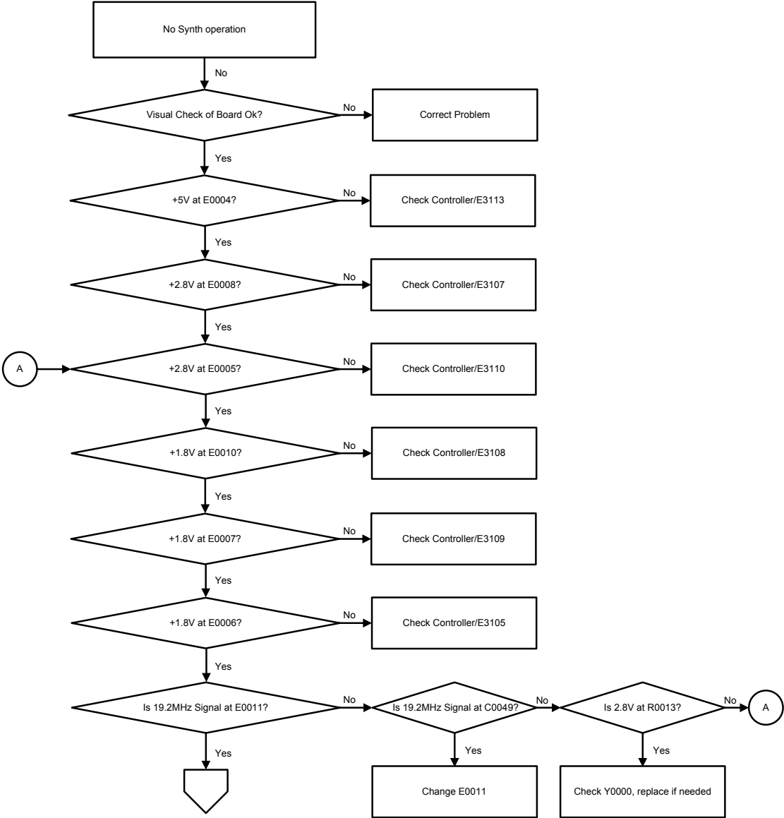
Figure 66: Troubleshooting Flow Chart for RFIC (Sheet 1 of 5)
