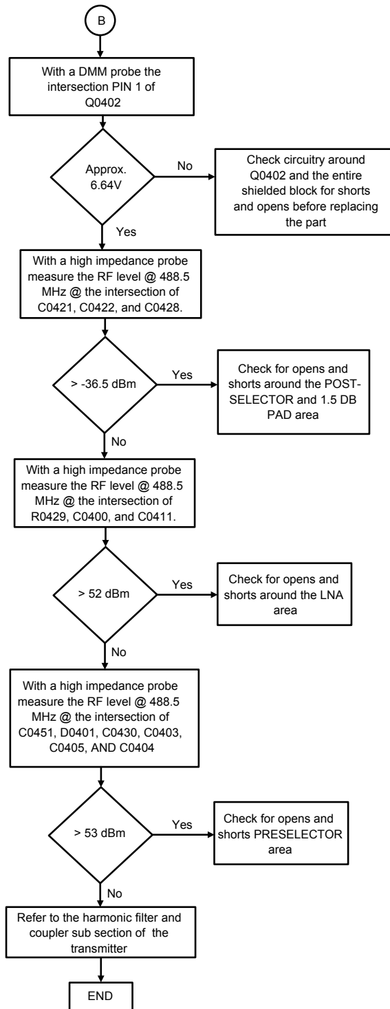
Figure 37: Troubleshooting Flow Chart for Receiver for 84012728001-A (Sheet 3 of 3)
