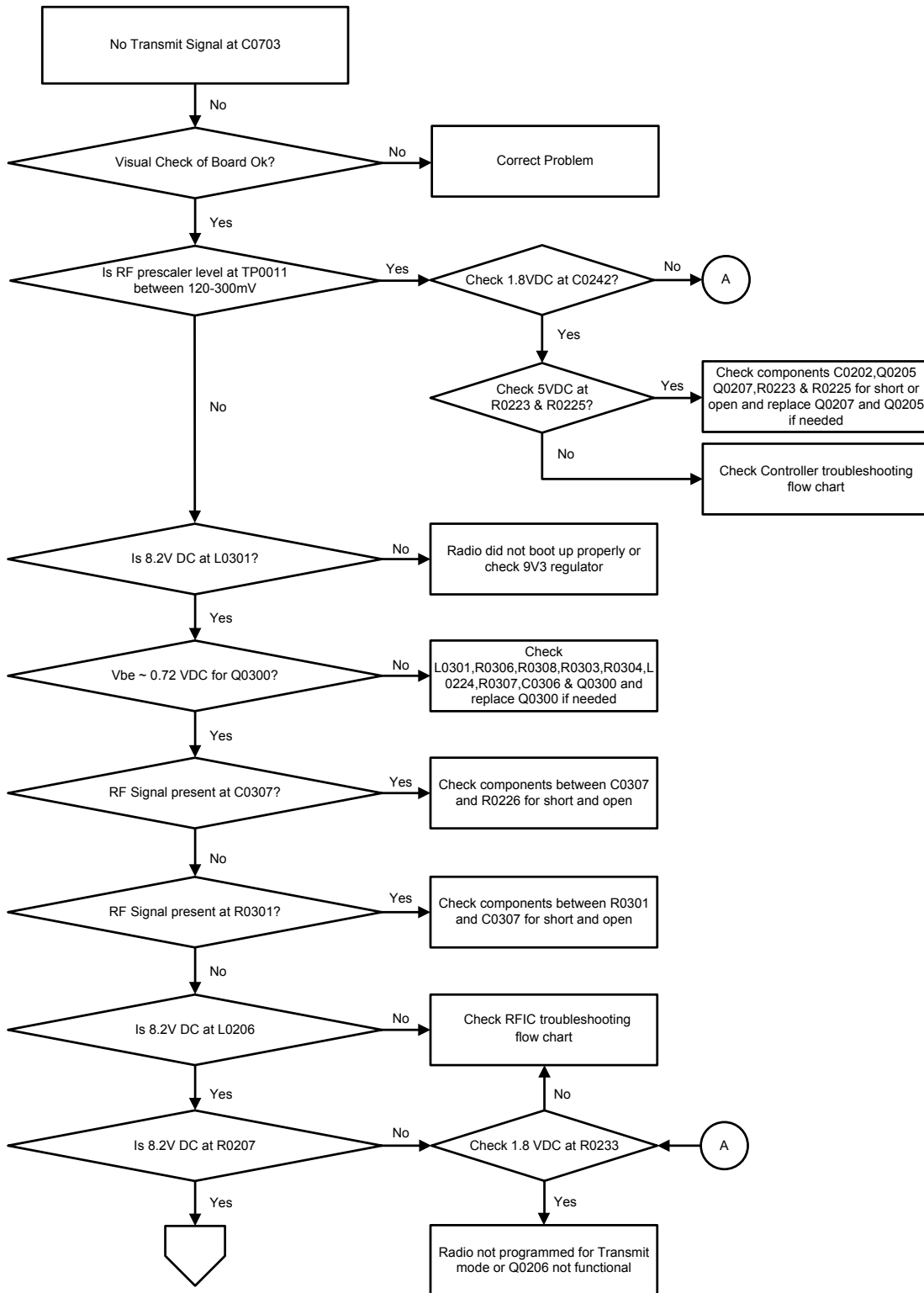
Figure 86: Troubleshooting Flow Chart for Tx VCO (Sheet 1 of 2)
