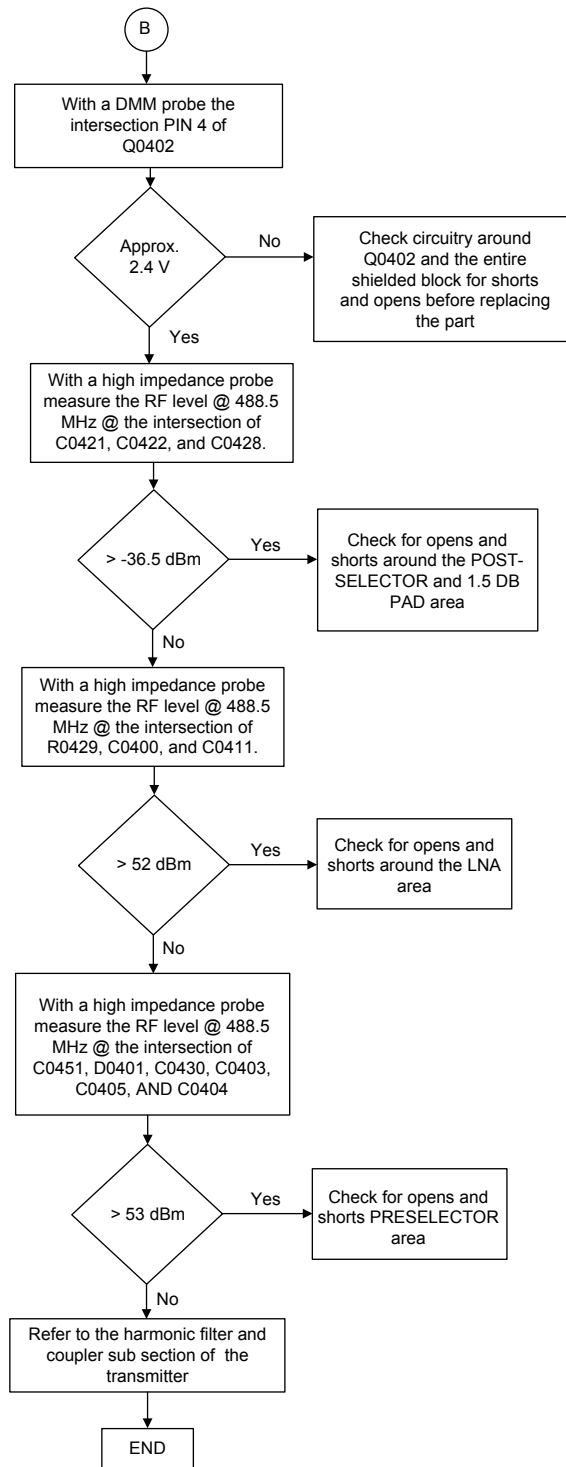
Figure 40: Troubleshooting Flow Chart for Receiver for 84012728003-C (Sheet 3 of 3)
