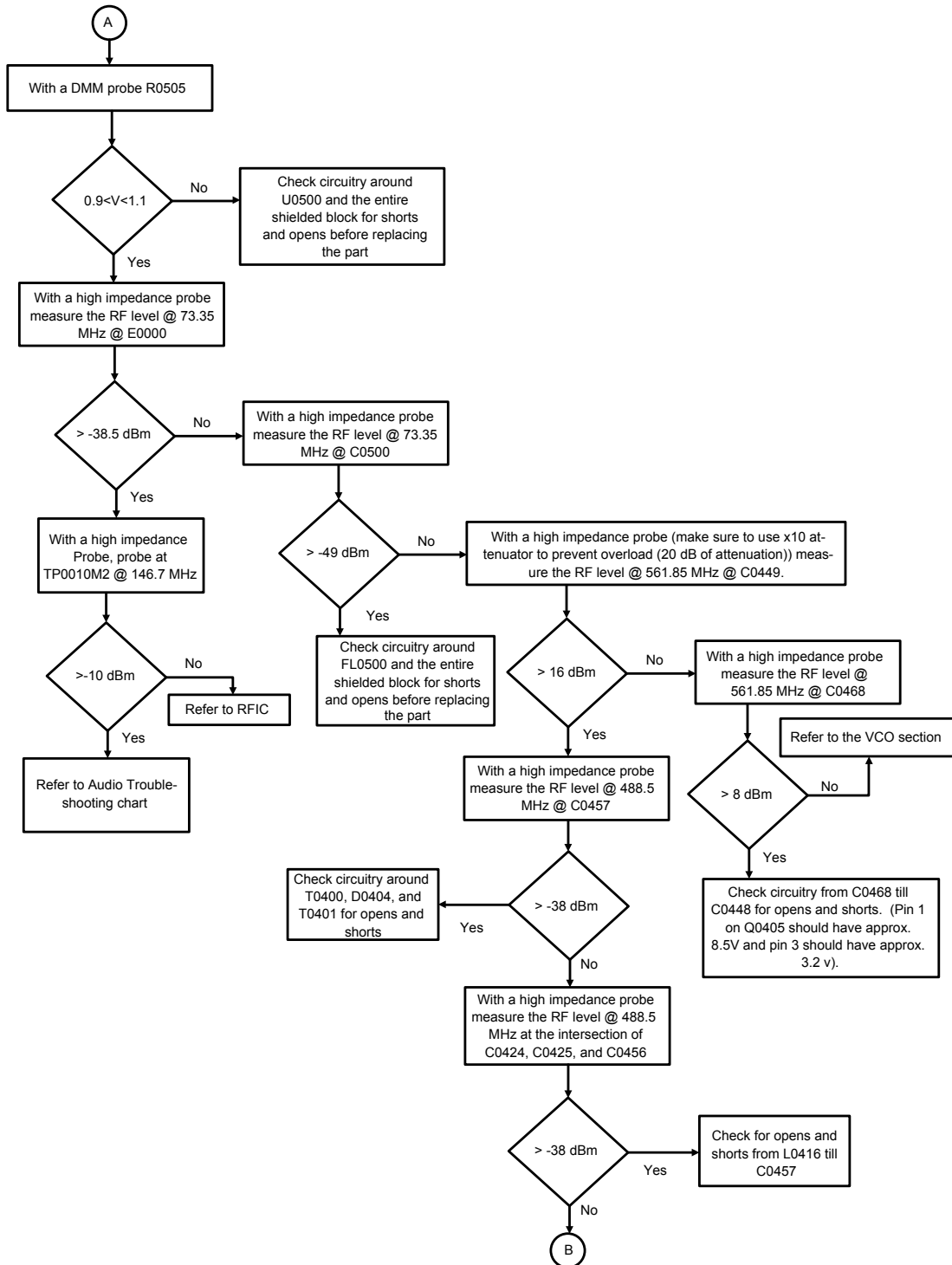
Figure 36: Troubleshooting Flow Chart for Receiver for 84012728001-A (Sheet 2 of 3)
