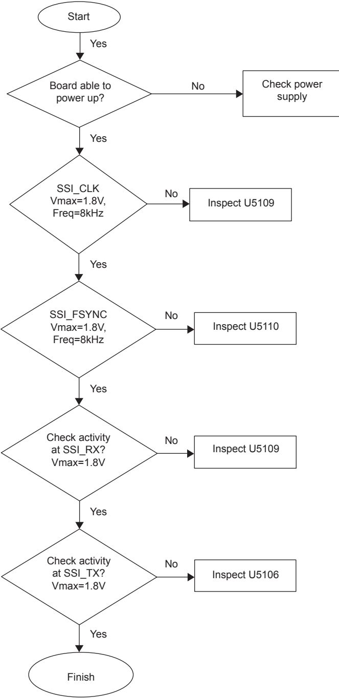
Figure 100: Troubleshooting Flow Chart for GOB (PMLN7324_S)
