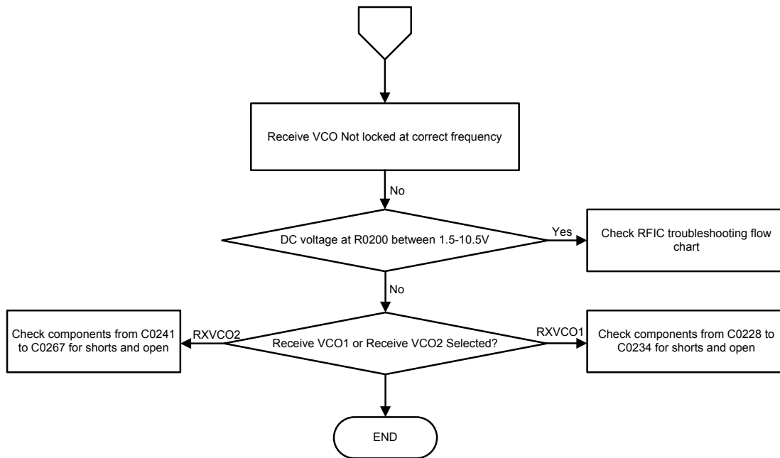
Figure 75: Troubleshooting Flow Chart for Rx VCO (Sheet 3 of 3)
