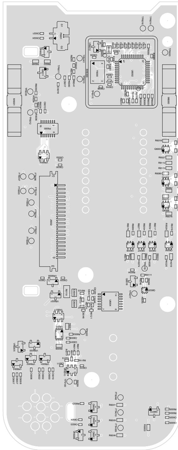
Figure 102: Numeric Display Control Head Bottom Side PCB No. 84012212002-B
