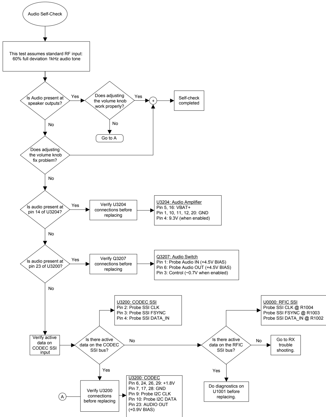
Figure 16: Troubleshooting Chart for Audio
