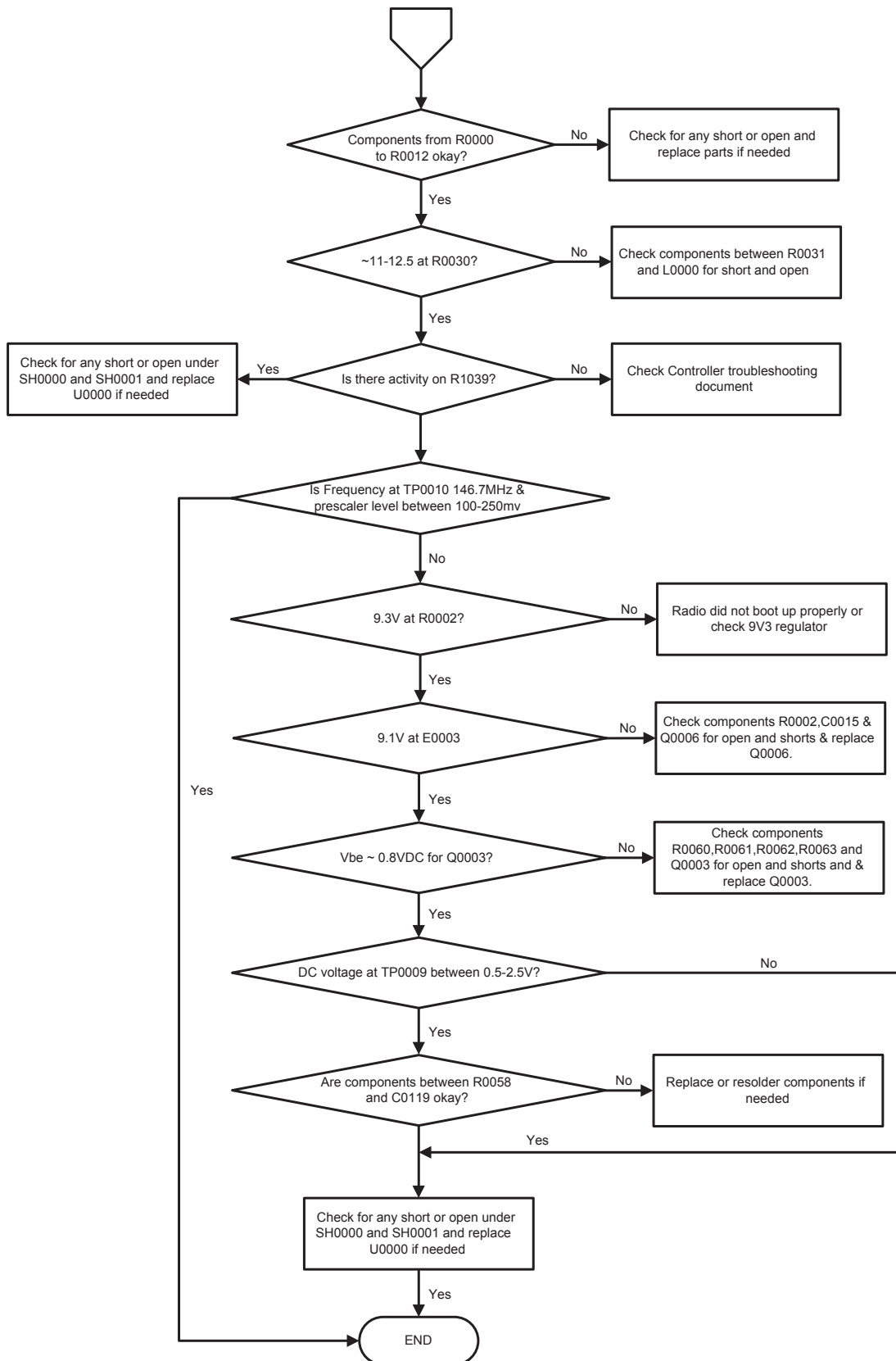
Figure 65: Troubleshooting Flow Chart for RFIC (Sheet 5 of 5)
