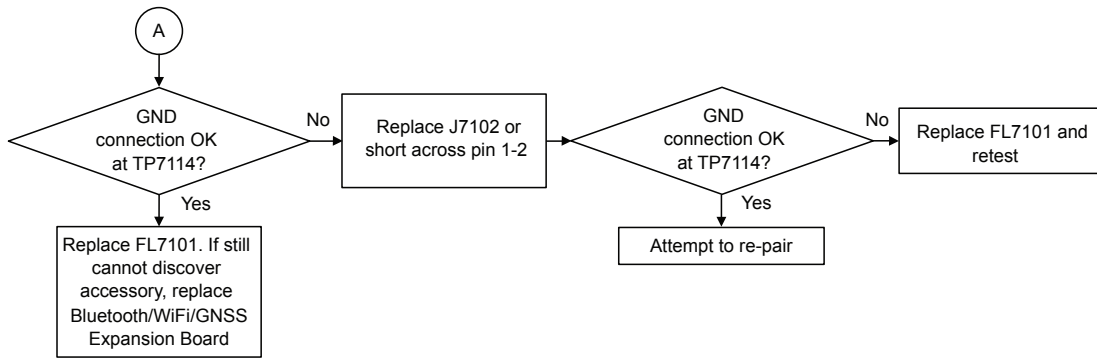
Figure 94: Troubleshooting Flow Chart for Bluetooth (Sheet 4 of 4)
