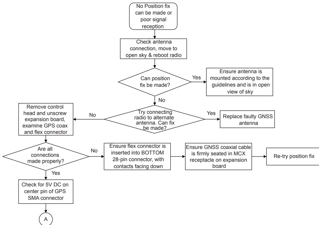
Figure 95: Troubleshooting Flow Chart for GNSS (Sheet 1 of 3)
