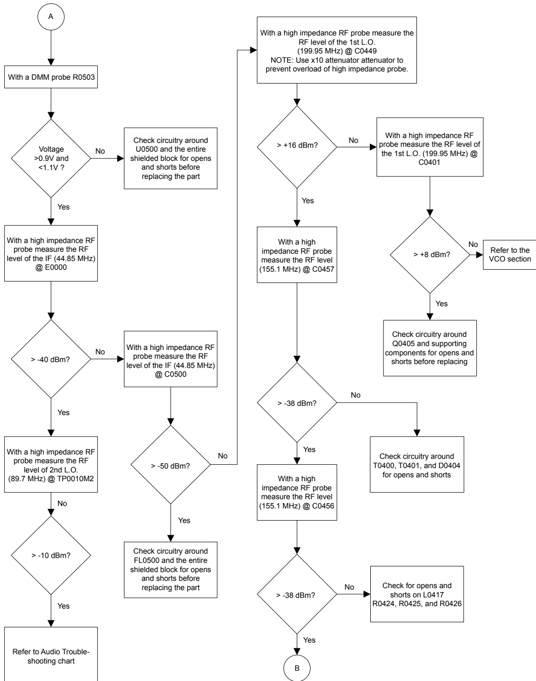
Figure 18: Troubleshooting Flow Chart for Receiver for 84012734001-A (Sheet 2 of 3)
