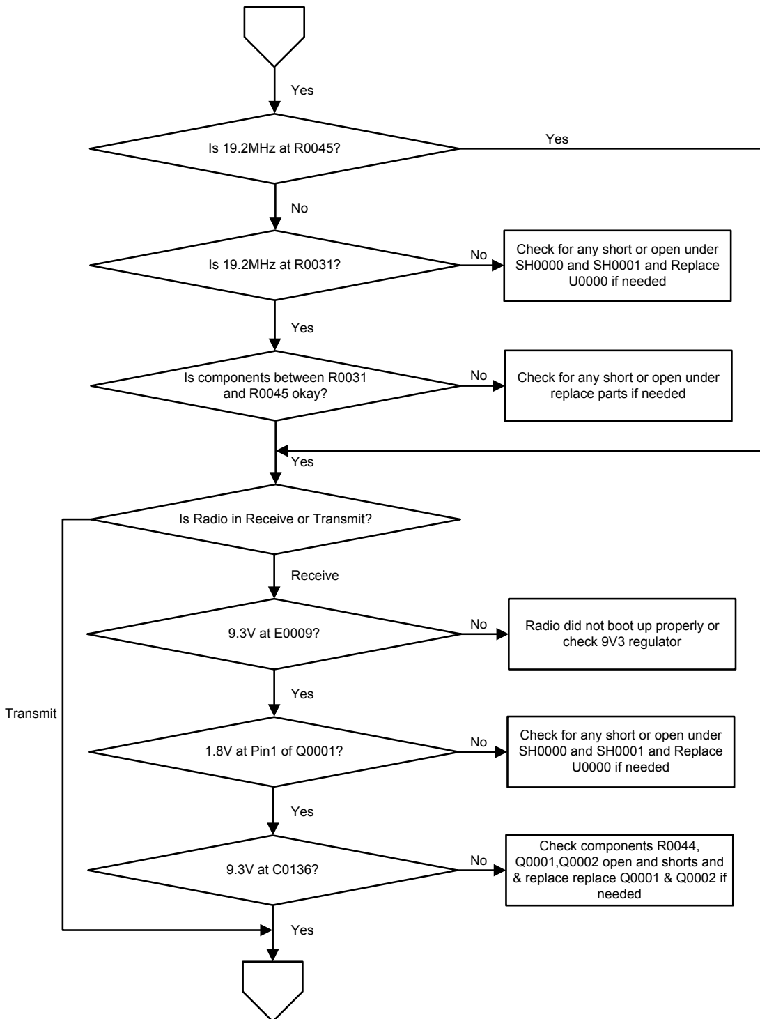
Figure 67: Troubleshooting Flow Chart for RFIC (Sheet 2 of 5)
