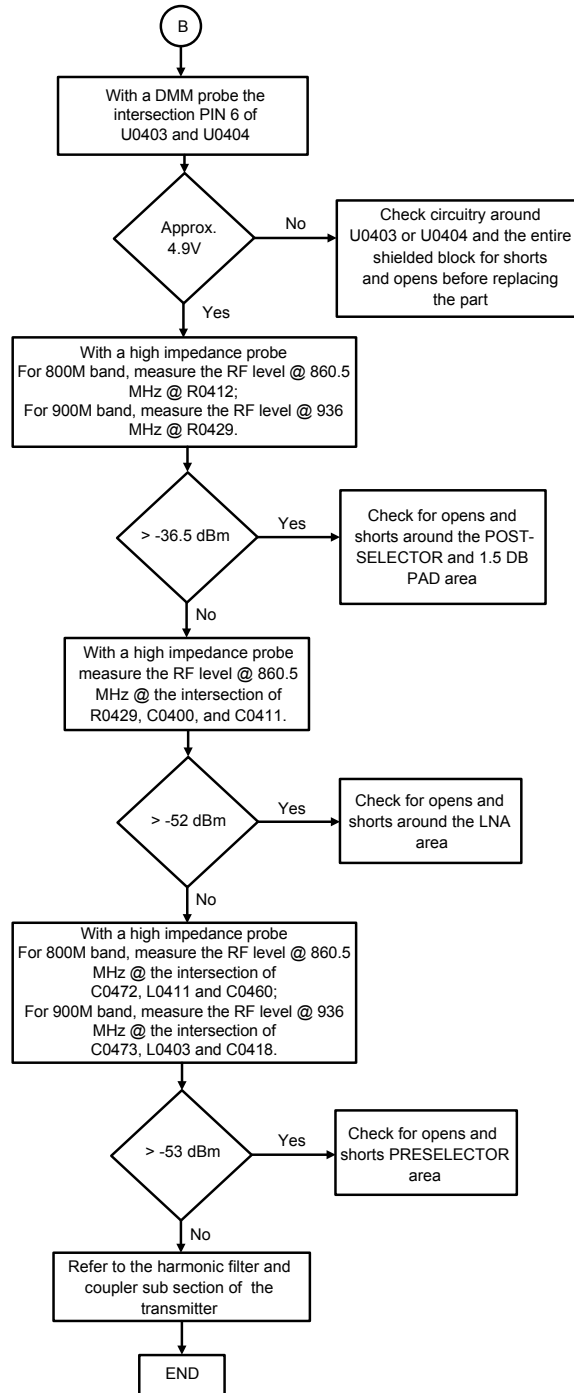
Figure 43: Troubleshooting Flow Chart for Receiver (Sheet 3 of 3)
