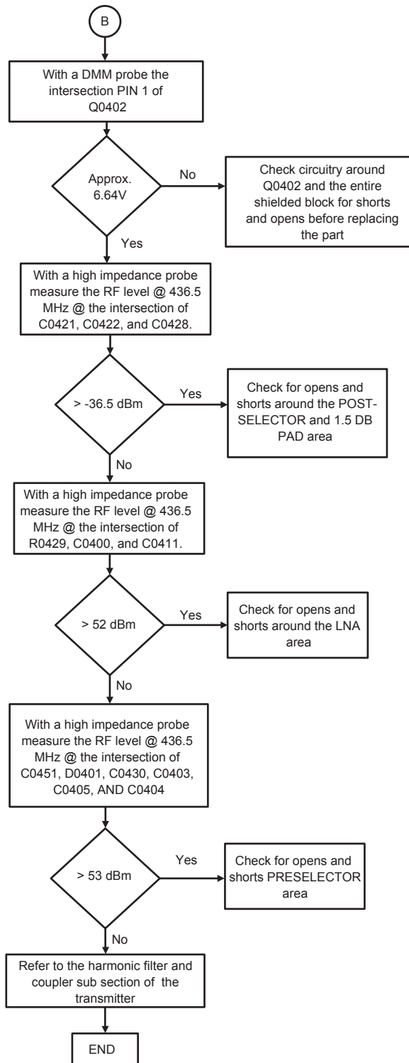
Figure 25: Troubleshooting Flow Chart for Receiver for 84012735001-A (Sheet 3 of 3)
