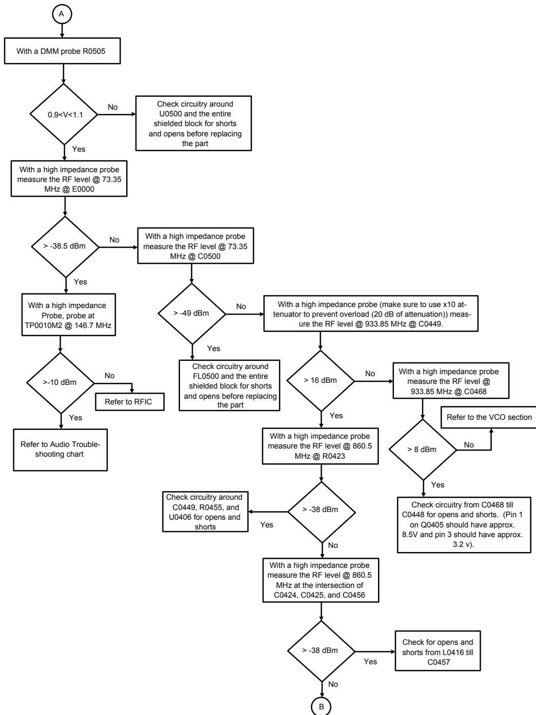
Figure 42: Troubleshooting Flow Chart for Receiver (Sheet 2 of 3)
