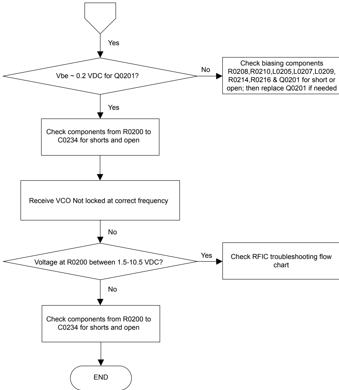
Figure 72: Troubleshooting Flow Chart for Rx VCO (Sheet 2 of 2)
