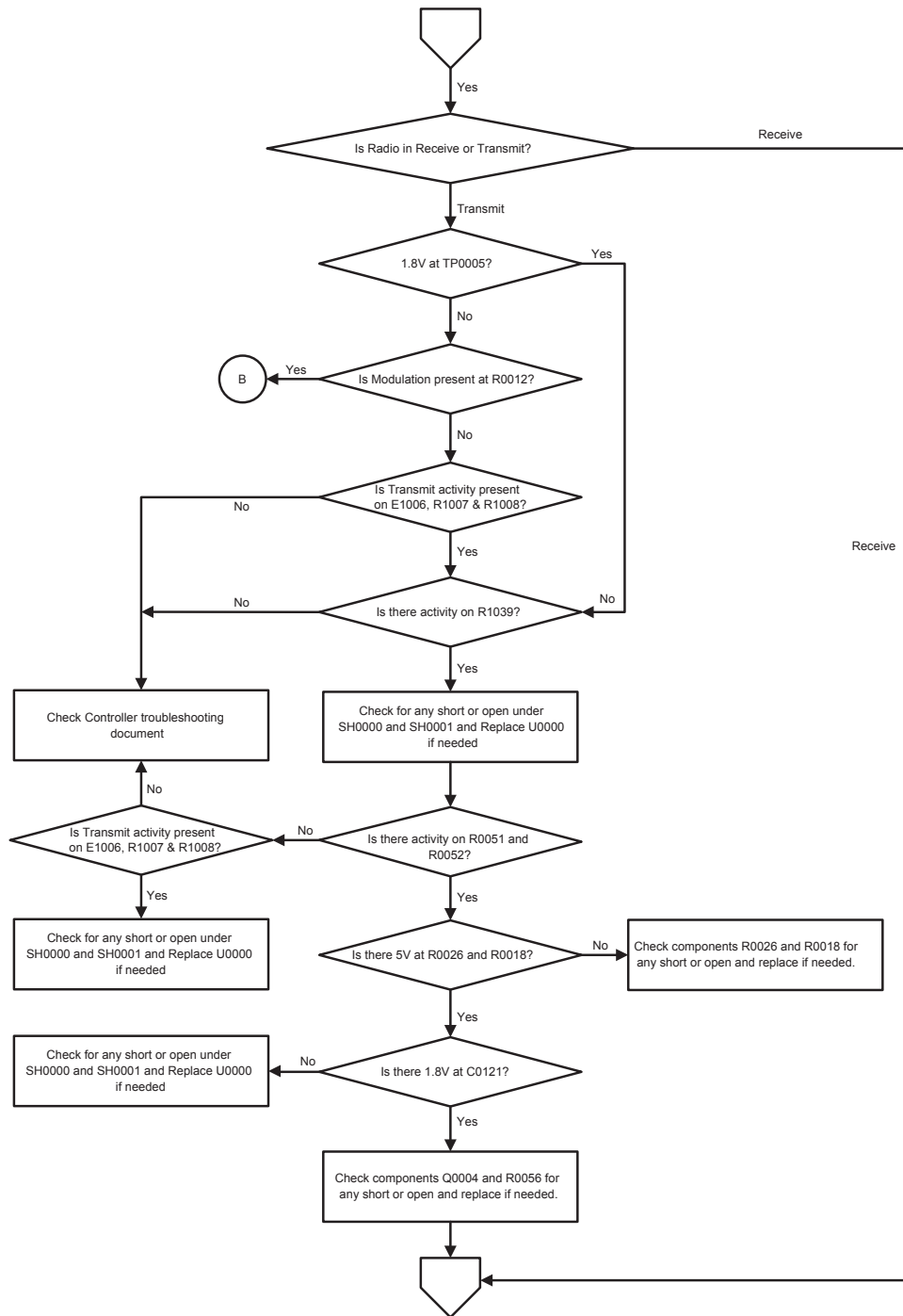
Figure 68: Troubleshooting Flow Chart for RFIC (Sheet 3 of 5)
