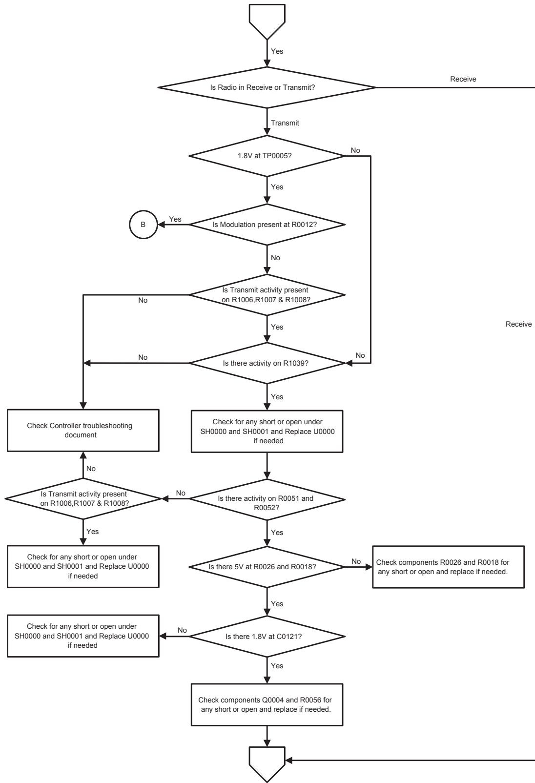
Figure 63: Troubleshooting Flow Chart for RFIC (Sheet 3 of 5)
