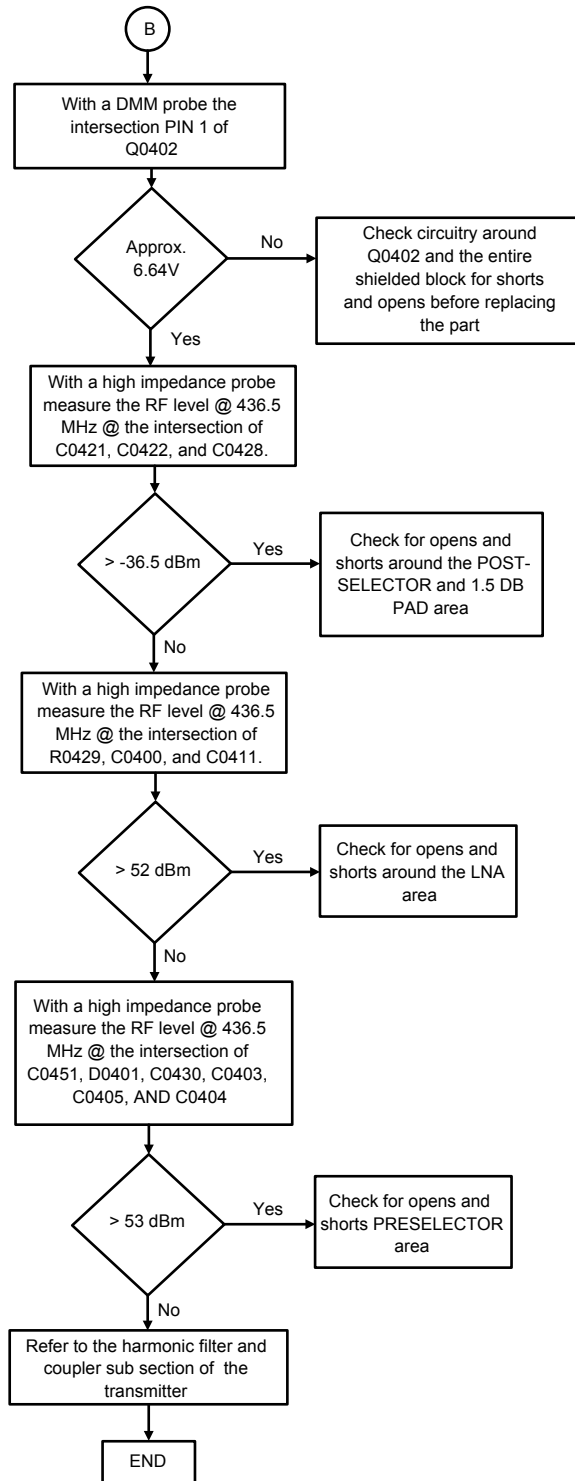
Figure 31: Troubleshooting Flow Chart for Receiver for 84012737001-A (Sheet 3 of 3)
