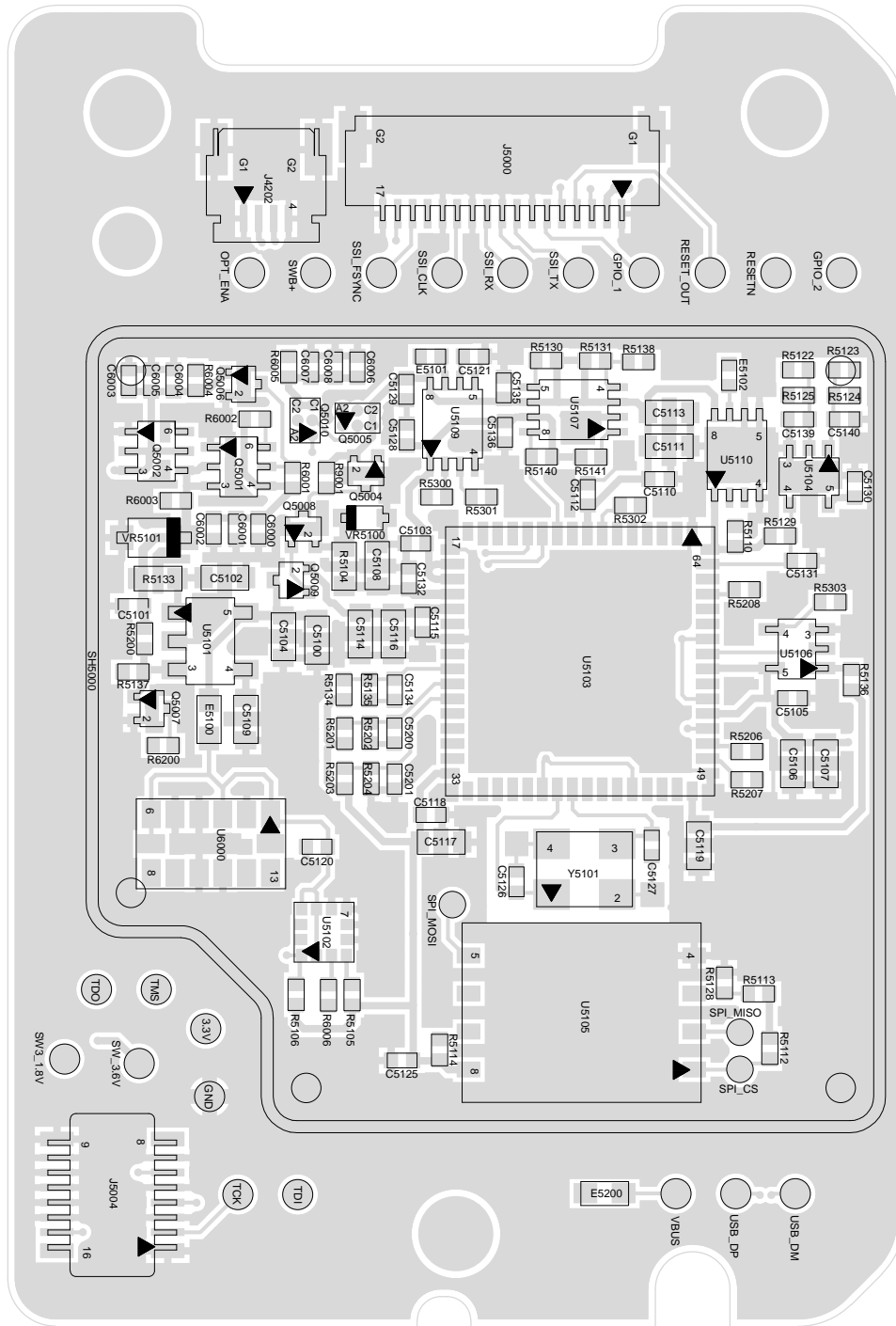
Figure 270: GOB Bottom Side PCB No. PC000957A01-CA
