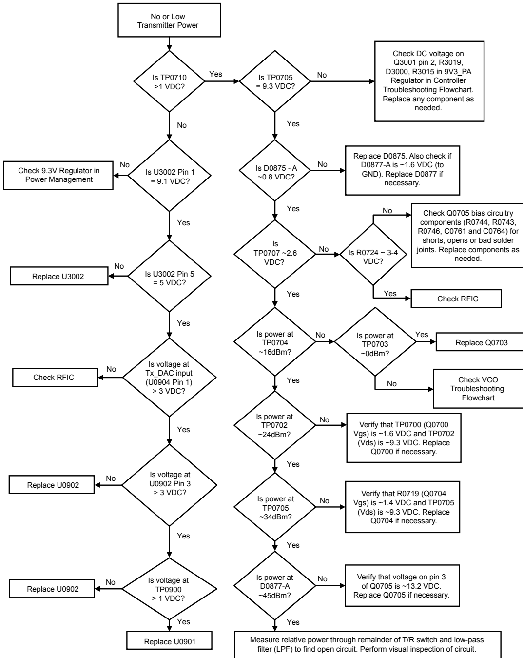
Figure 46: Troubleshooting Flow Chart for Transmitter
