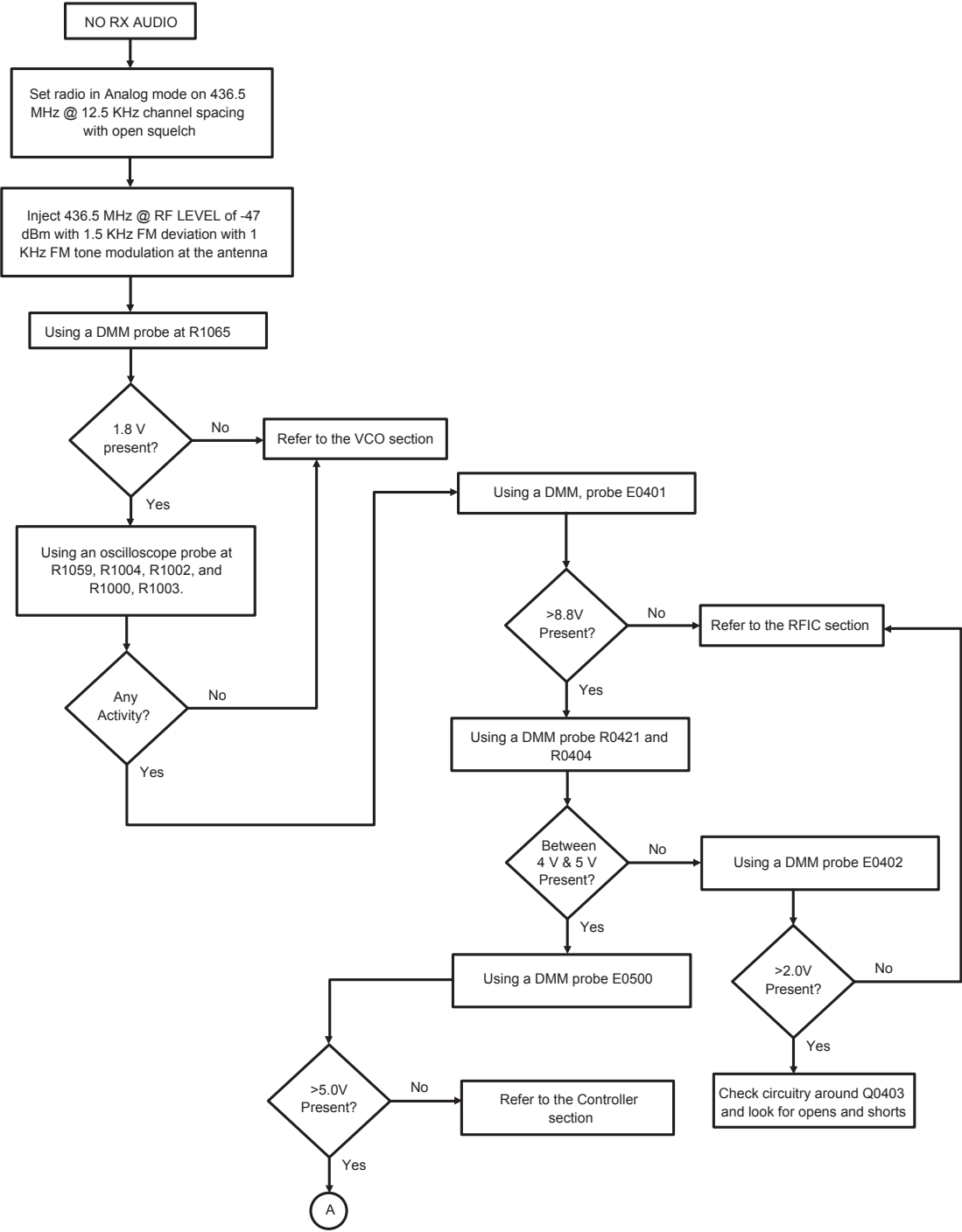
Figure 26: Troubleshooting Flow Chart for Receiver for 84012735003-C (Sheet 1 of 3)
