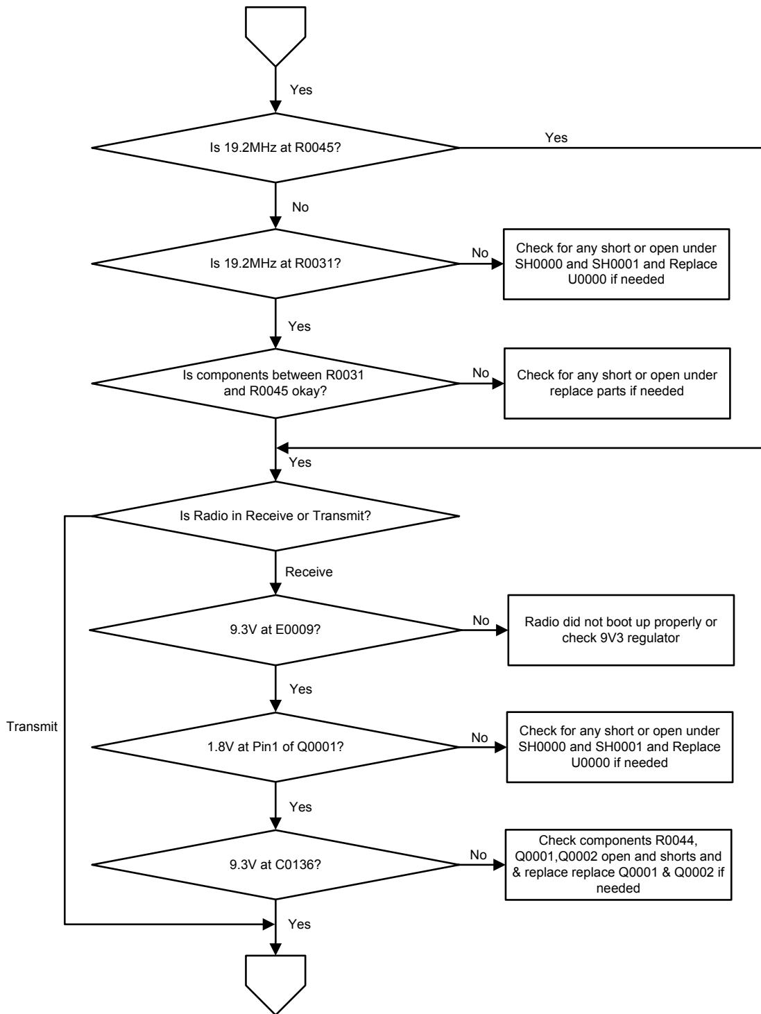
Figure 57: Troubleshooting Flow Chart for RFIC (Sheet 2 of 5)
