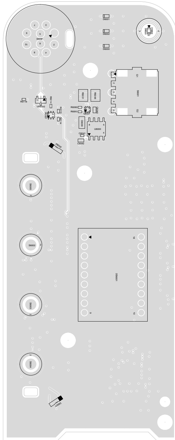
Figure 101: Numeric Display Control Head Top Side PCB No. 84012212002-B
