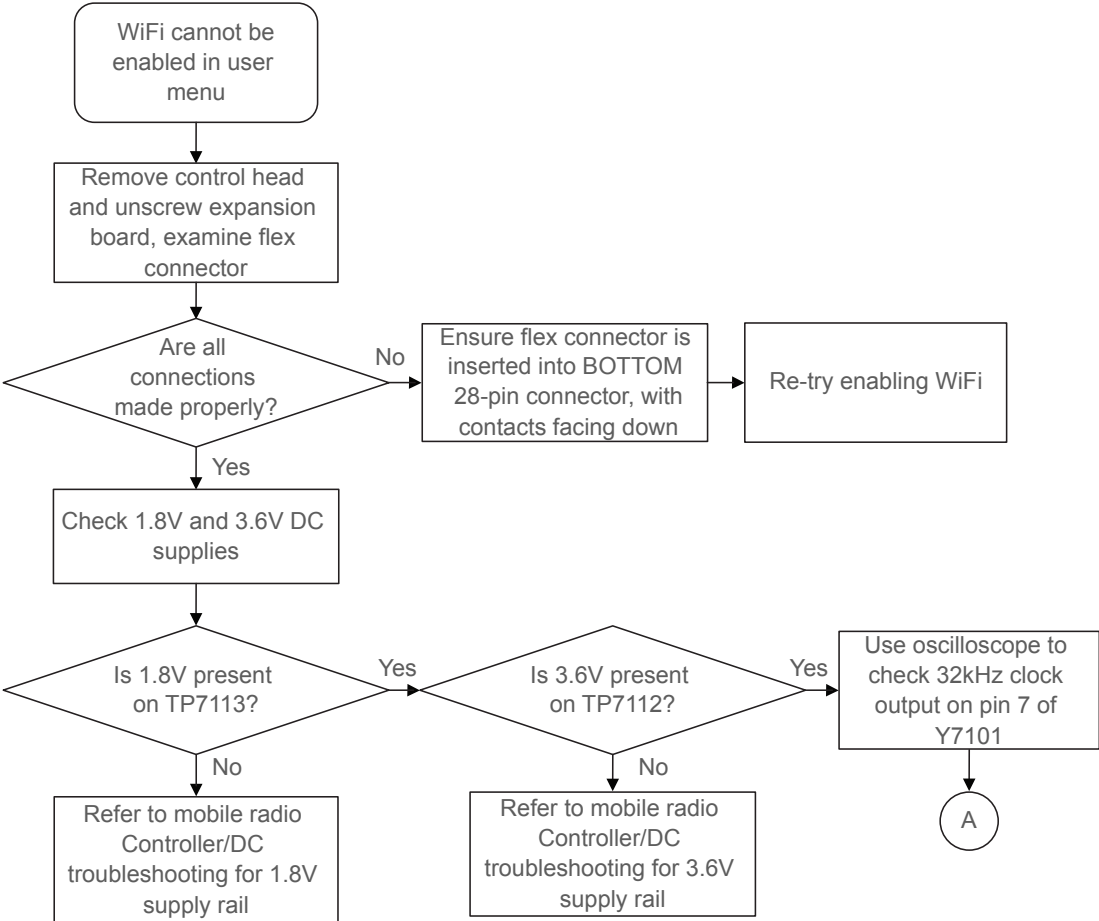
Figure 98: Troubleshooting Flow Chart for Wi-Fi (Sheet 1 of 2)
