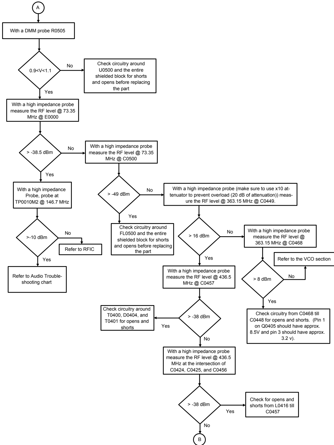
Figure 30: Troubleshooting Flow Chart for Receiver for 84012737001-A (Sheet 2 of 3)
