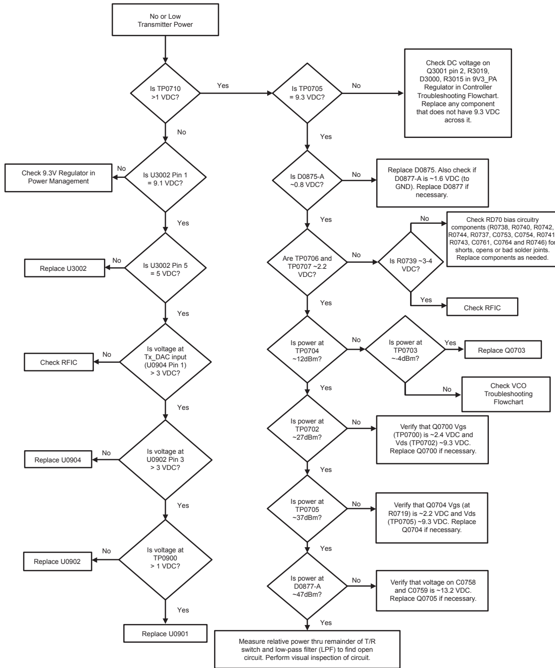
Figure 47: Troubleshooting Flow Chart for Transmitter
