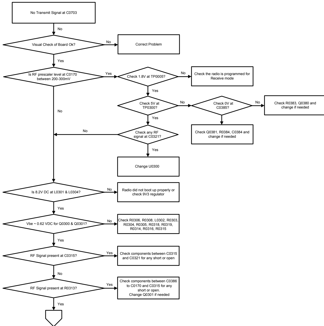
Figure 88: Troubleshooting Flow Chart for Tx VCO (Sheet 1 of 3)
