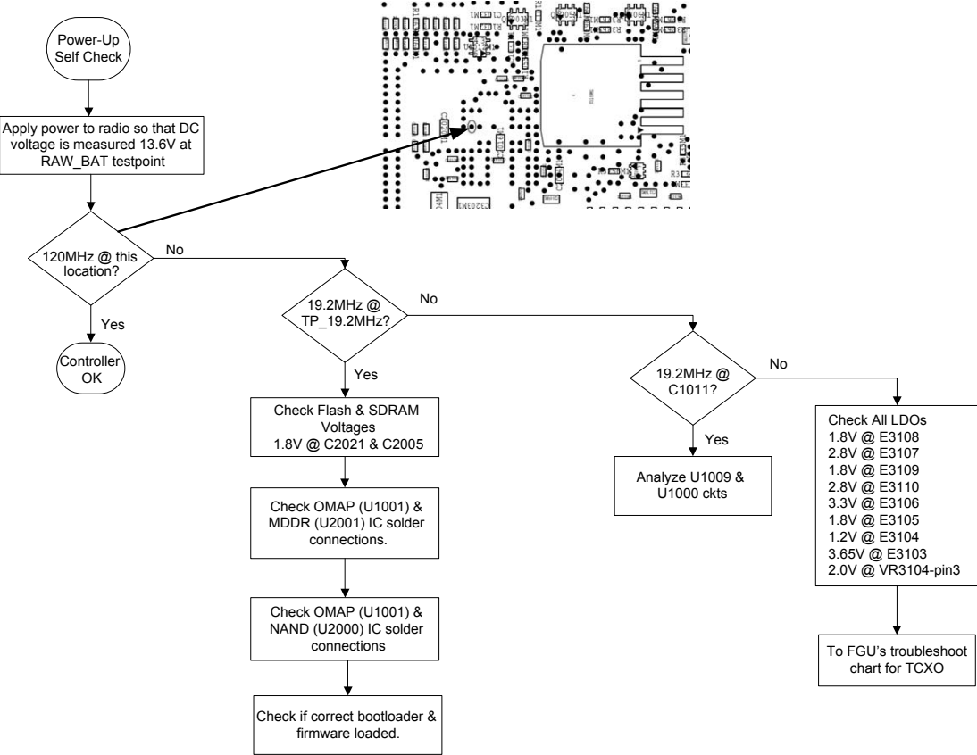
Figure 12: Troubleshooting Chart for Power-Up
