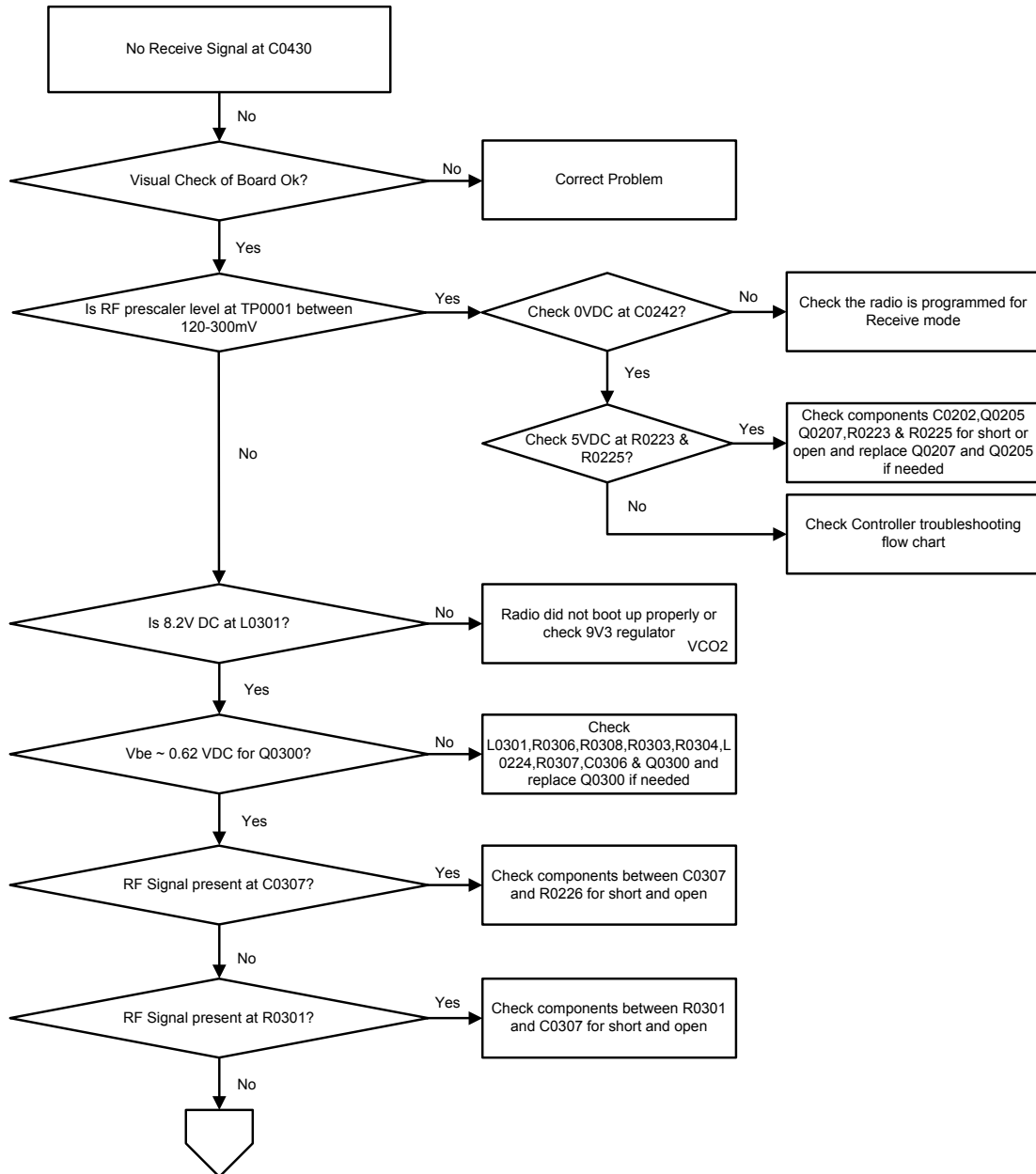
Figure 73: Troubleshooting Flow Chart for Rx VCO (Sheet 1 of 3)
