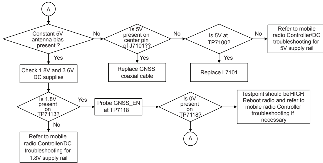
Figure 97: Troubleshooting Flow Chart for GNSS (Sheet 3 of 3)
