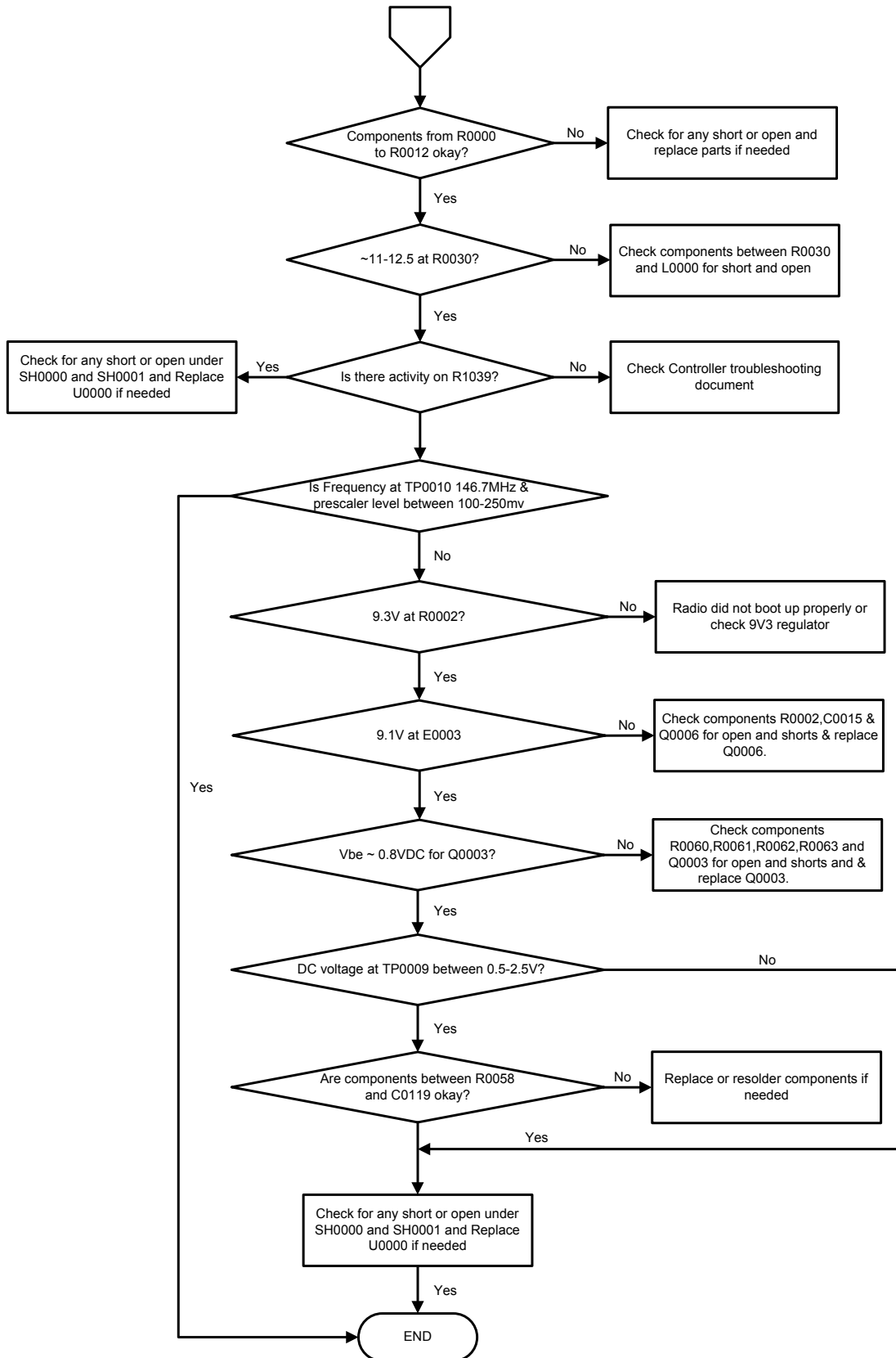
Figure 60: Troubleshooting Flow Chart for RFIC (Sheet 5 of 5)
