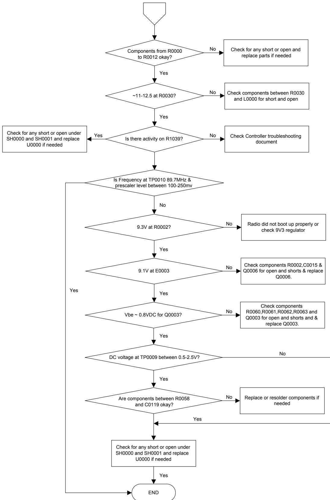
Figure 55: Troubleshooting Flow Chart for RFIC (Sheet 5 of 5)
