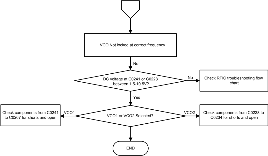
Figure 90: Troubleshooting Flow Chart for Tx VCO (Sheet 3 of 3)
