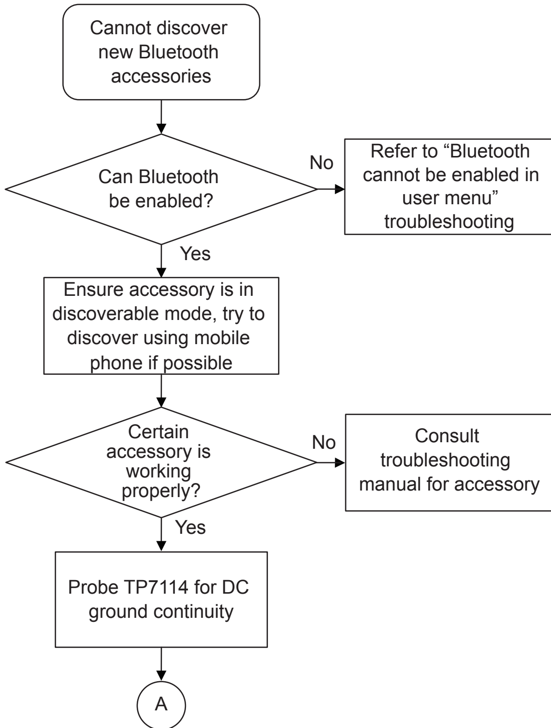
Figure 93: Troubleshooting Flow Chart for Bluetooth (Sheet 3 of 4)
