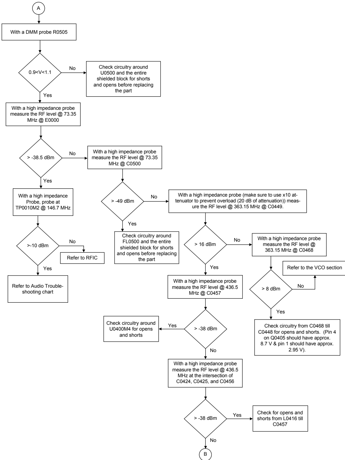
Figure 33: Troubleshooting Flow Chart for Receiver for 84012737003-C (Sheet 2 of 3)
