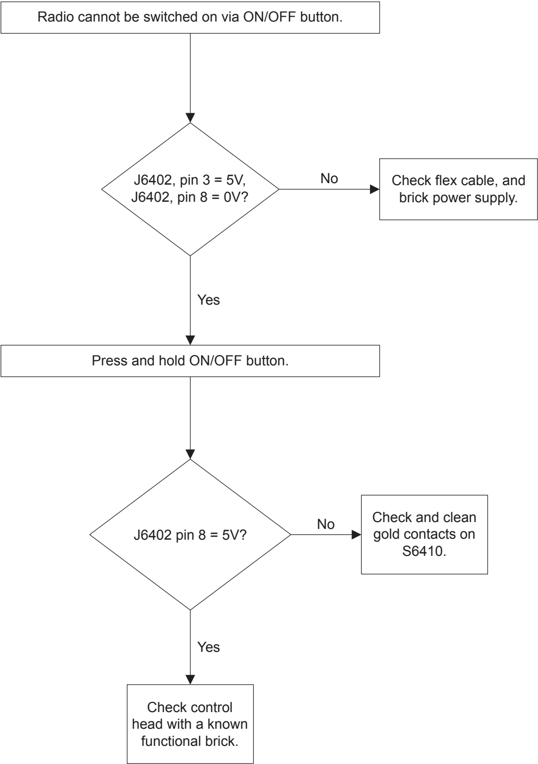
Figure 8: Troubleshooting Flow Chart for On/Off
