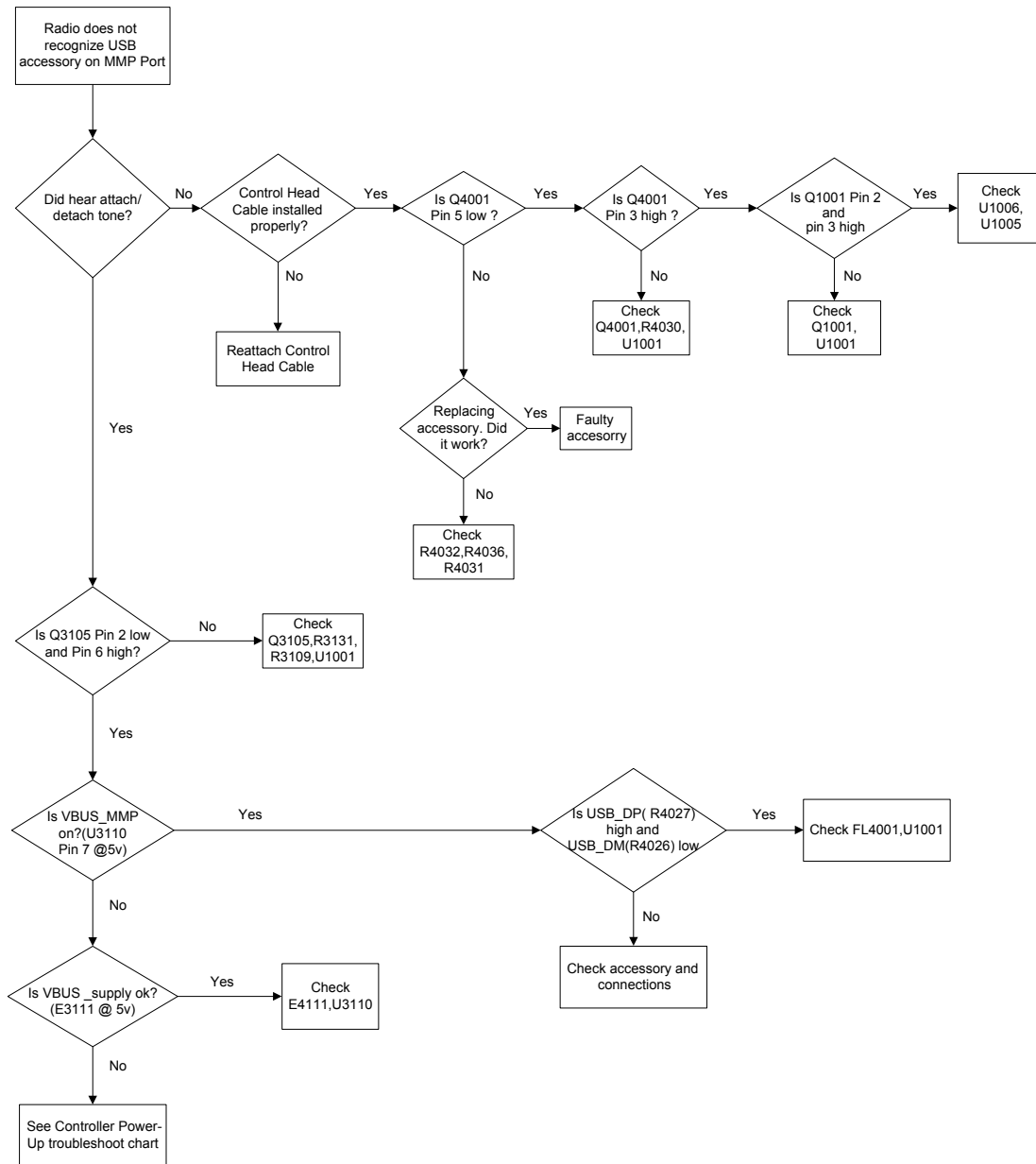
Figure 15: Troubleshooting Chart for MMP USB (Host Mode)
