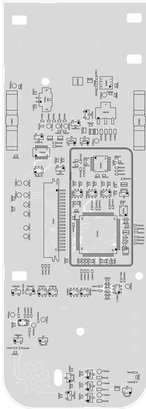
Figure 105: Colour Display Control Head Bottom Side PCB No. 84012211002-B
