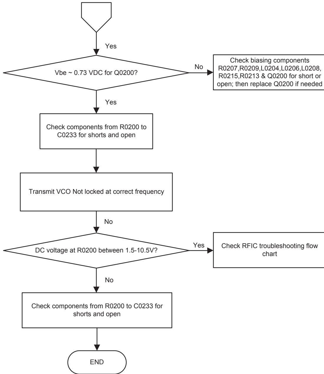
Figure 87: Troubleshooting Flow Chart for Tx VCO (Sheet 2 of 2)
