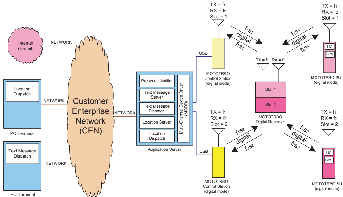
Figure 105: MOTOTRBO Radios in Digital Two-Slot Digital Repeater Mode with a Server-Based Configuration Using Control Stations and Remote Dispatchers
