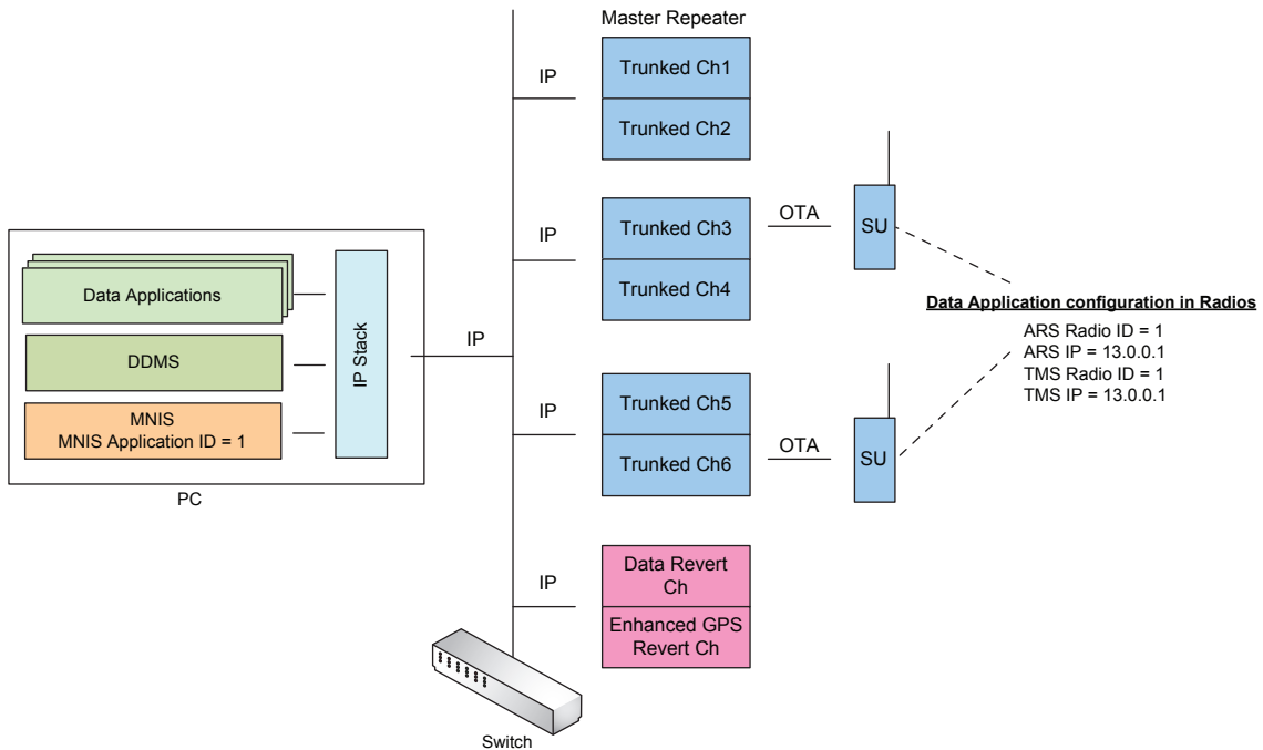
Figure 170: Capacity Plus Single Site System with MNIS Deployed Remotely
