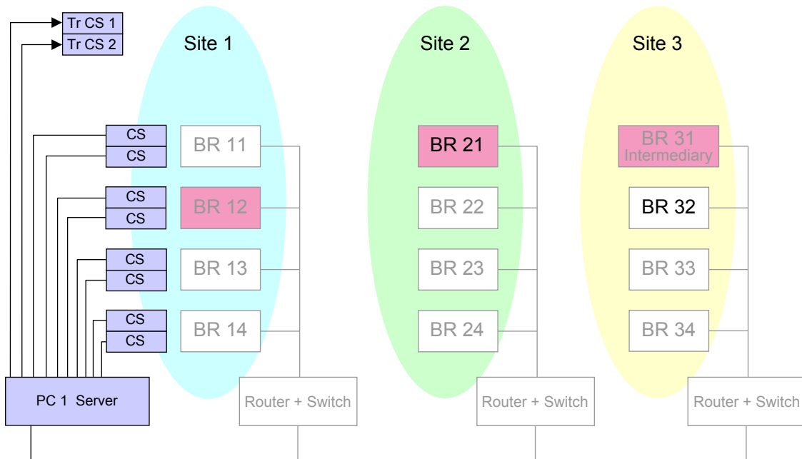
Figure 127: Capacity Plus Multi Site System with Data over Trunked Channels
