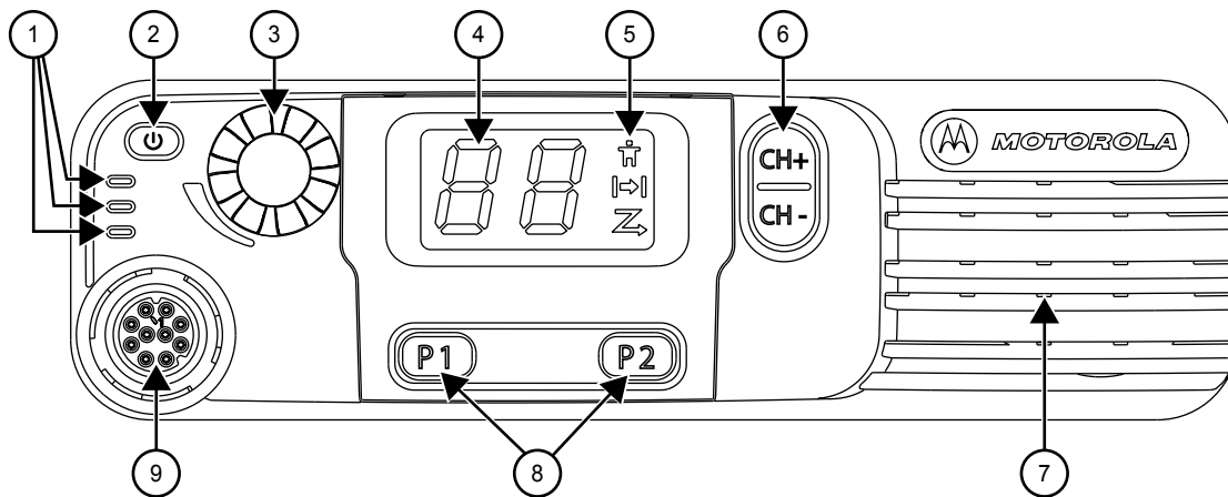
Figure 83: MOTOTRBO Mobile Control Head (Numeric Display Model)
