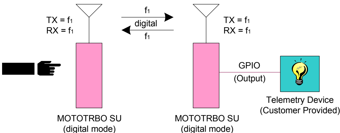
Figure 87: Send Telemetry Command from MOTOTRBO Radio to Another MOTOTRBO Radio to Toggle an Output Pin
