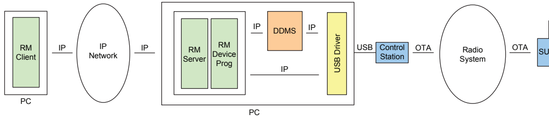
Figure 52: Remote RM Client from RM Server with Control Station
