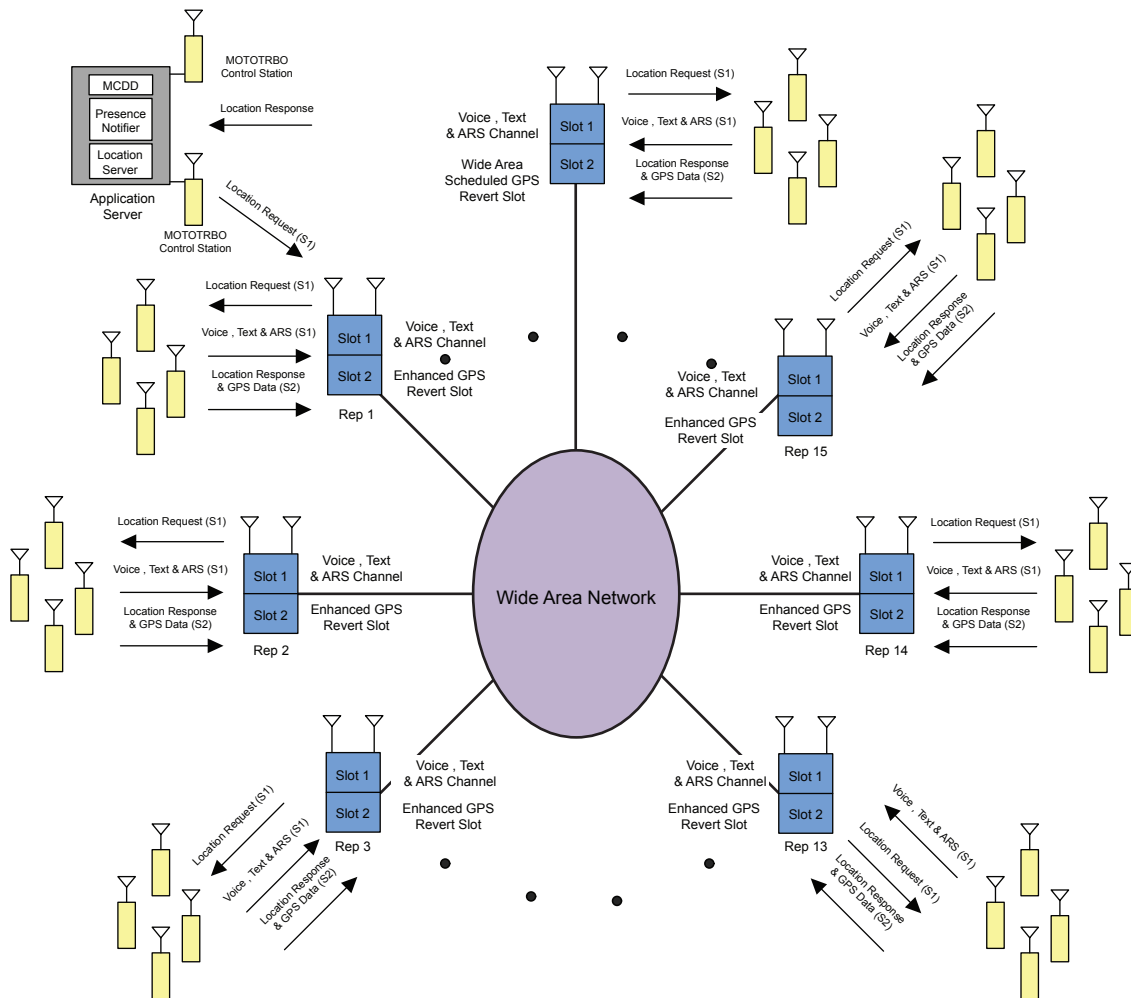
Figure 109: IP Site Connect System with an Enhanced GPS Revert Channel
