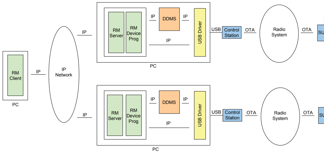
Figure 54: Remote RM Client with Multiple RM Servers with Control Station
