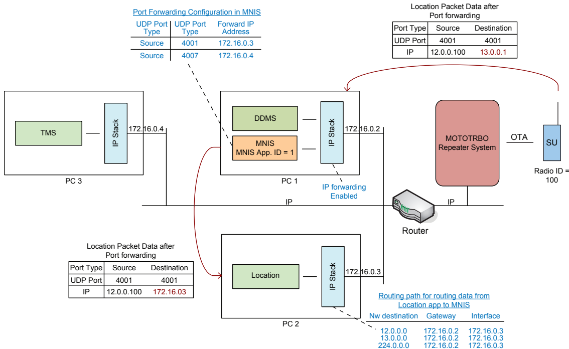
Figure 174: Application and MNIS Deployed on Separate Computers
