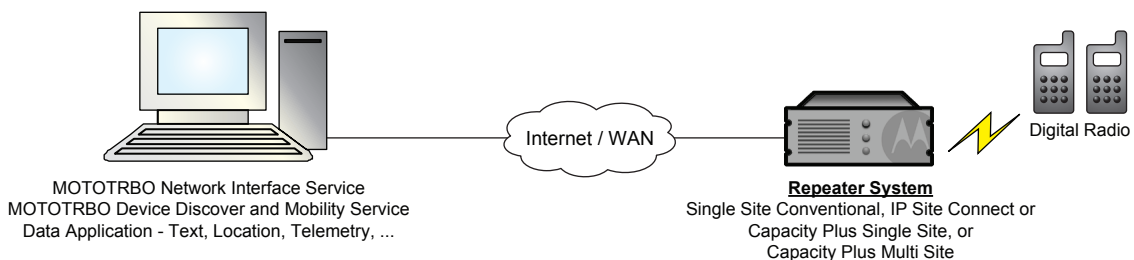
Figure 79: MOTOTRBO Network Interface Service (MNIS)
