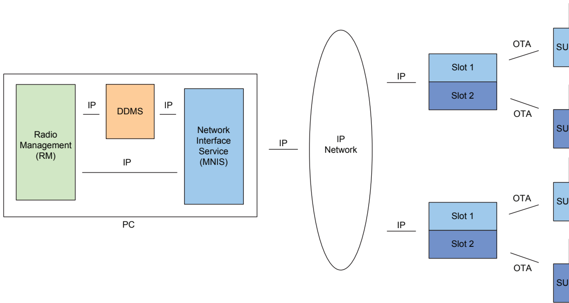
Figure 184: Multi-Channel RM Application with MNIS in Single Site or IP Site Connect Mode
