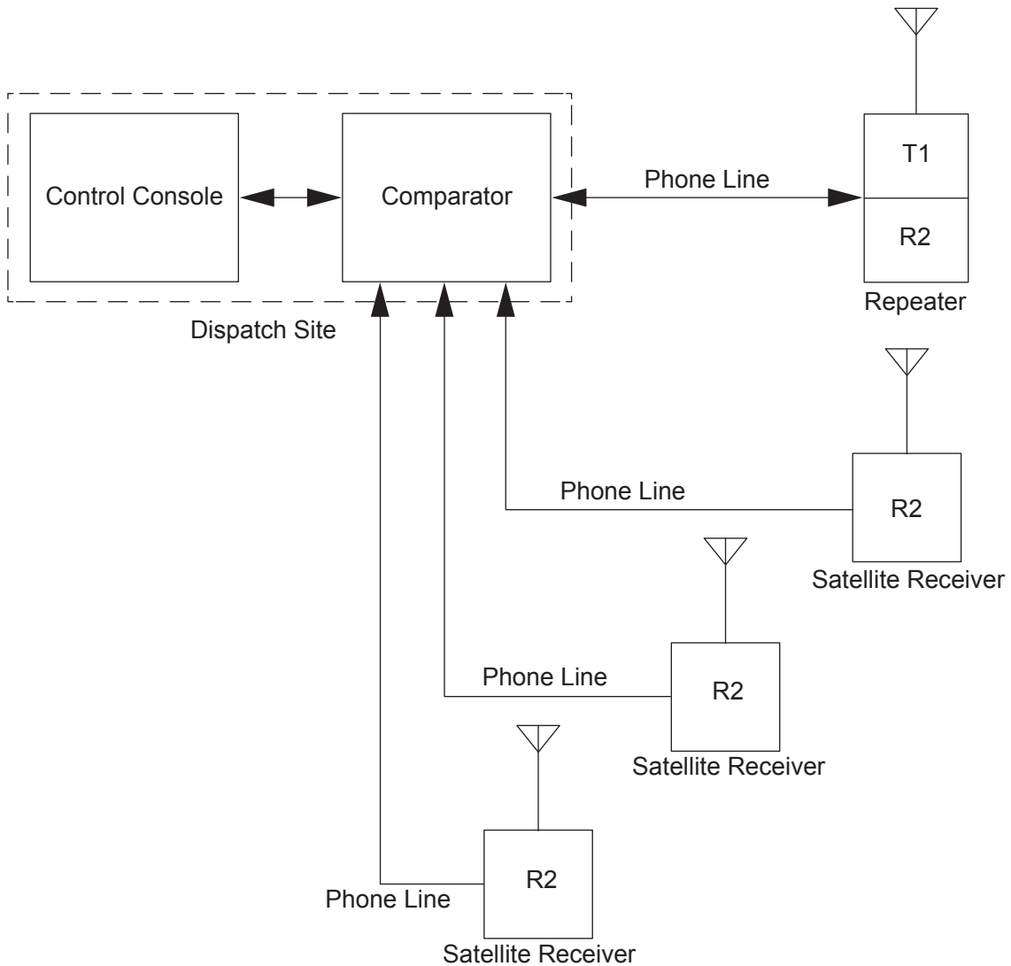
Figure 76: Satellite Receiver Connections Within a Voting System
