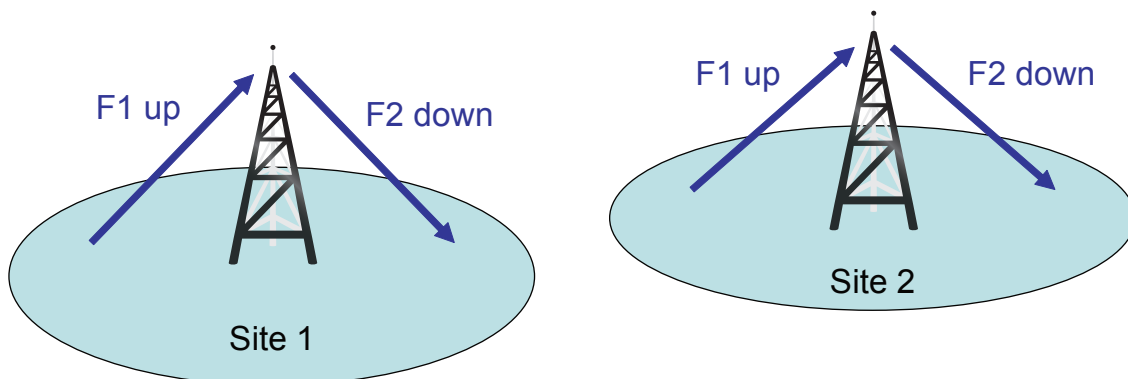
Figure 150: Multiple Repeaters
