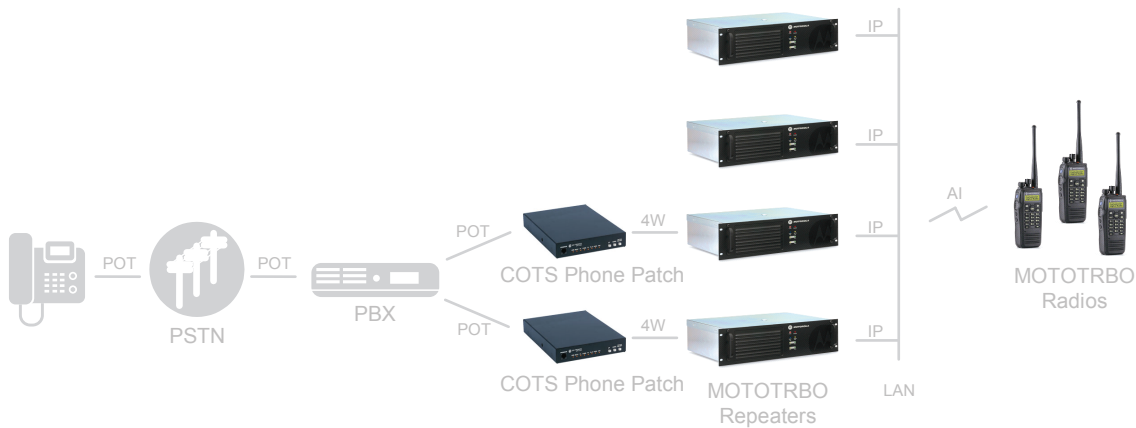
Figure 65: Phone Patch Topology in a Capacity Plus Single Site Configuration
