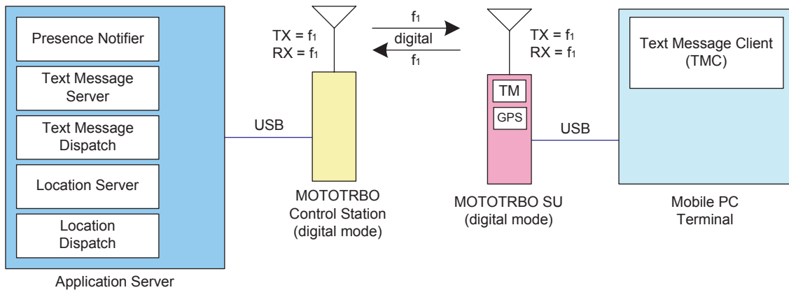
Figure 91: MOTOTRBO Radios In Digital Direct Mode with Text Message Server, Location Server and Local Dispatchers
