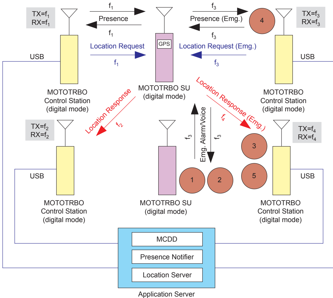
Figure 180: Emergency Alarm with Voice to Follow and GPS Revert Interaction Diagram
