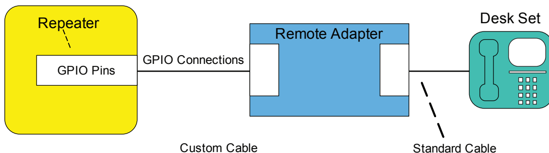
Figure 29: Local Connection Using GPIO Lines
