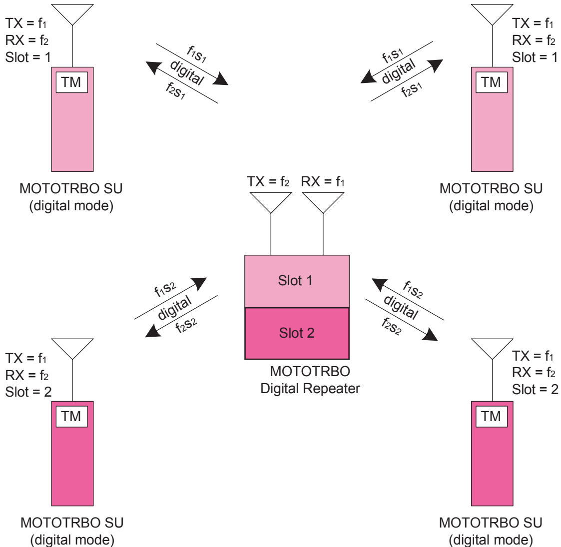
Figure 101: MOTOTRBO Radios in Digital Two-Slot Digital Repeater Mode with Built-In Text Messaging
