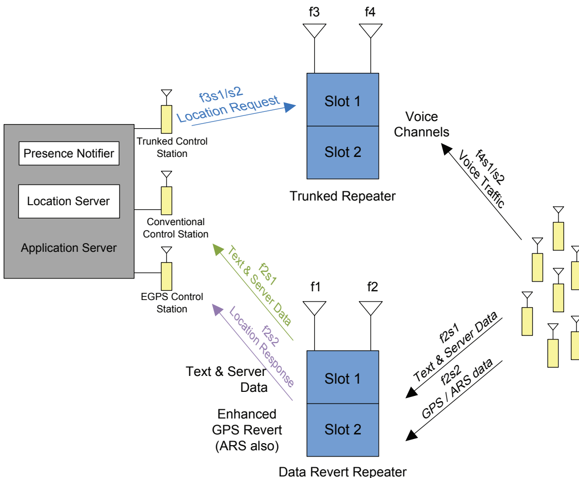
Figure 110: A Capacity Plus Single Site System with an Enhanced GPS Revert Channel
