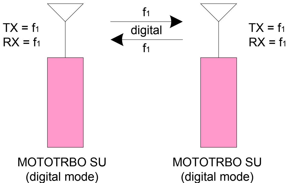
Figure 84: MOTOTRBO Radios (in digital mode) In Direct Mode/Dual Capacity Direct Mode
