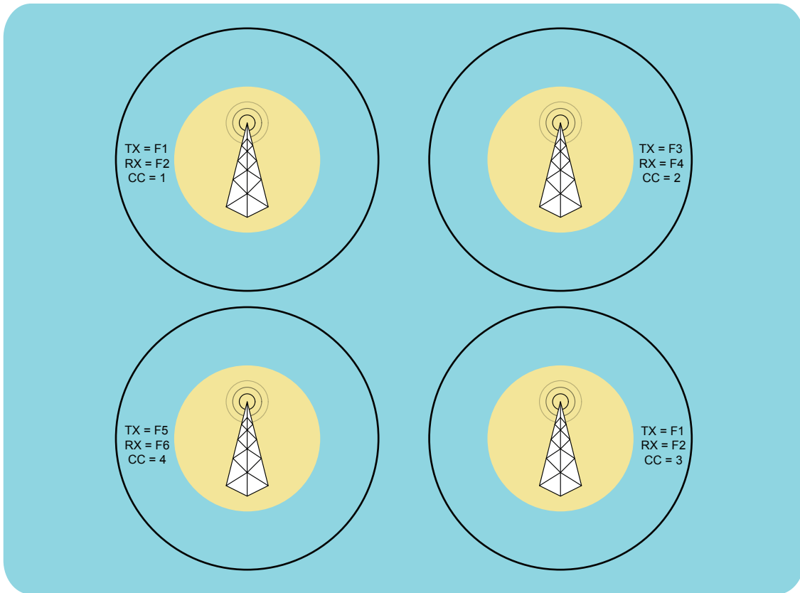
Figure 25: Isolated No Overlapping Coverage (Rural)
