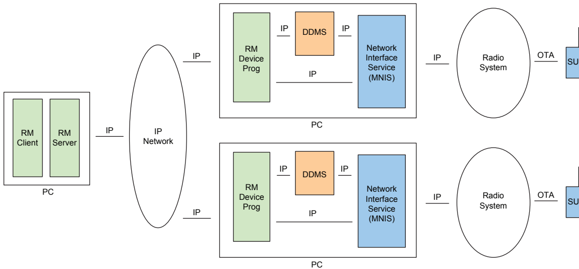
Figure 57: RM Server with Remote Device Programmers and MNIS
