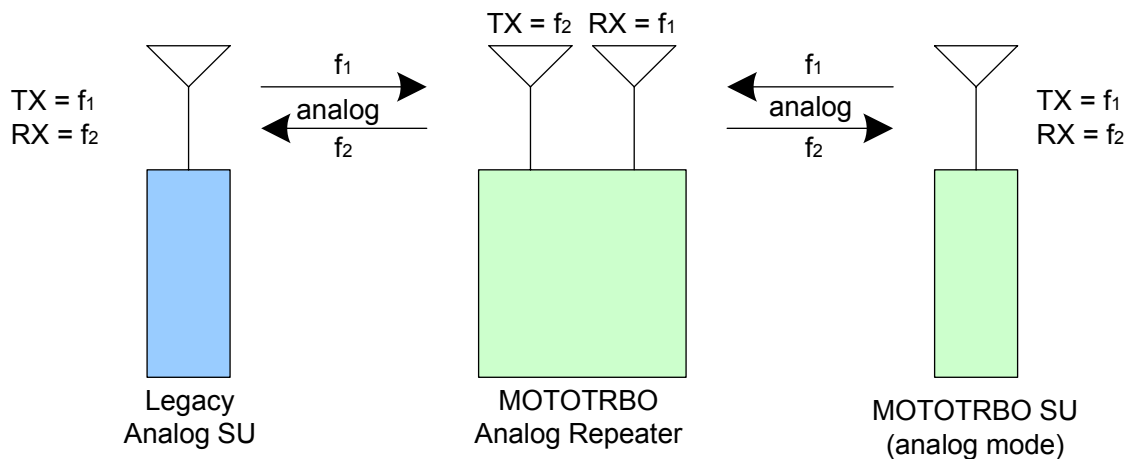
Figure 112: MOTOTRBO Analog and Legacy Analog Radios on MOTOTRBO Analog Repeater
