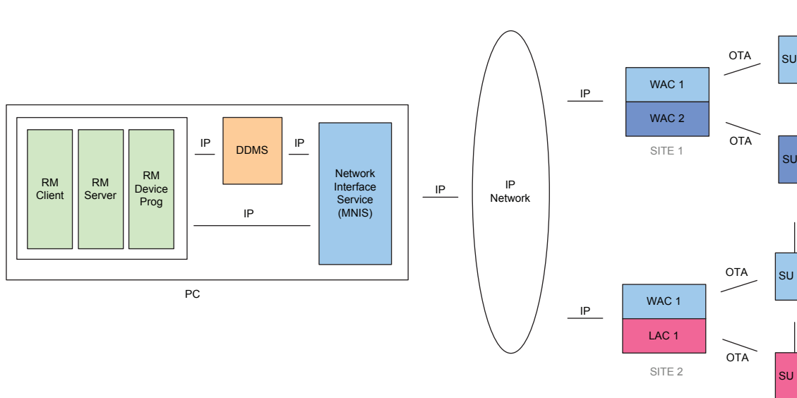
Figure 189: RM Application with MNIS in IP Site Connect Mode Covering Local Channels
