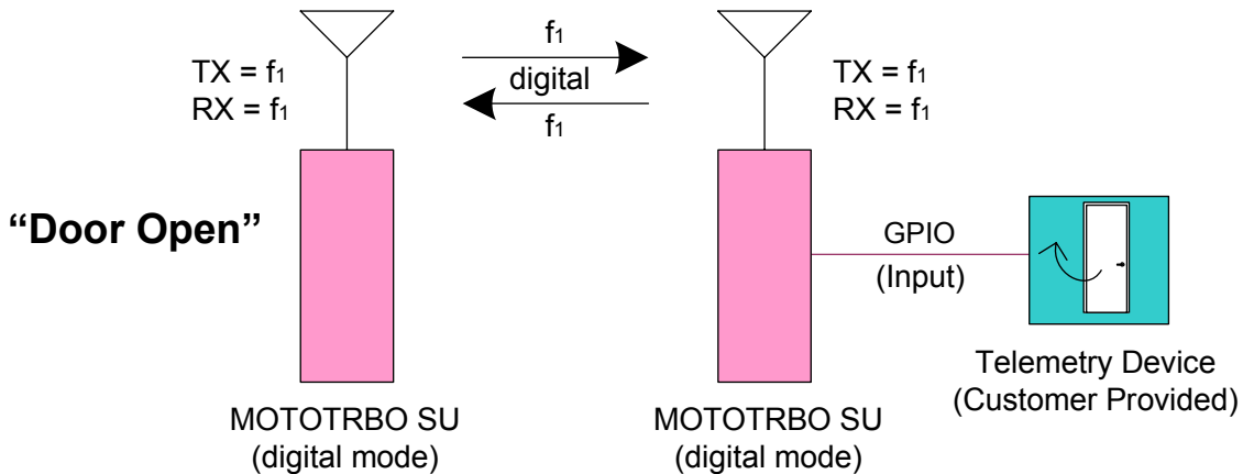
Figure 88: Send Telemetry Message from MOTOTRBO Radio to Another MOTOTRBO Radio when Input Pin State Changes
