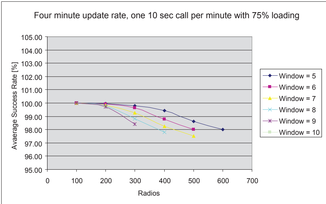
Figure 146: Four Minute Update Rate with a 10-second Call per Minute at 75% Loading
