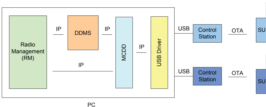
Figure 181: Multi-Channel RM Application with Control Stations in Direct Mode
