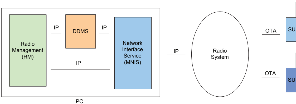
Figure 59: Multi-Channel Non-Remote RM Application Configuration with MNIS
