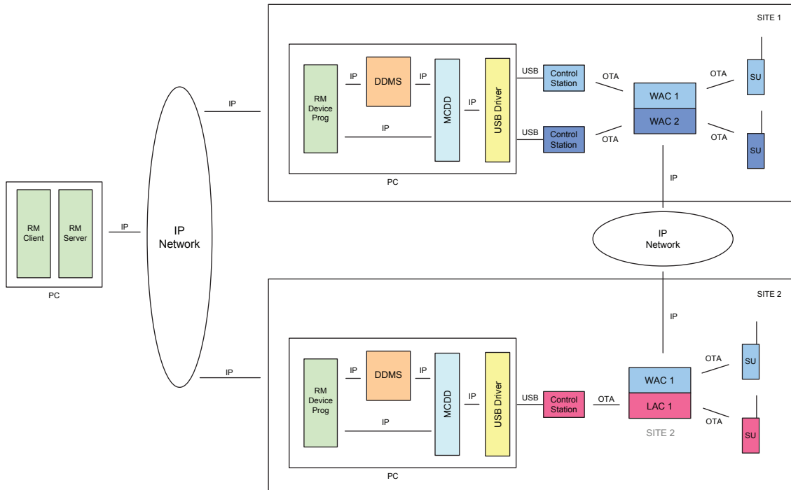
Figure 188: RM Application with Control Stations in IP Site Connect Mode Covering Local Channels with Remote Device Programmers
