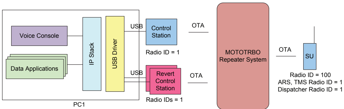
Figure 175: System with Control Stations Used by a Voice Console and Data Applications
