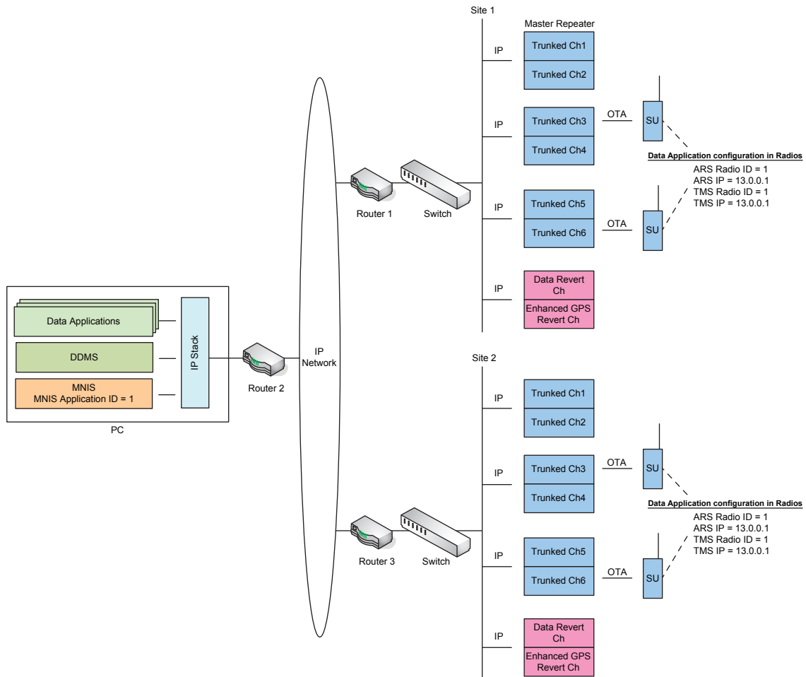
Figure 171: Capacity Plus Multi Site System with MNIS
