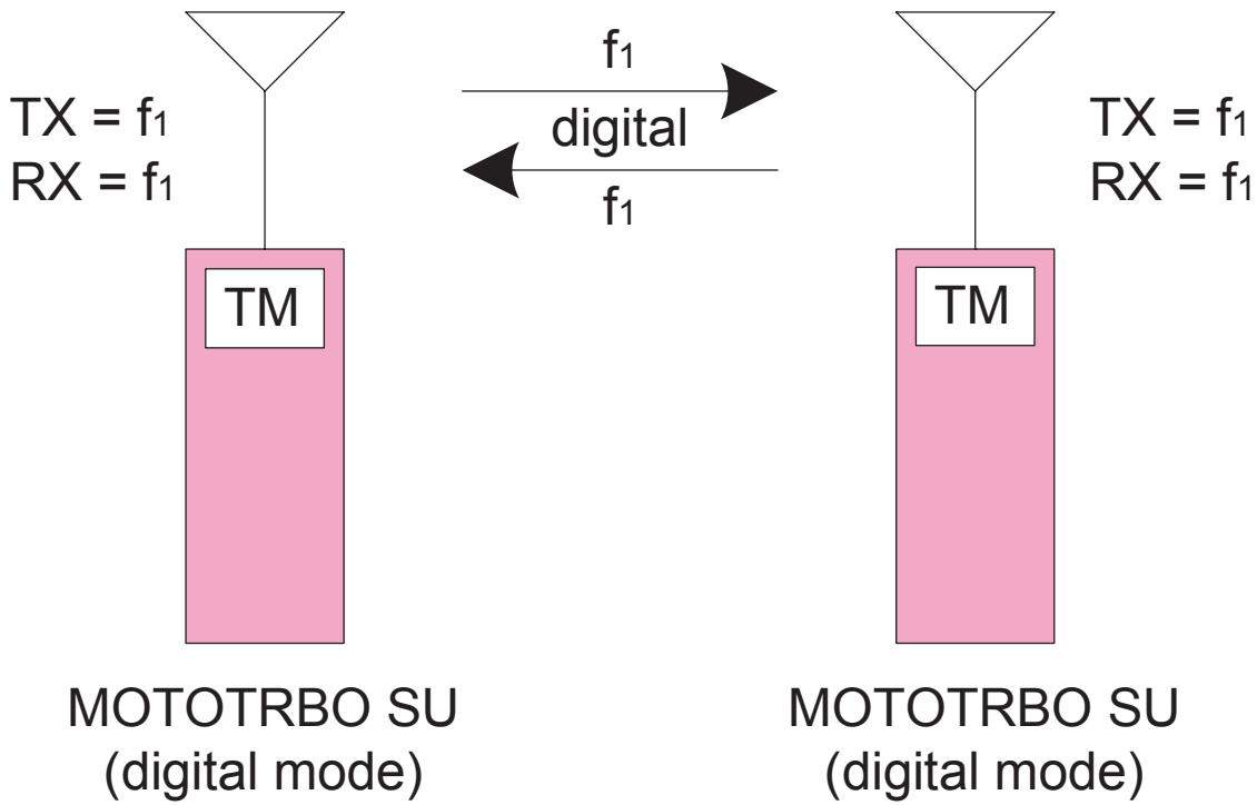
Figure 85: MOTOTRBO Radios (in digital mode) Text Messaging In Direct Mode/Dual Capacity Direct Mode
