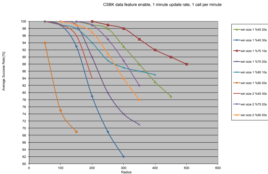
Figure 149: One Minute Update Rate with Different Window Sizes, Loading and Call Duration
