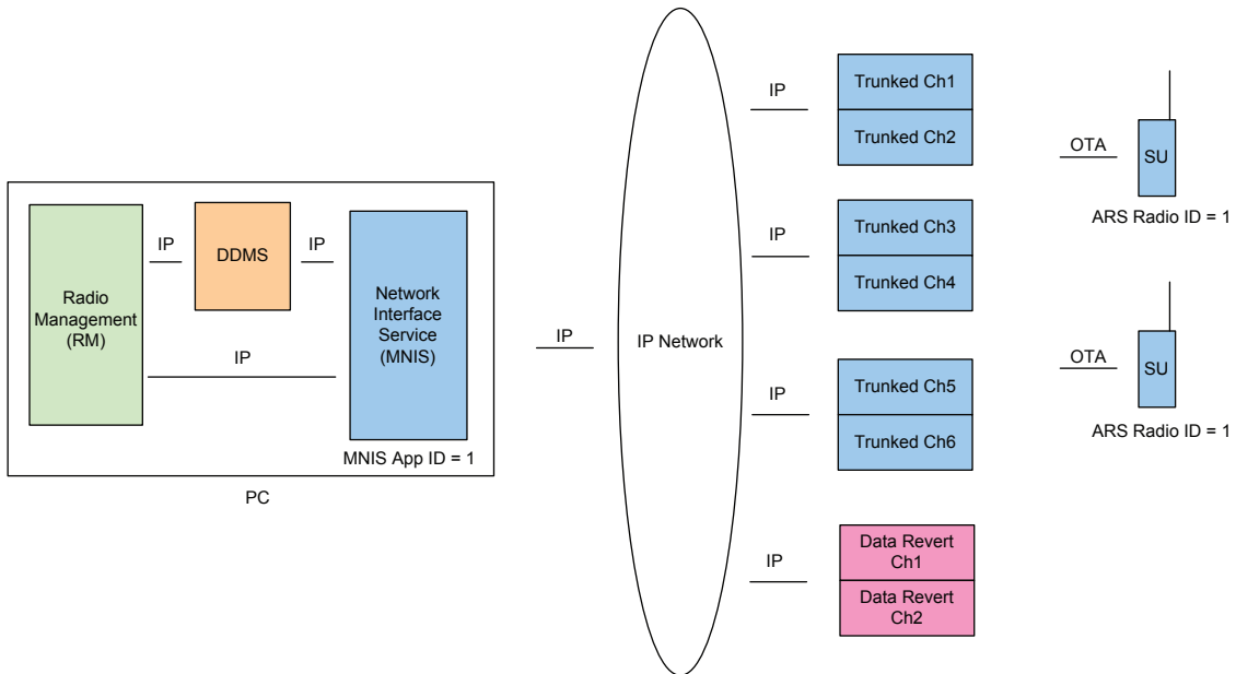
Figure 197: RM Application in a Capacity Plus System with a MNIS and a DDMS, and Data Revert Channels
