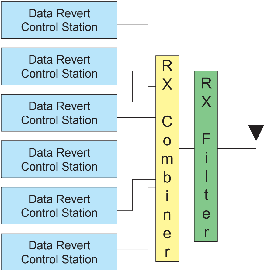
Figure 212: Installation of Control Stations for Unconfirmed Data
