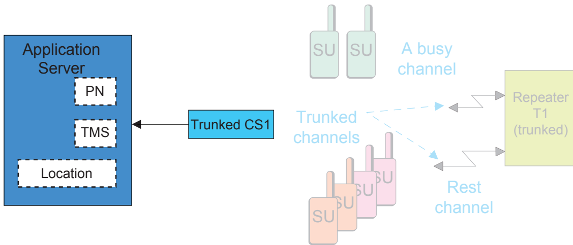
Figure 124: Two-Channel Capacity Plus Single Site Devices with Data over Trunked Channels
