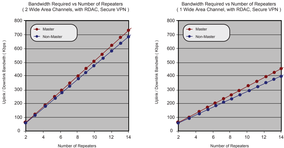
Figure 158: Required Bandwidth Calculations While Utilizing a Secure Virtual Private Network
