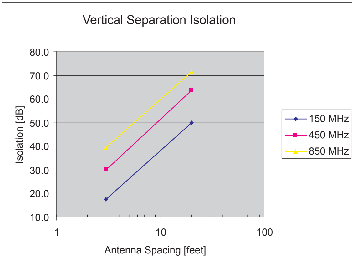
Figure 215: Vertical Separation Isolation
