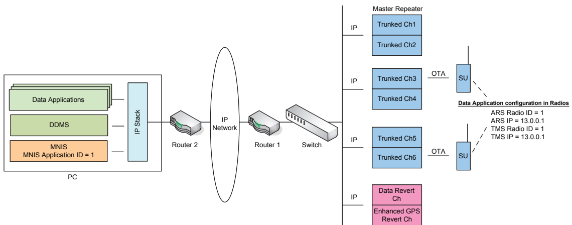
Figure 170: Capacity Plus Single Site System with MNIS Deployed Remotely
