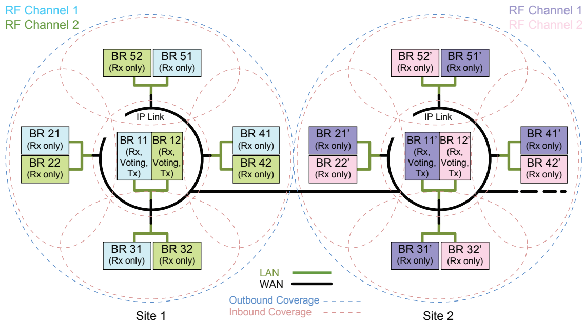
Figure 133: Digital Voting Topology for a Two-Site Capacity Plus Multi Site System
