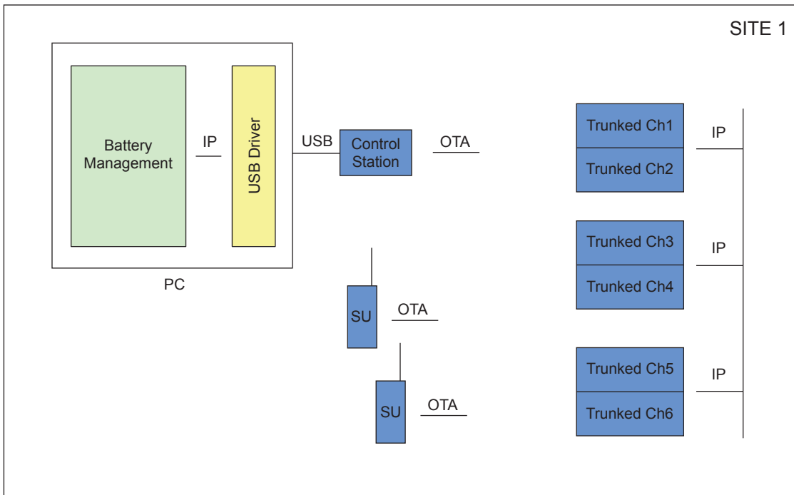
Figure 40: BMA Deployment in Capacity Plus with a Control Station
