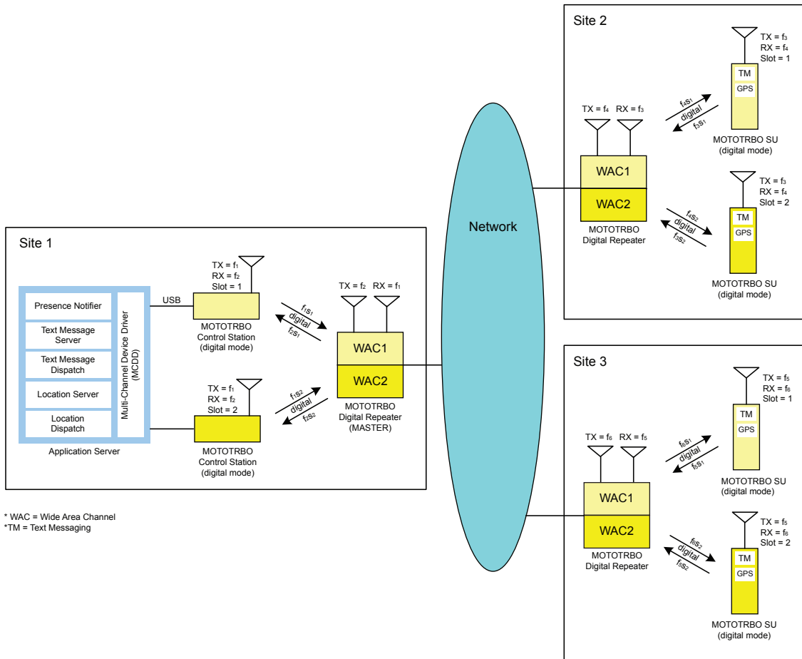
Figure 114: Wide Area System with Centralized Data Application Server
