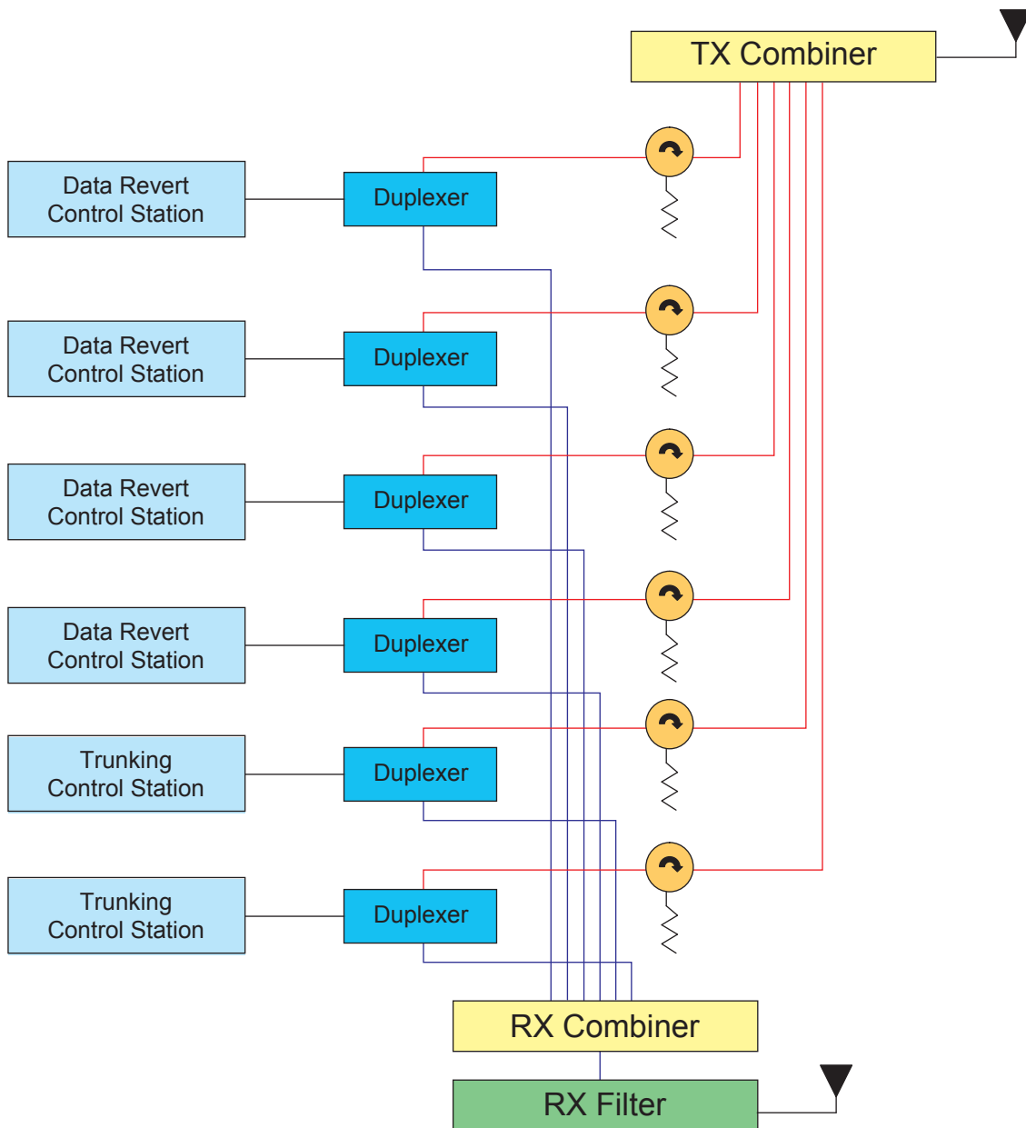
Figure 213: Installation of Control Stations for Confirmed Data
