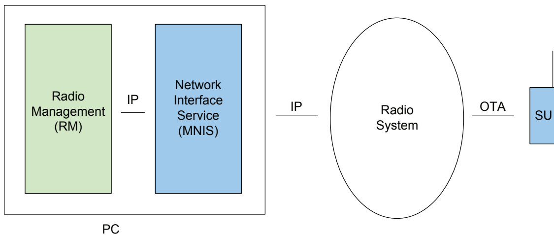
Figure 48: Single Channel Non-Remote RM Application Configuration Through MNIS
