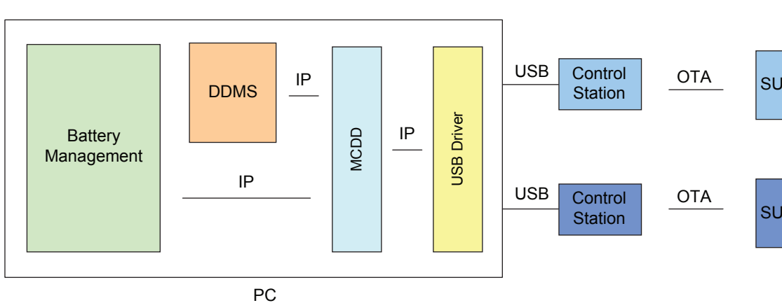
Figure 37: BMA Deployment in Multi-Channel Direct Mode with Control Stations
