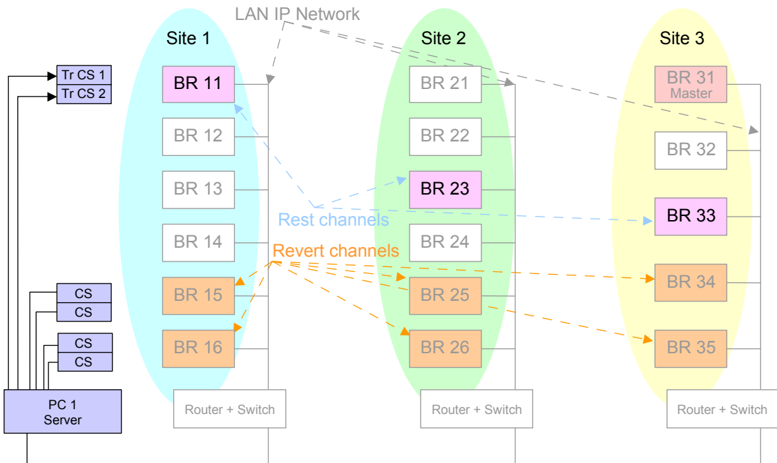
Figure 129: Capacity Plus Multi Site System with Data over Wide Area Revert Channels
