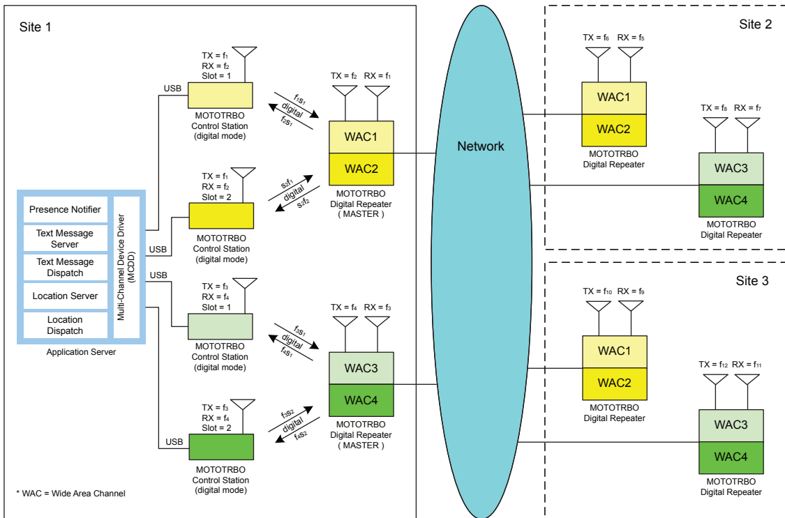
Figure 116: Multiple Wide Area Systems with Centralized Data Application Server
