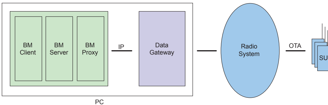
Figure 43: BMA Deployment with Client, Server and Proxy on the Same PC
