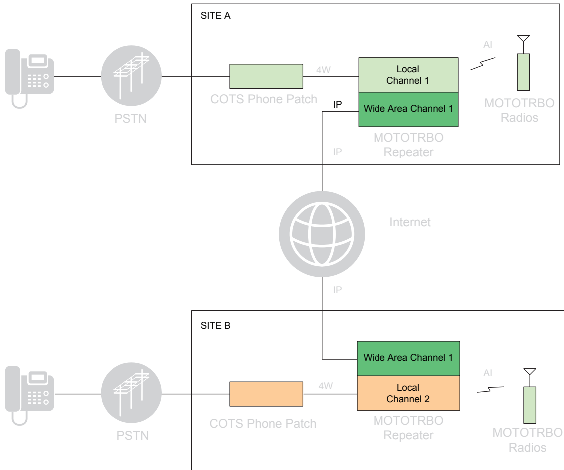
Figure 61: Phone Patch Topology in IP Site Connect Local Area Channel Configuration
