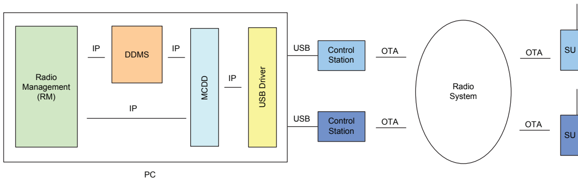
Figure 58: Multi-Channel Non-Remote RM Application Configuration with Control Stations
