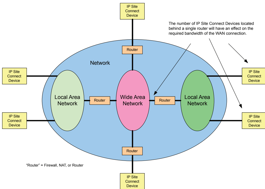
Figure 119: IP Site Connect Devices connected through Local Area and Wide Area Network
