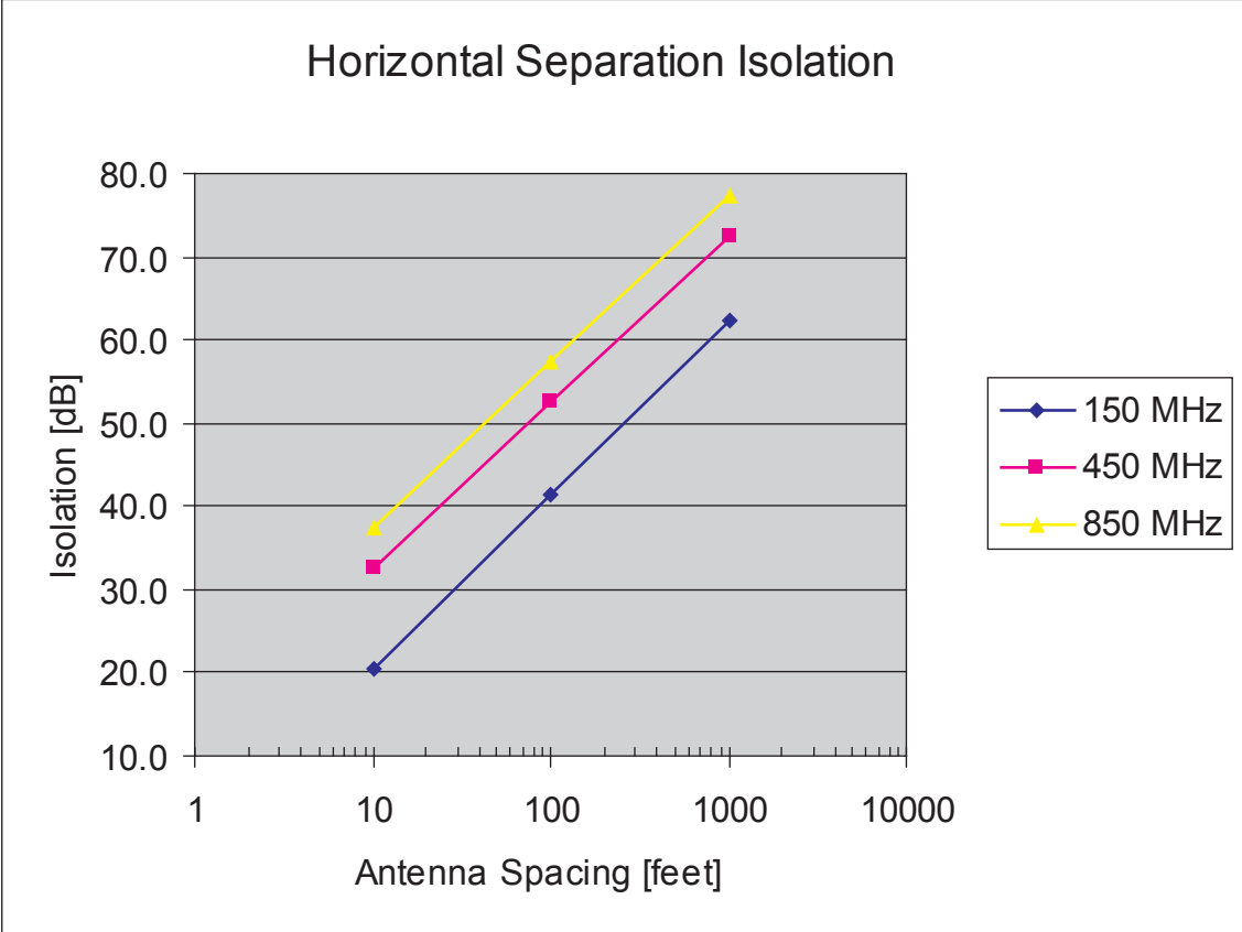
Figure 214: Horizontal Separation Isolation
