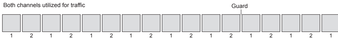
Figure 98: Dual Capacity Direct Mode Channels
