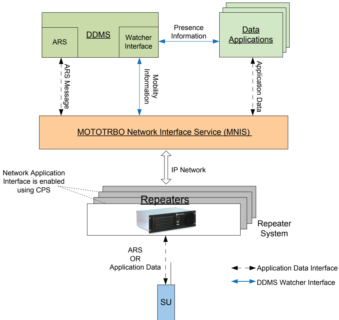
Figure 166: MNIS and DDMS Interface Overview
