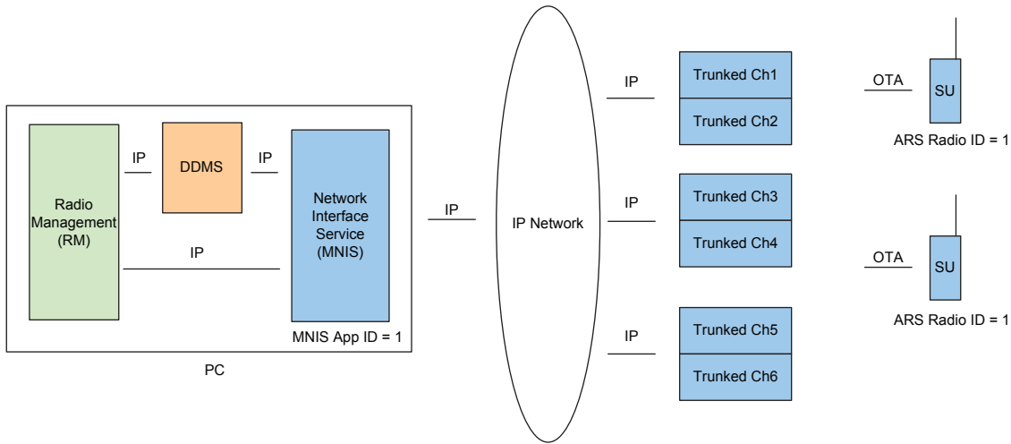
Figure 196: RM Application in a Capacity Plus System with a MNIS and a DDMS
