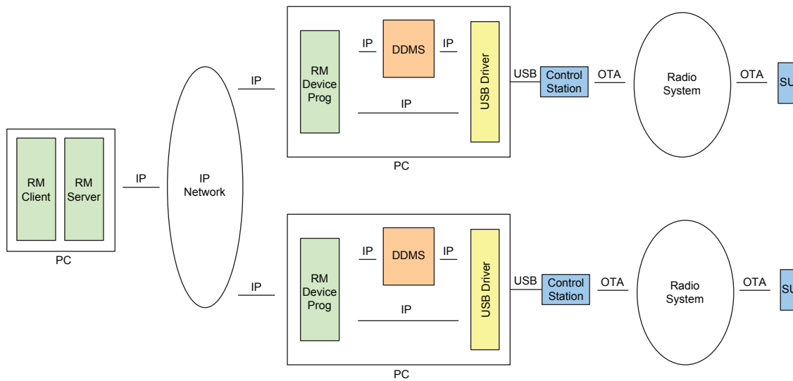
Figure 56: RM Server with Remote Device Programmers and Control Stations
