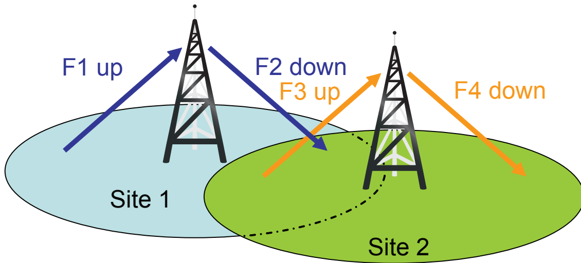
Figure 151: Multiple Repeaters with Overlap
