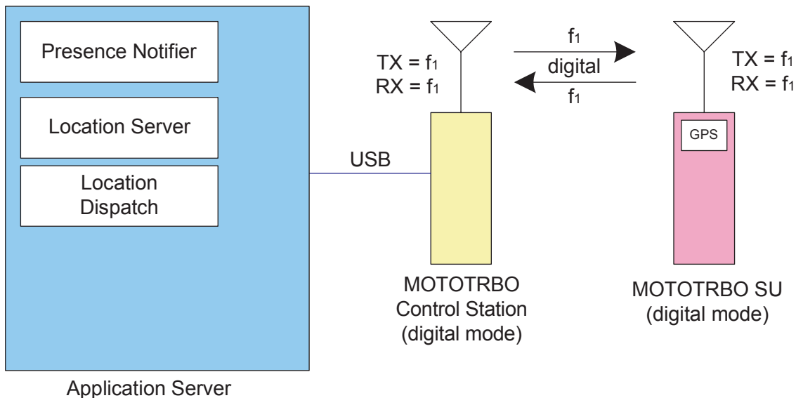
Figure 90: MOTOTRBO Radios In Digital Direct Mode/Dual Capacity Direct Mode with Location Server and Local Location Client
