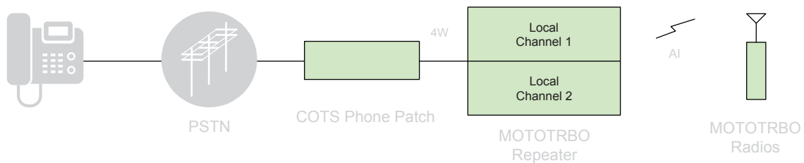
Figure 60: Phone Patch Topology in Single Site Configuration
