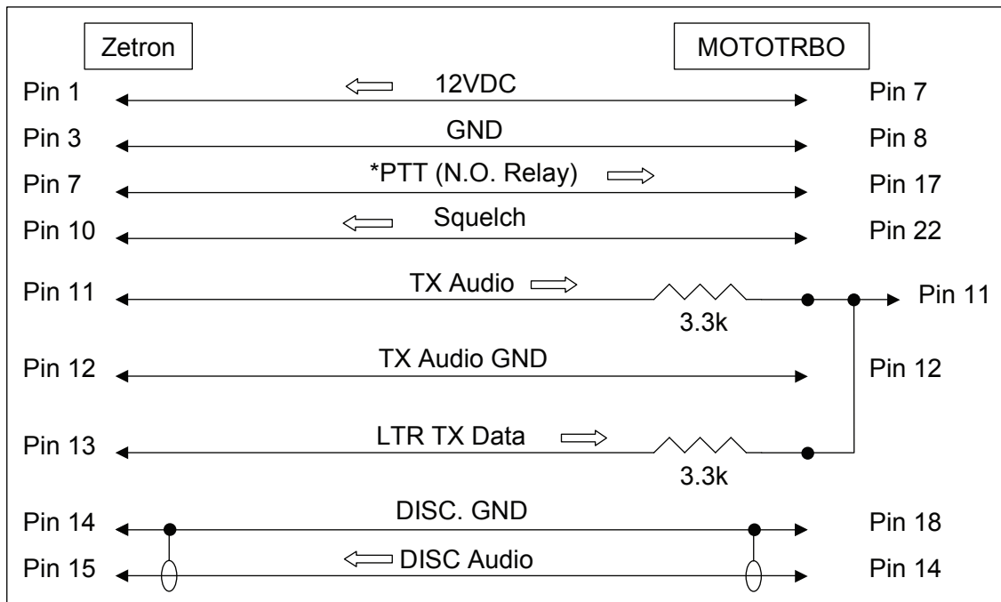
Figure 69: XPR 8300/XPR 8380/XPR 8400 Cable Schematic for Zetron Controllers
