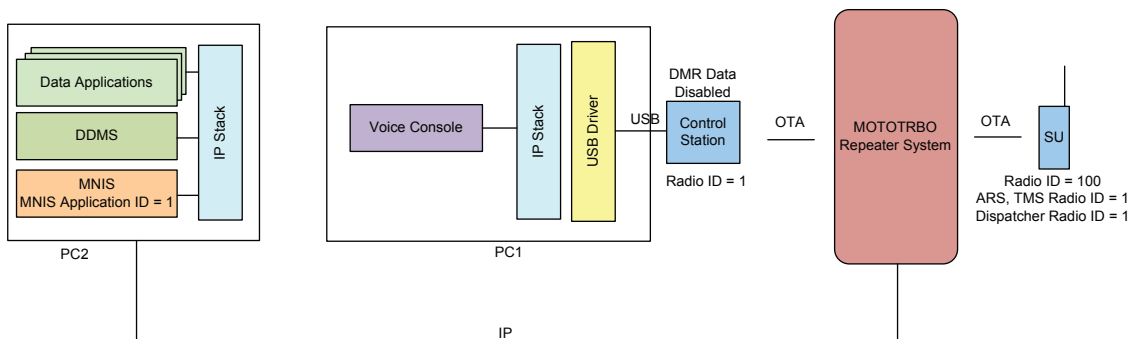
Figure 176: System with a Control Stations Used by a Voice Console and MNIS Used by Data Applications
