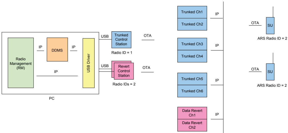
Figure 194: RM Application in a Capacity Plus System with a DDMS, Data Revert Channels, and Control Stations
