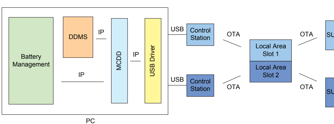
Figure 36: BMA Deployment in Single Channel Direct Mode with Control Stations
