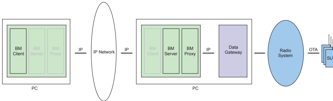
Figure 44: BMA Deployment with Client Remote from Server and Proxy
