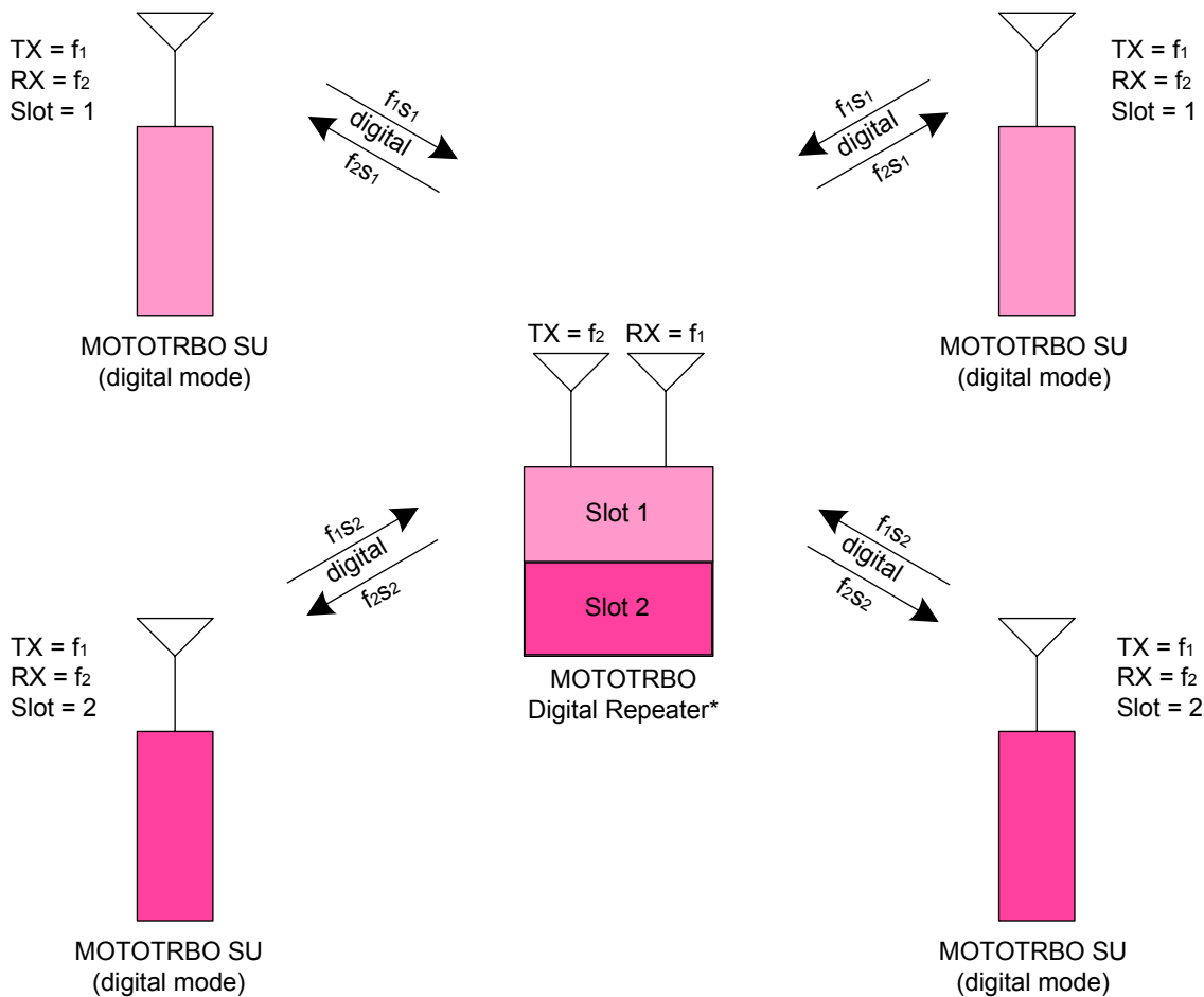
Figure 100: MOTOTRBO Digital Radios on MOTOTRBO Two-Slot Digital Repeater
