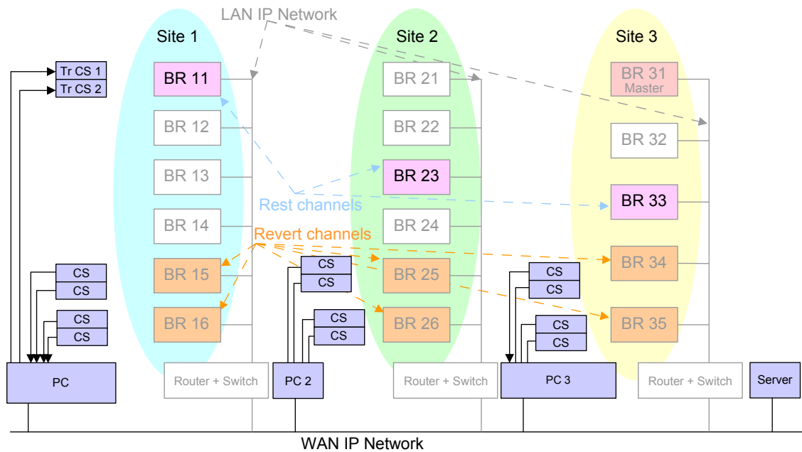
Figure 128: Capacity Plus Multi Site System with Data over Local Revert Channels
