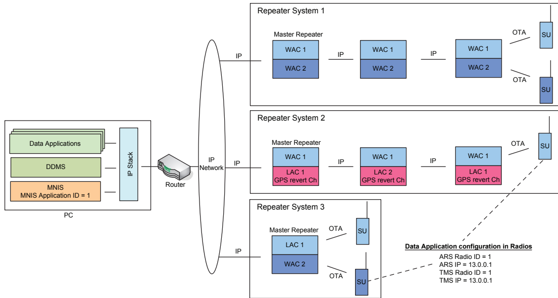
Figure 168: Multiple Conventional Systems with MNIS
