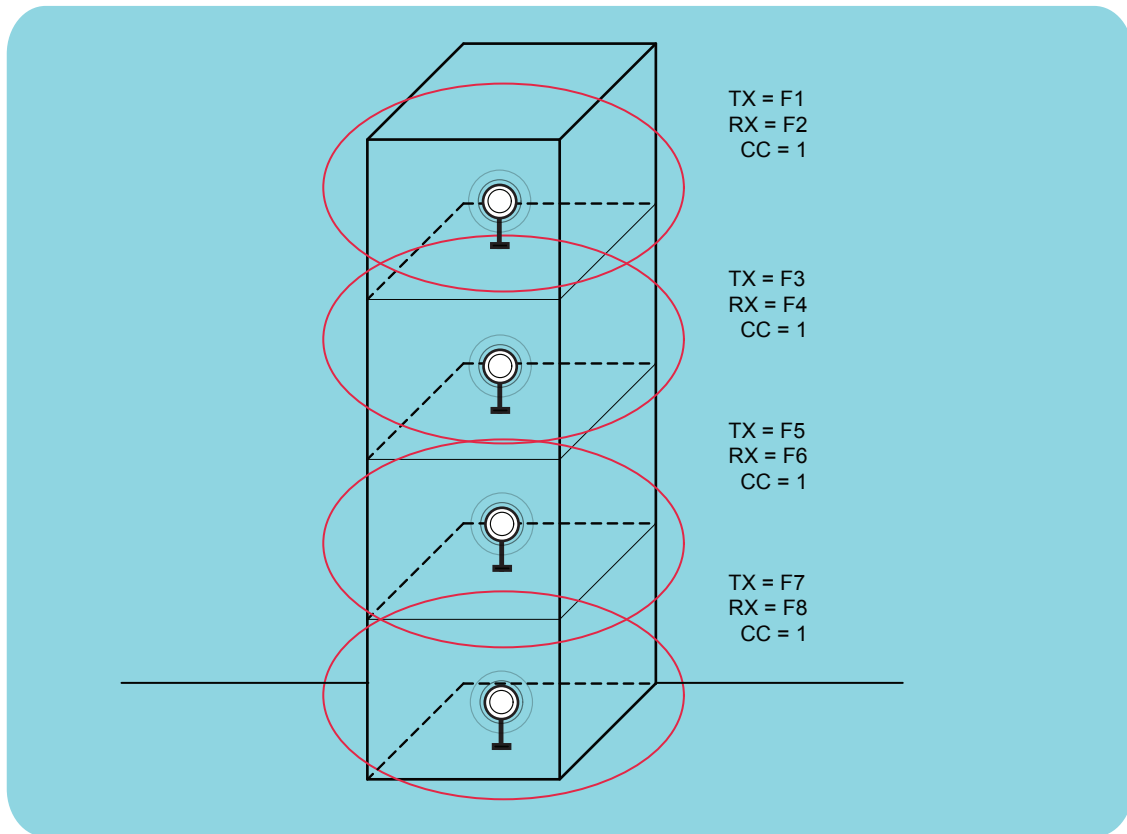
Figure 27: Multi-Floor Coverage
