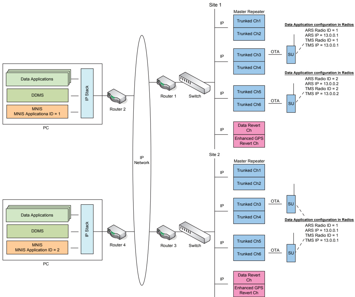
Figure 172: Capacity Plus Multi Site System with Two MNIS
