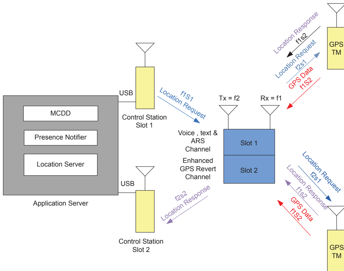
Figure 108: Single Site Conventional System with an Enhanced GPS Revert Channel
