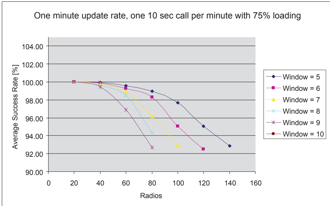
Figure 145: One Minute Update Rate with a 10-second Call per Minute at 75% Loading
