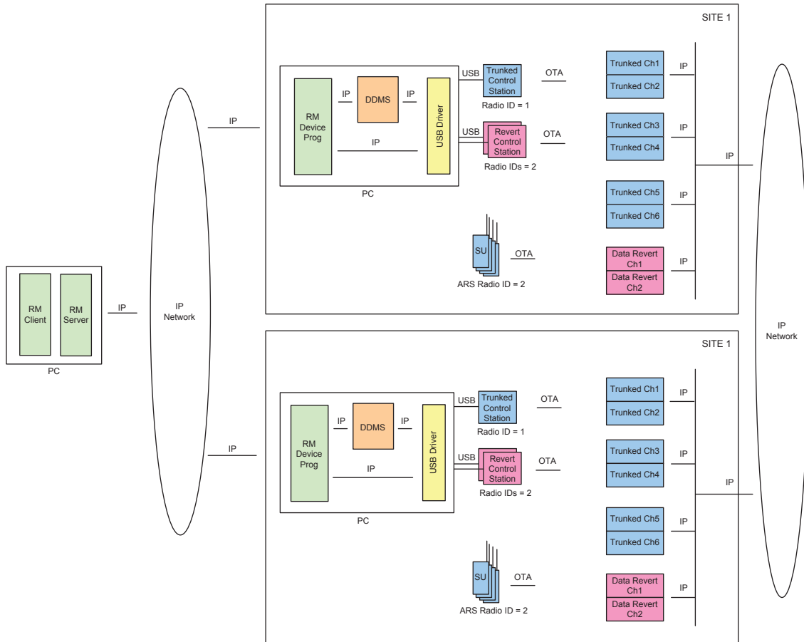
Figure 199: RM Application with Control Stations in a Capacity Plus Multi Site System with Presence (DDMS) and Local Area Data Revert Channels
