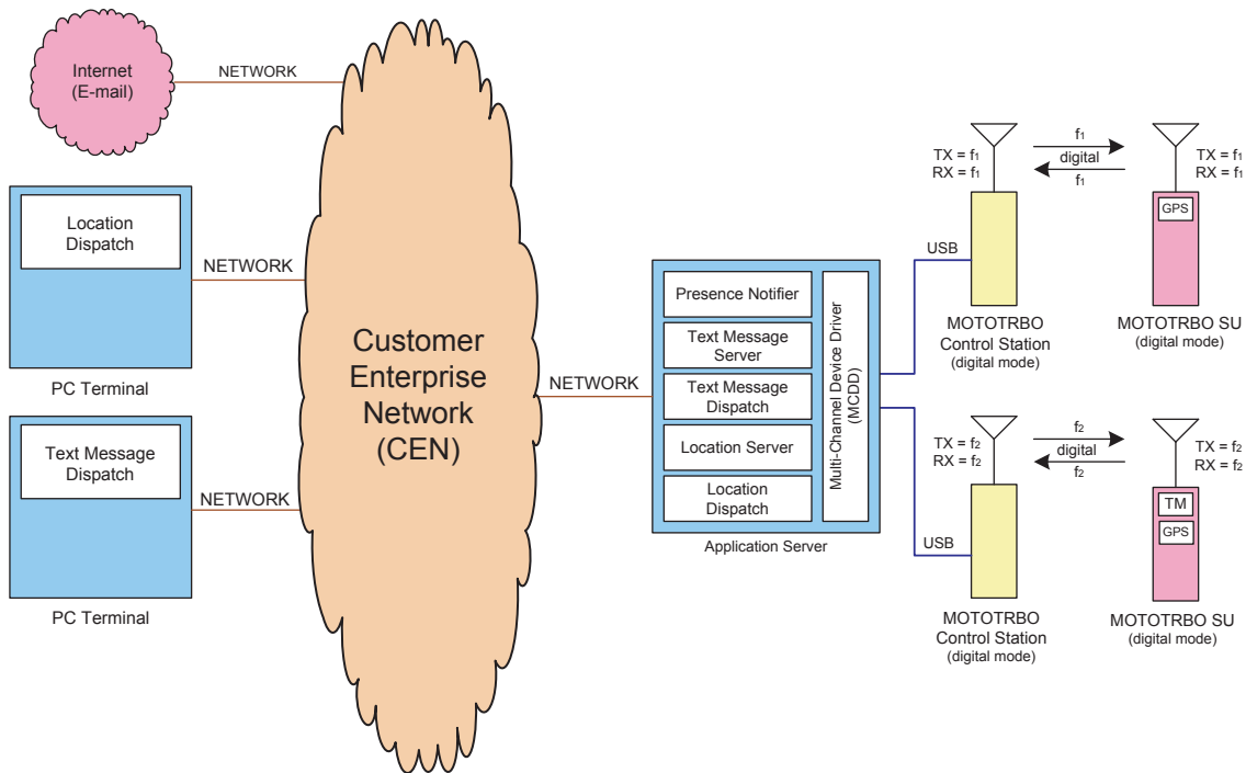
Figure 93: MOTOTRBO Radios in Two Channel Digital Direct Mode Server-Based Configuration with Remote Dispatchers
