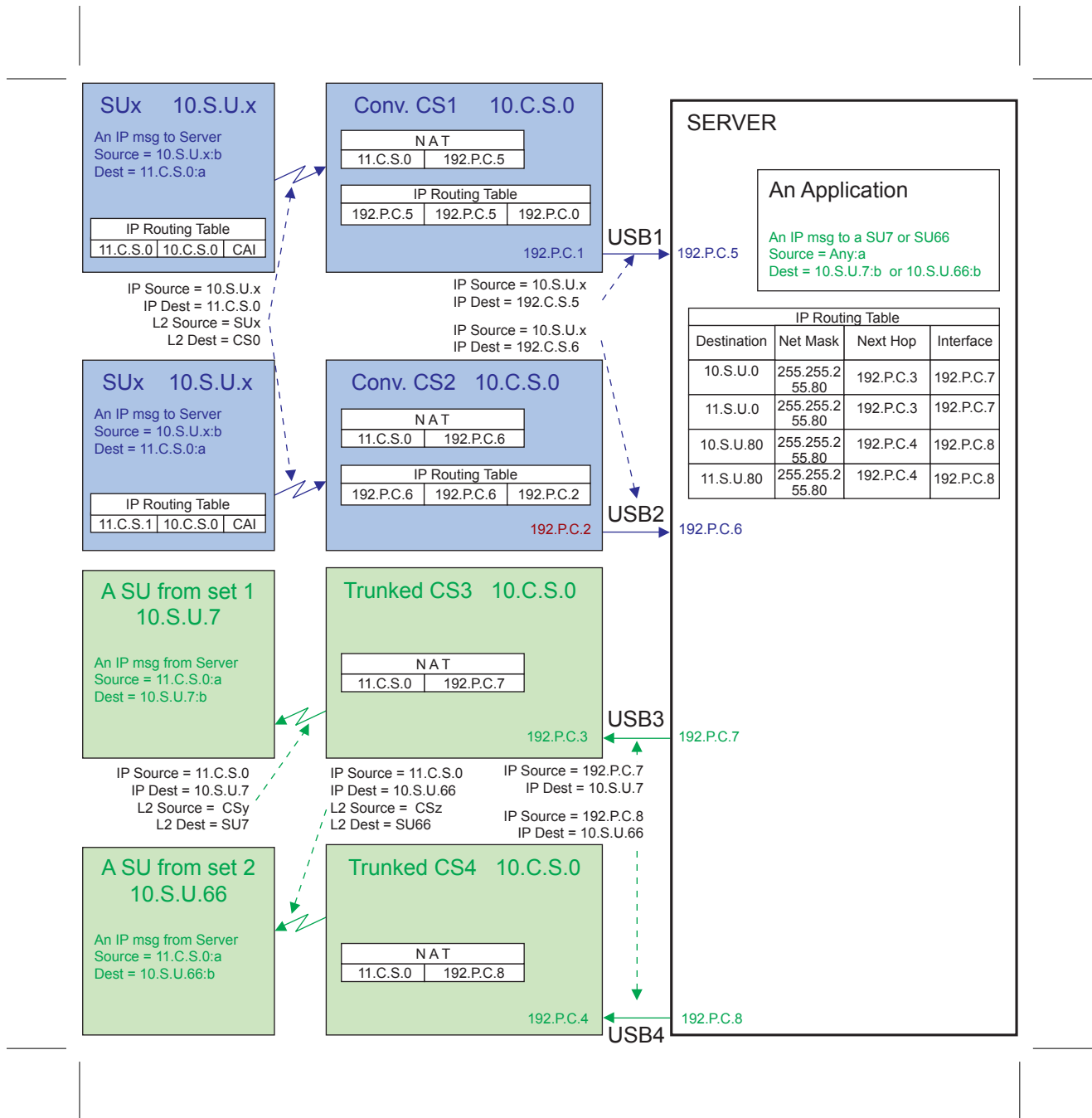
Figure 165: An example showing IPv4 addresses in a Capacity Plus Single Site Configuration with Data Revert
