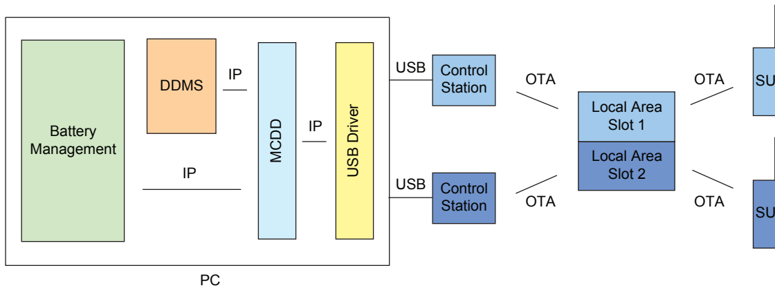
Figure 38: BMA Deployment in Single Site with Control Stations
