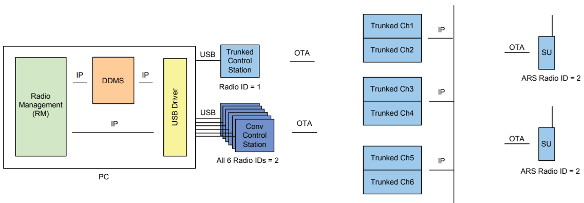
Figure 193: RM Application in a Capacity Plus System with a DDMS and One Trunked and Numerous Conventional Control Stations
