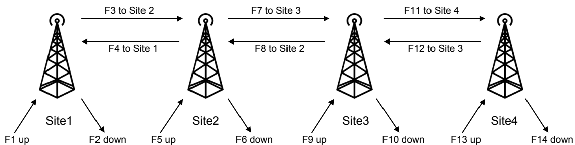
Figure 209: Example of a Dedicated MOTOTRBO Link System with Four Backhaul Sites
