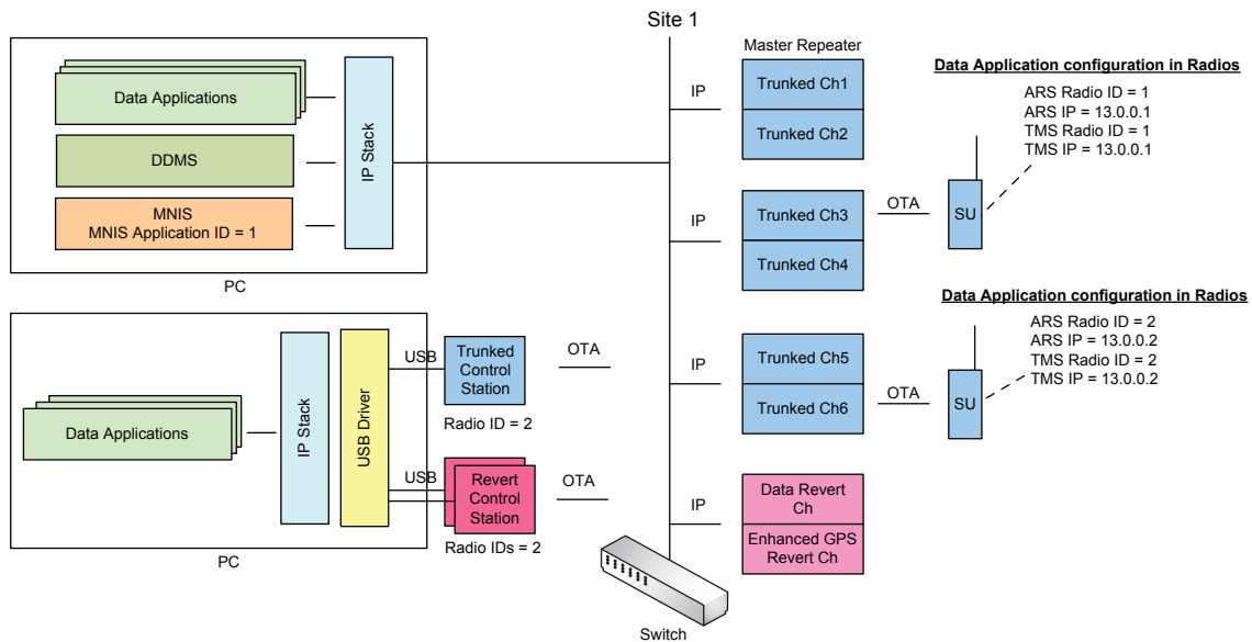
Figure 173: Capacity Plus Single Site System with MNIS and Control Stations
