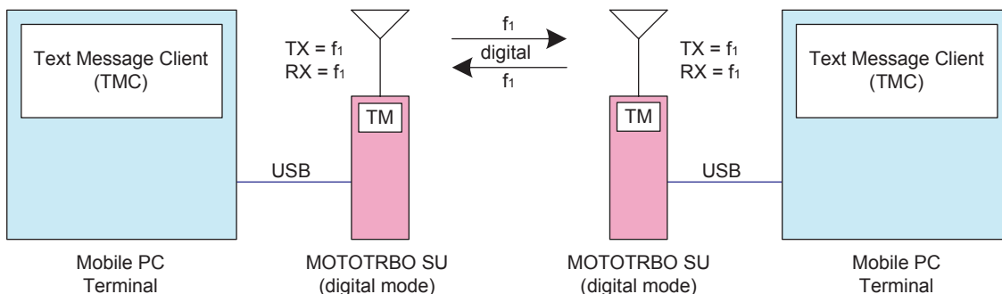
Figure 86: MOTOTRBO Radios (in digital mode) Text Messaging In Multiple Direct Mode/Dual Capacity Direct Mode
