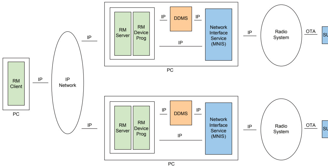
Figure 55: Remote RM Client with Multiple RM Servers with MNIS
