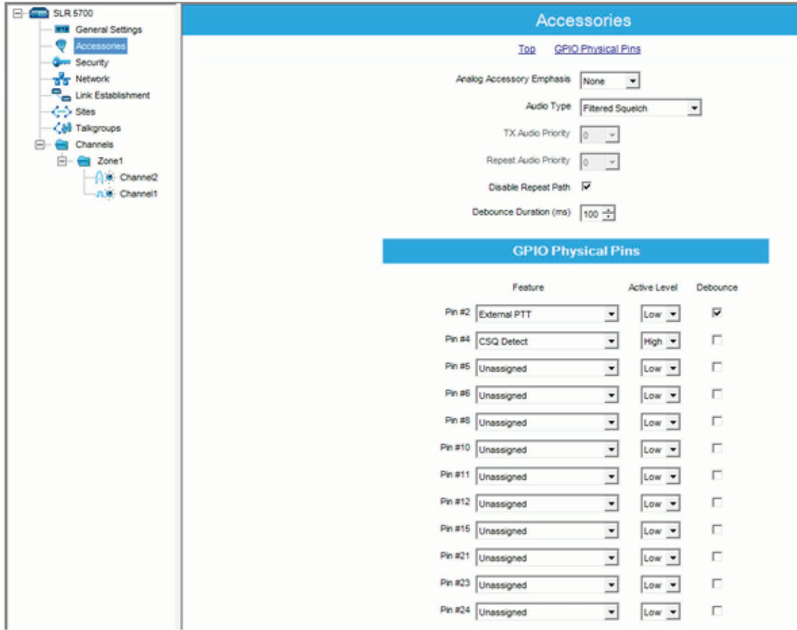
Figure 71: CPS Configuration for M827/M807 Controller (1 of 2)
