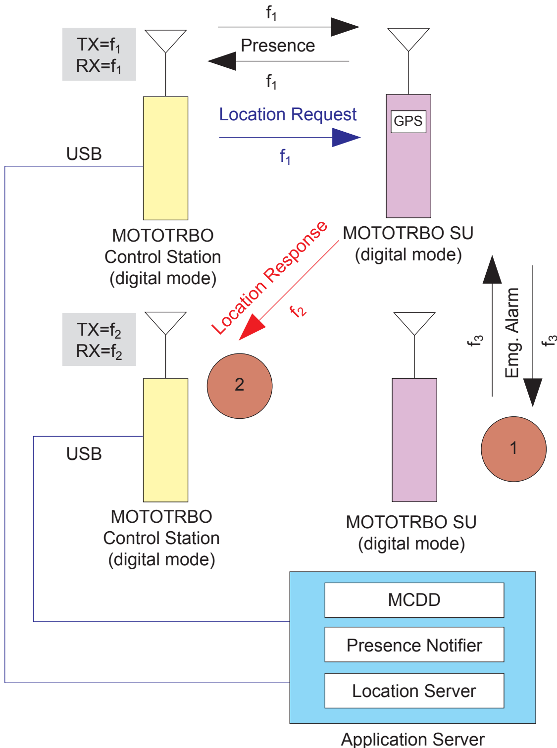
Figure 178: Emergency Alarm and GPS Revert Interaction Diagram
