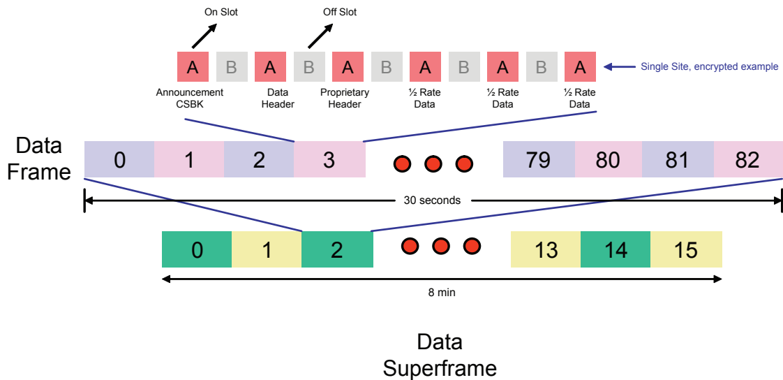
Figure 18: GPS Revert Channel Location Windows Data Structure for a Window Size of Six
