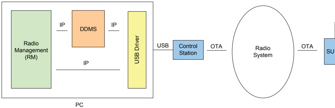
Figure 50: Single Channel Non-Remote RM Application with Presence and MNIS
