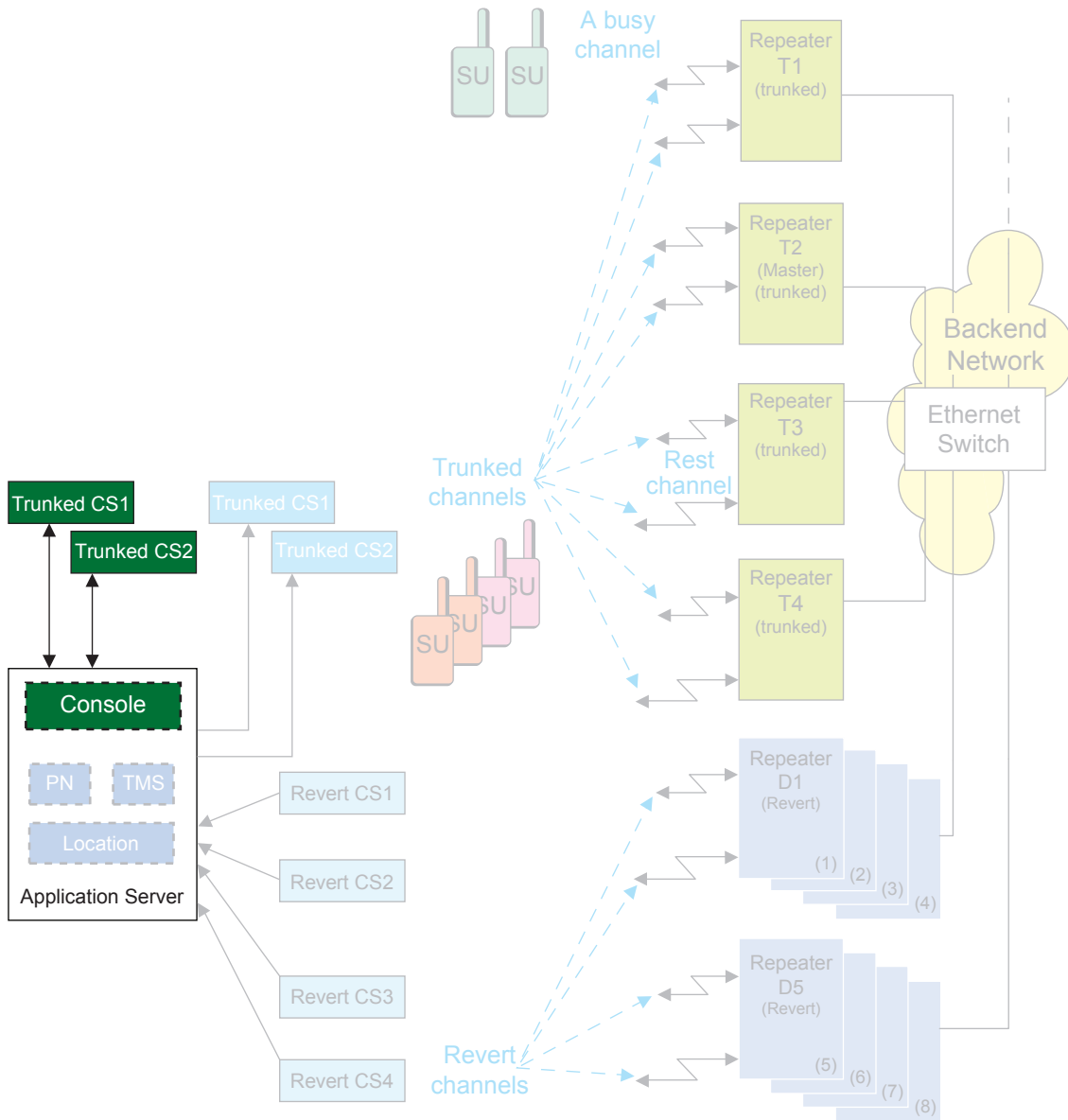
Figure 126: Capacity Plus Single Site Devices with a Dispatch Station (Console)
