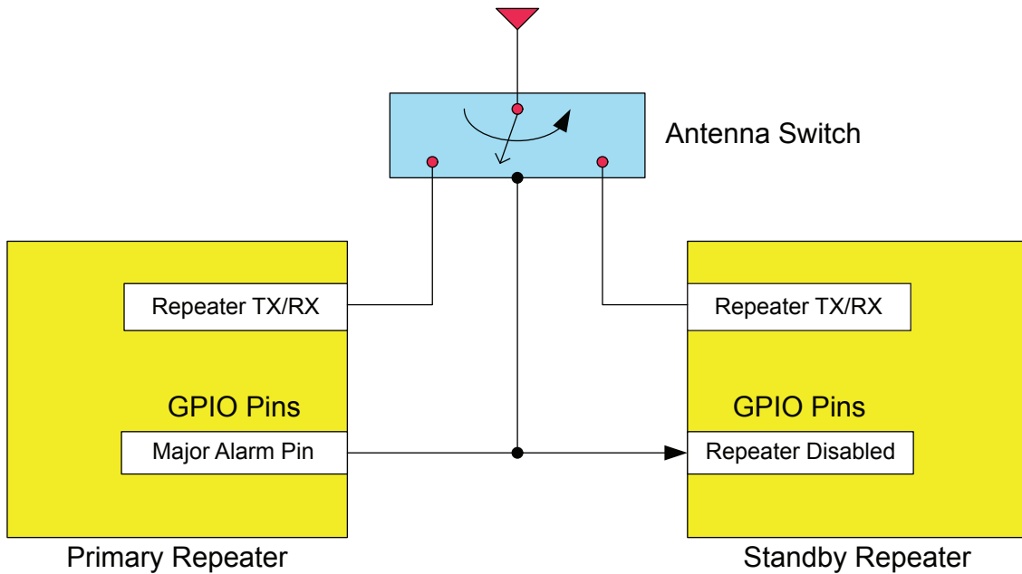
Figure 30: Redundant Repeater Setup
