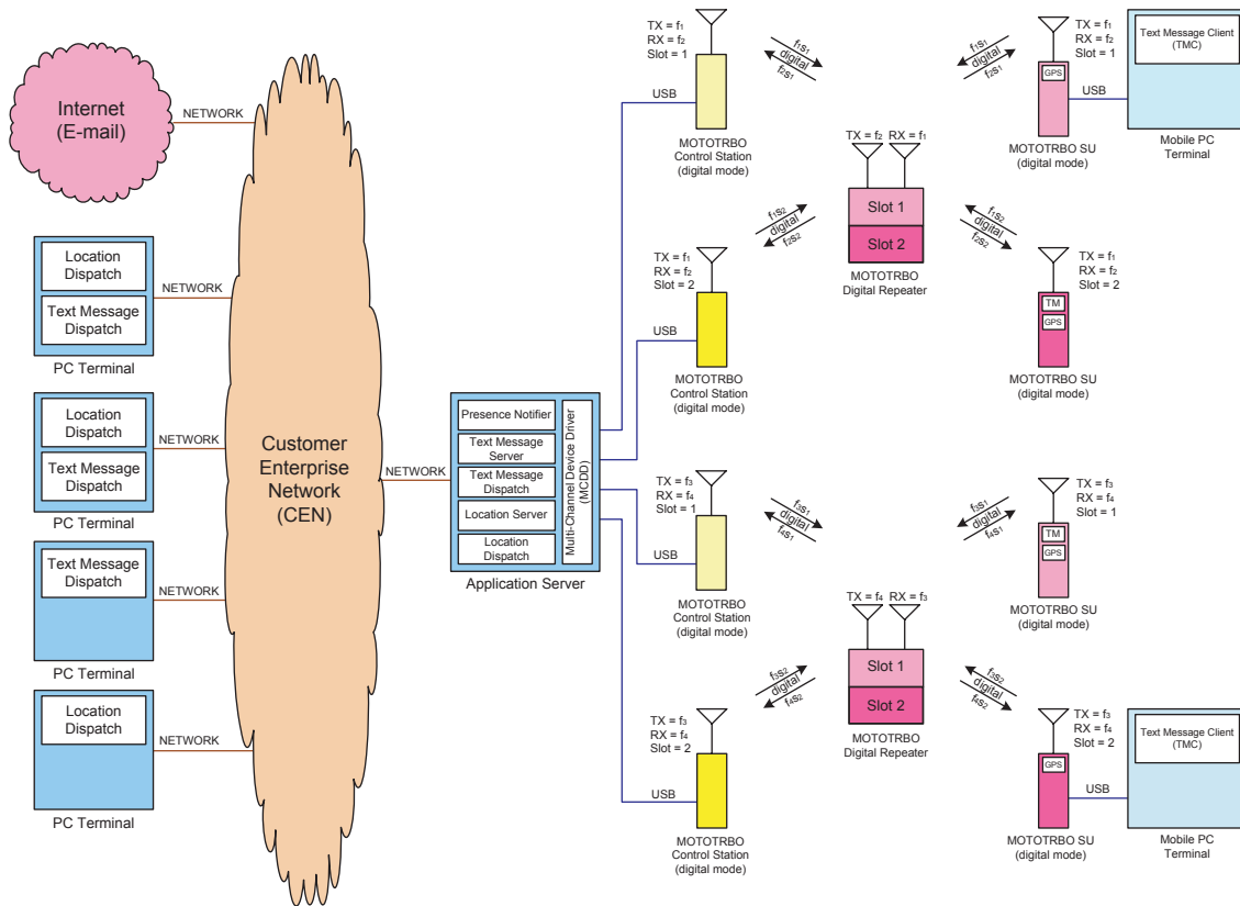
Figure 106: MOTOTRBO Radios in Digital Two-Slot, Digital Repeater Mode with Text Message Server, Location Server Using Control Stations with Local and Remote Dispatchers
