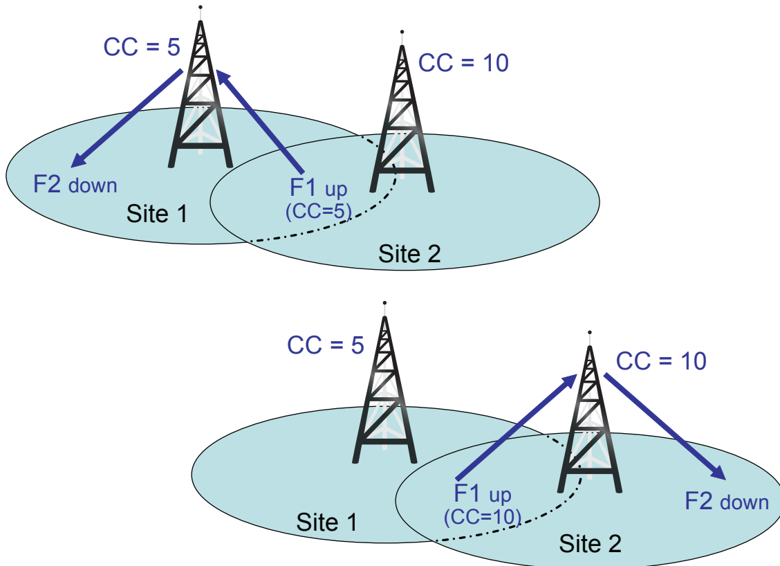
Figure 153: Multiple Digital Repeaters with Unique Color Codes
