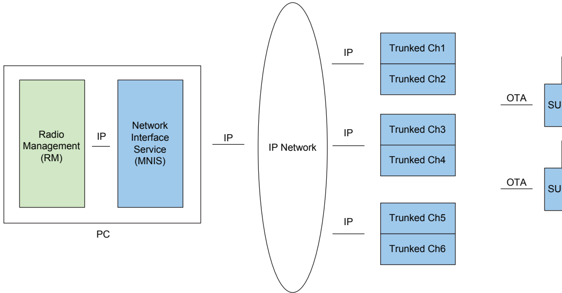
Figure 195: RM Application in a Capacity Plus System with a MNIS
