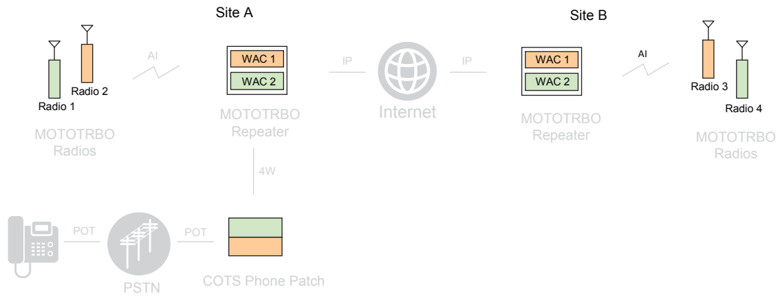
Figure 63: Two APP Boxes Supporting Two Wide Area Channels in IP Site Connect
