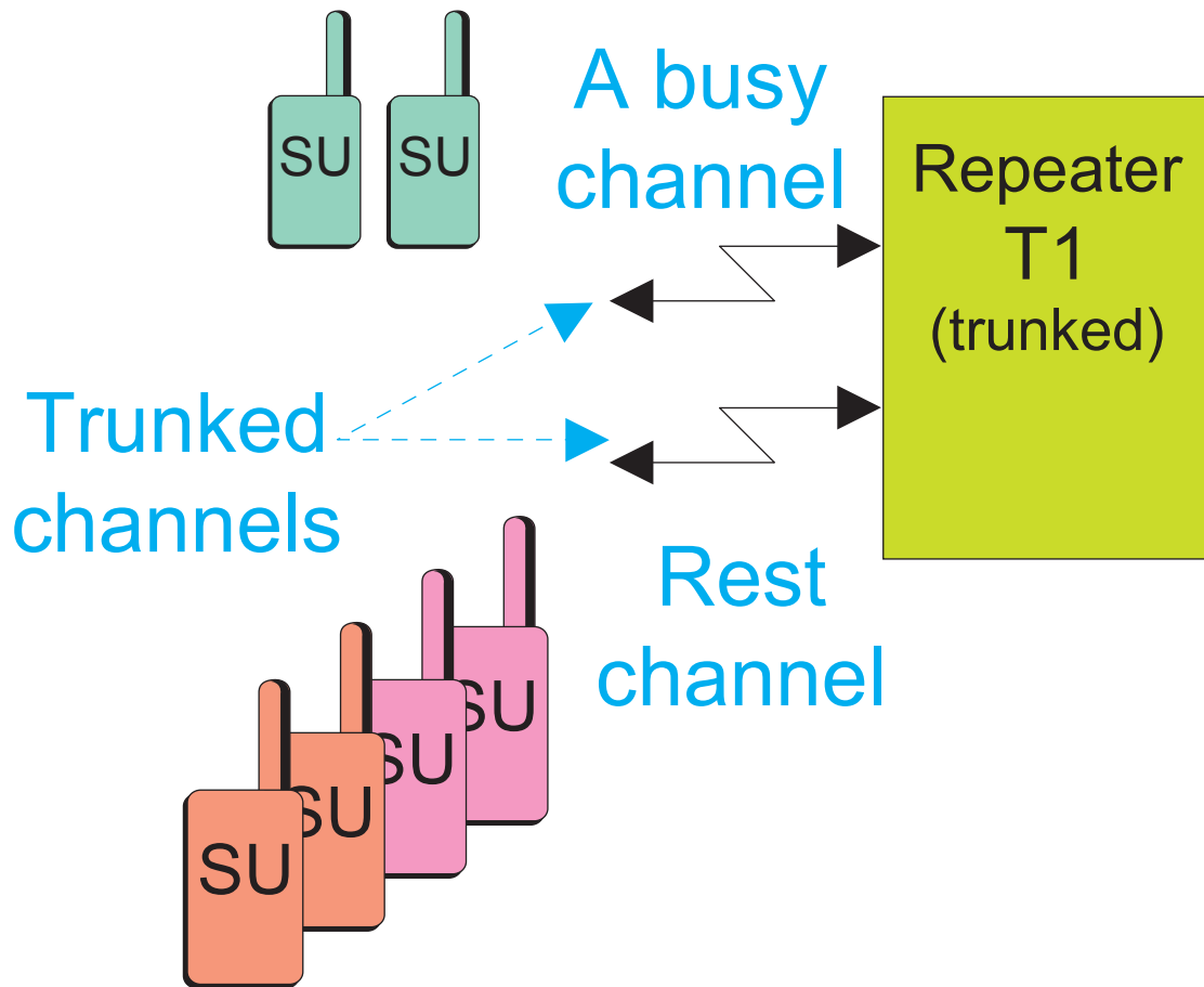
Figure 121: Two-Channel Capacity Plus Single Site System without Data Application Server
