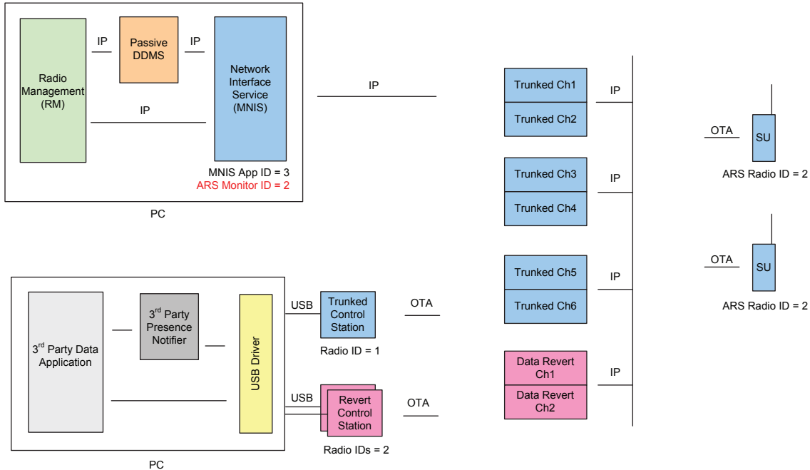
Figure 203: RM Application with MNIS and Passive Presence Configuration with Third-Party Data Application on a Capacity Plus Single Site Data Revert Configuration
