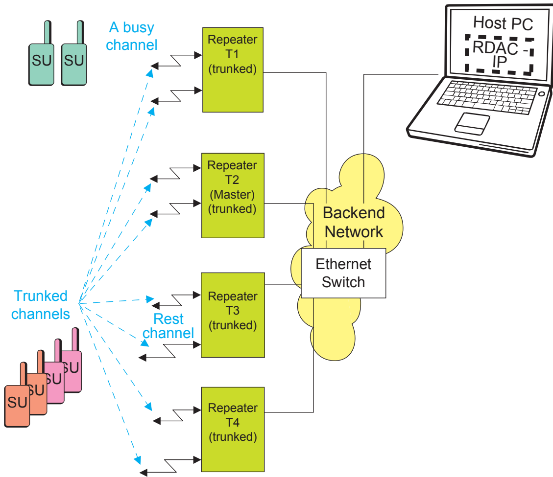
Figure 120: Capacity Plus Single Site Devices with Local RDAC and no Data Application Server
