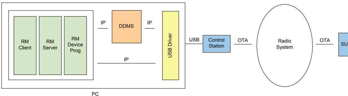
Figure 51: Single Channel Non-Remote RM Application with Presence
