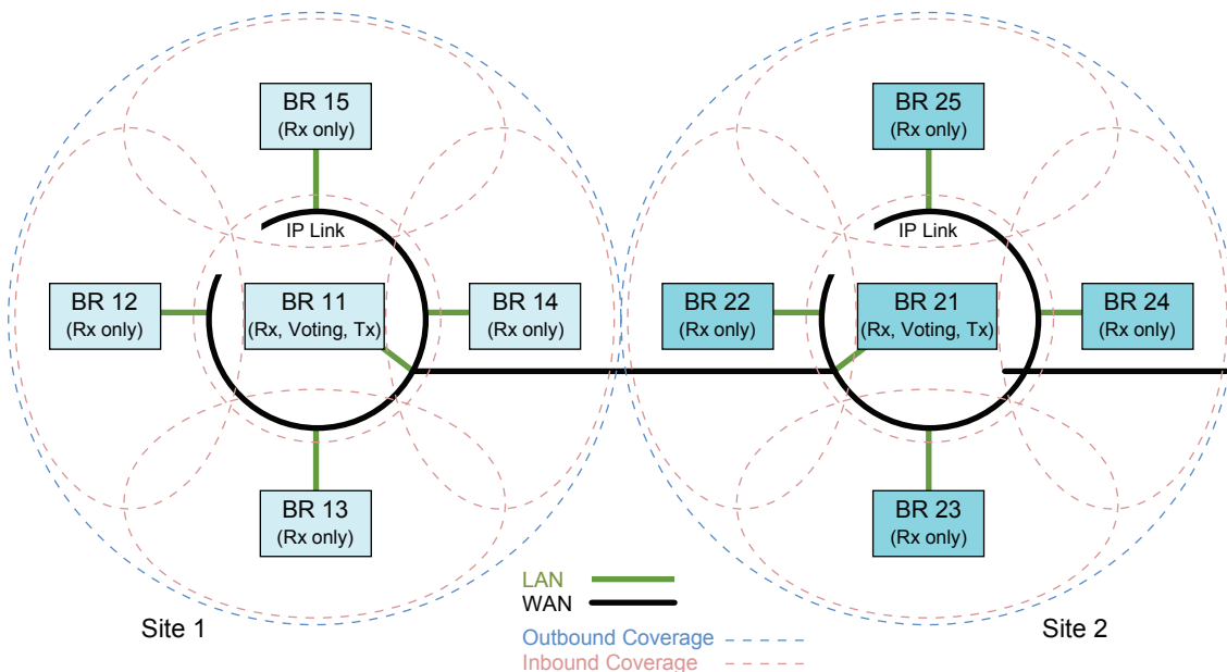
Figure 131: Digital Voting Topology for a Two-Site IP Site Connect System
