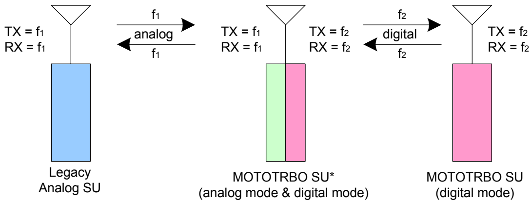
Figure 96: Legacy Analog and MOTOTRBO Analog and Digital Radios in Direct Mode
