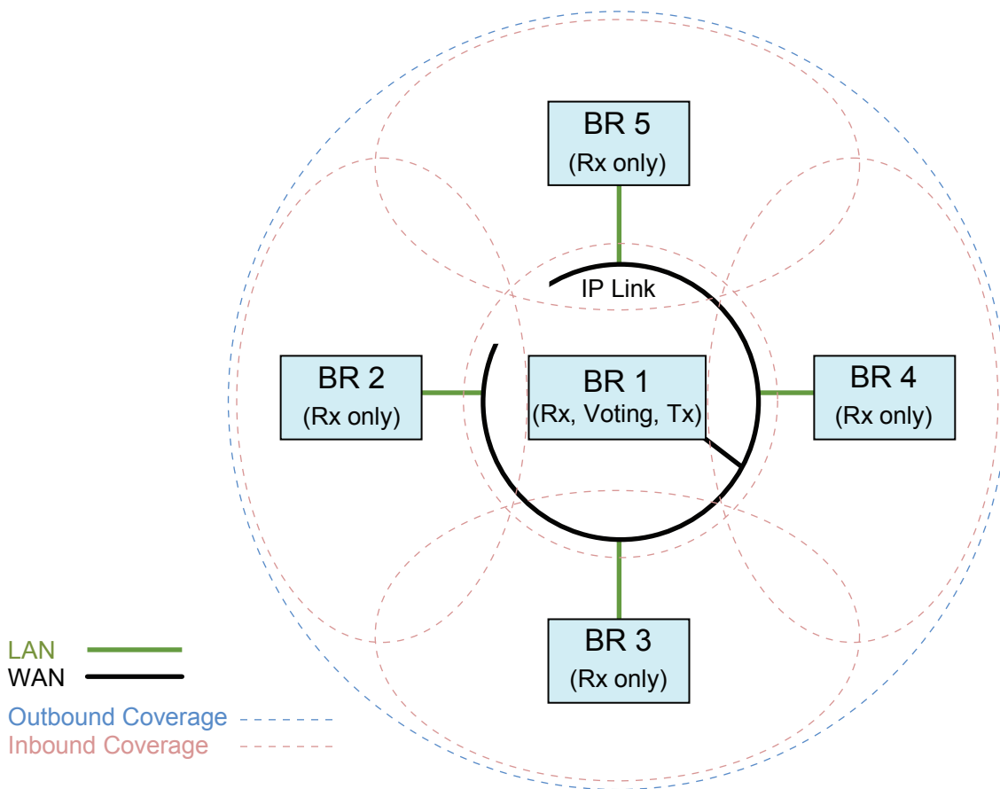
Figure 130: Digital Voting Topology for Conventional Single Site or IP Site Connect Local Channel
