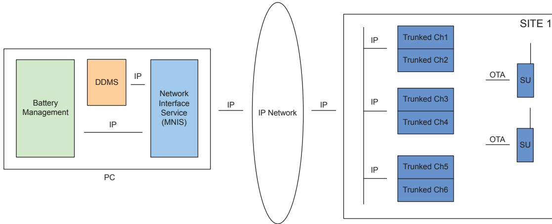
Figure 34: BMA Deployment in Capacity Plus Single Site with MNIS
