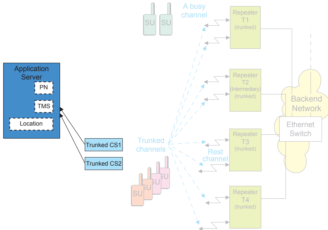
Figure 123: Capacity Plus Single Site Devices with Data over Trunked Channels
