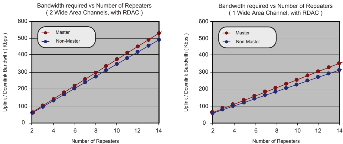
Figure 156: Required Bandwidth for Two Simple IP Site Connect System Configurations
