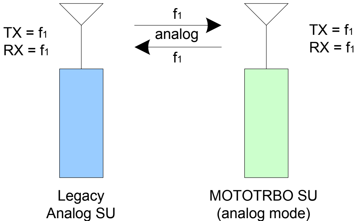
Figure 95: Legacy Analog Radios and MOTOTRBO Radios (in analog mode) in Direct Mode
