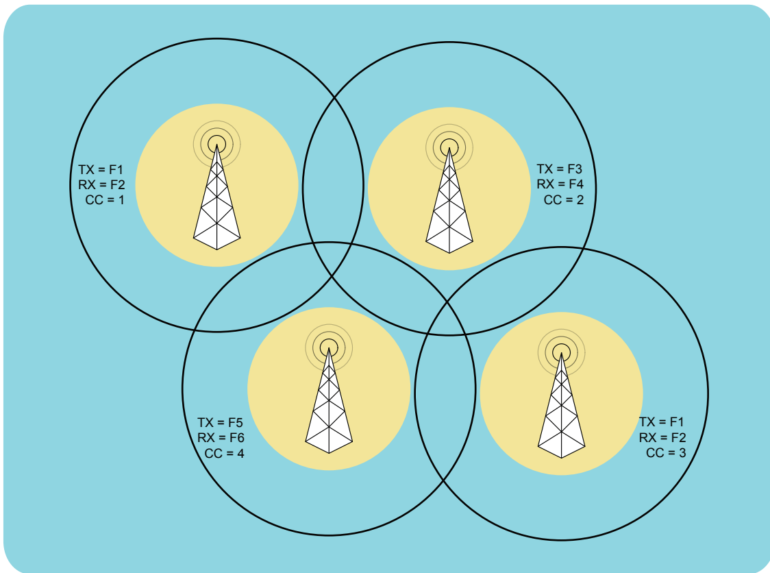
Figure 24: Dense Overlapping Coverage (Urban)
