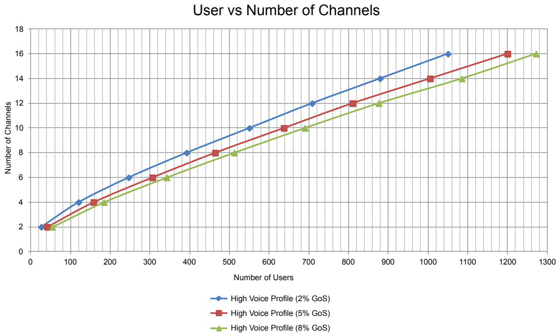
Figure 137: Number of Users Versus Number of Channels for Voice-Only Profile
