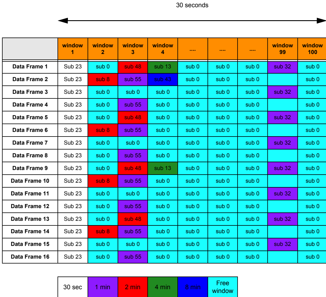
Figure 13: Subscriber Scheduling in a Window Map with 30 Seconds Data Frame
