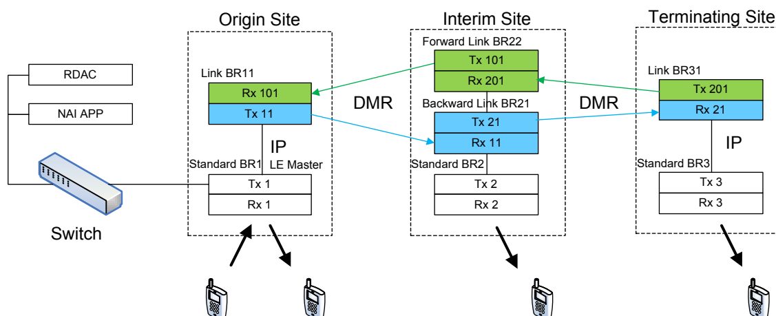
Figure 134: Dedicated Standalone MOTOTRBO Link System
