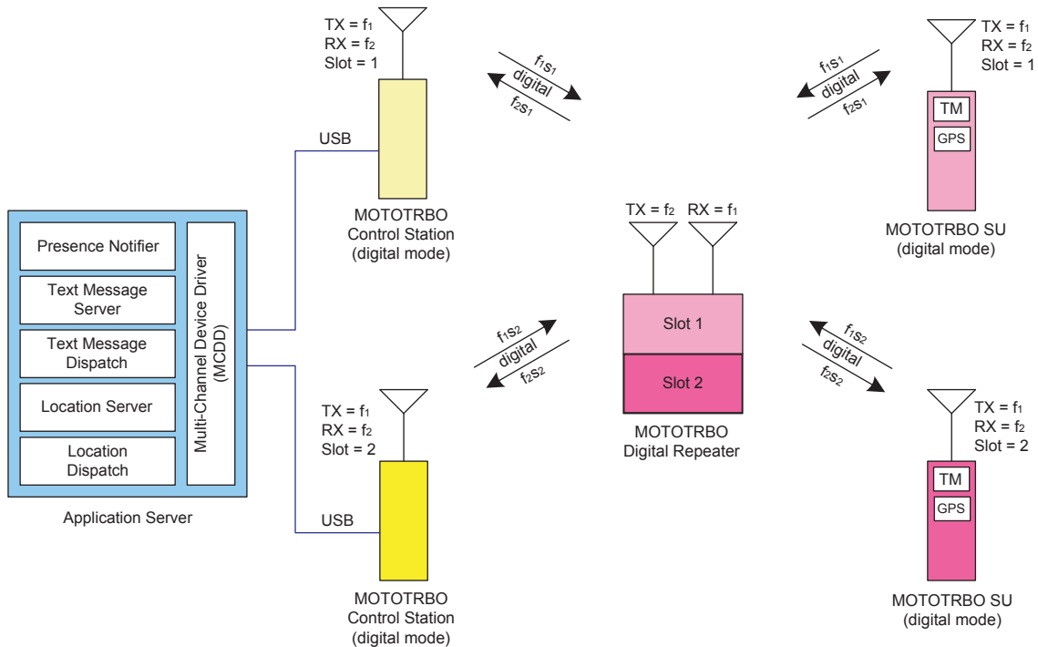
Figure 104: MOTOTRBO Radios in Digital Two-Slot Digital Repeater Mode with a Server-Based Configuration Using Control Stations
