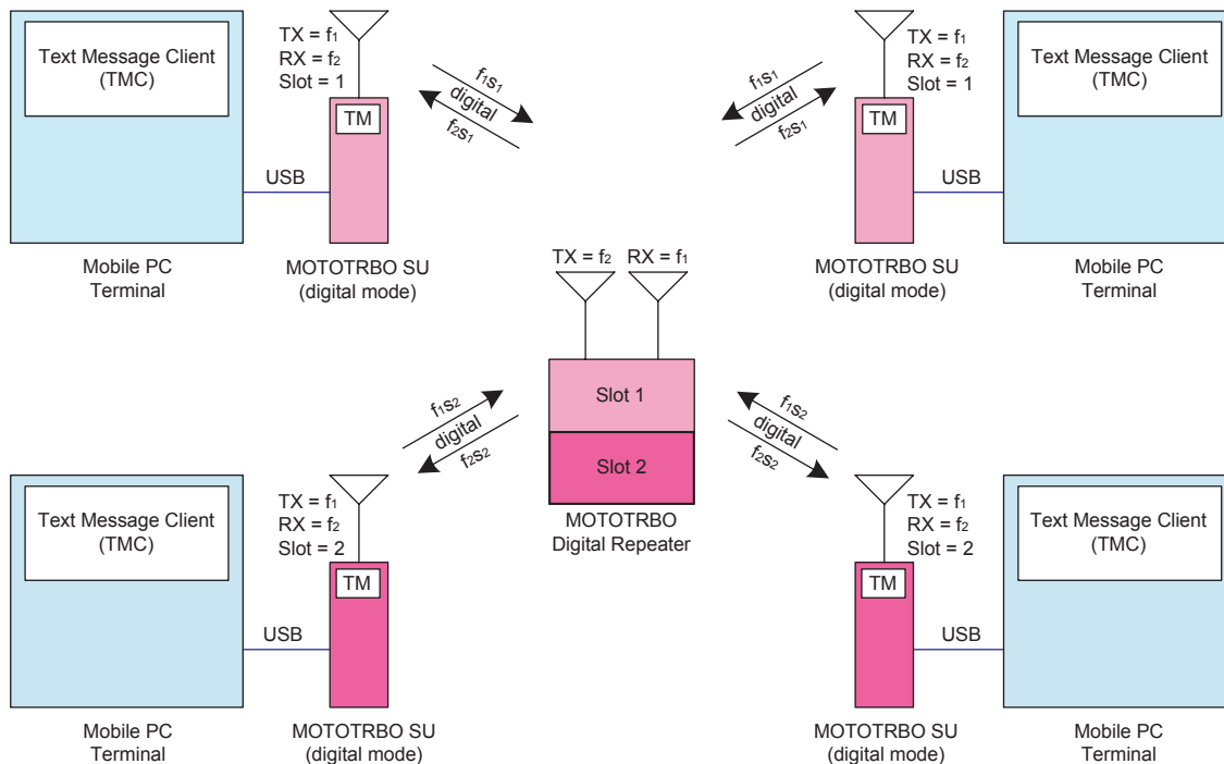
Figure 102: MOTOTRBO Radios in Digital Two-Slot Digital Repeater Mode with Text Messaging
