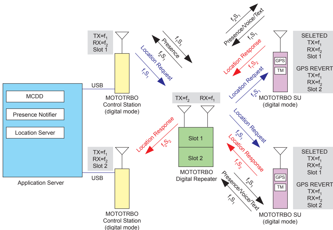
Figure 107: MOTOTRBO Radios in Two-Slot Digital Repeater Mode with GPS Revert Configuration
