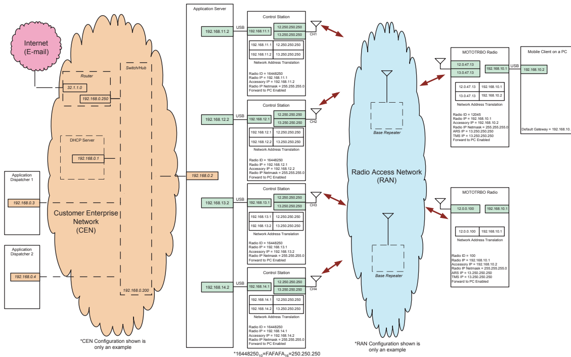
Figure 164: Example MOTOTRBO System IP Plan
