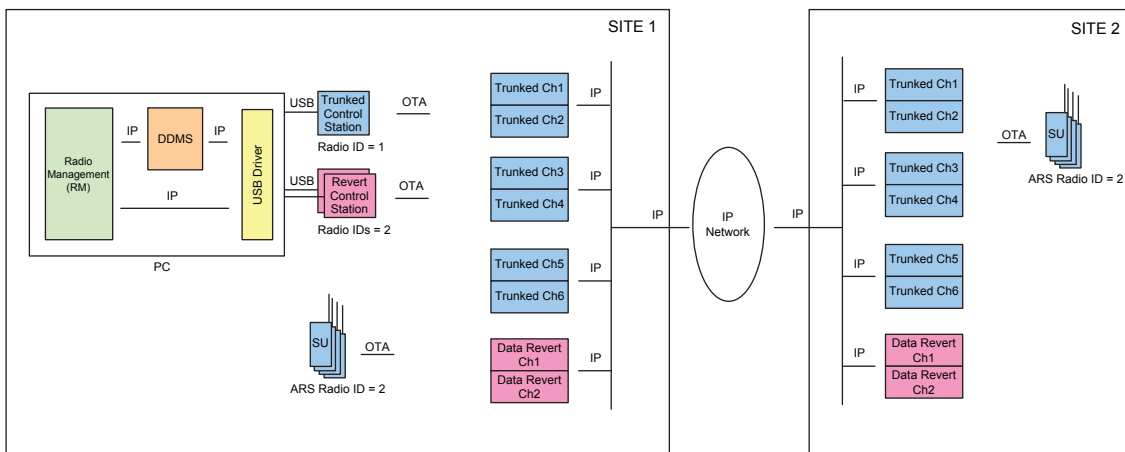
Figure 198: RM Application with Control Stations in a Capacity Plus Multi Site System with Presence (DDMS) and Wide Area Data Revert Channels
