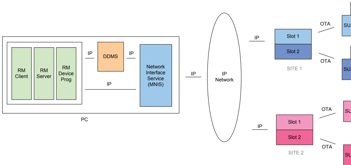
Figure 187: RM Application with MNIS Covering RF Isolated Single Site Repeaters
