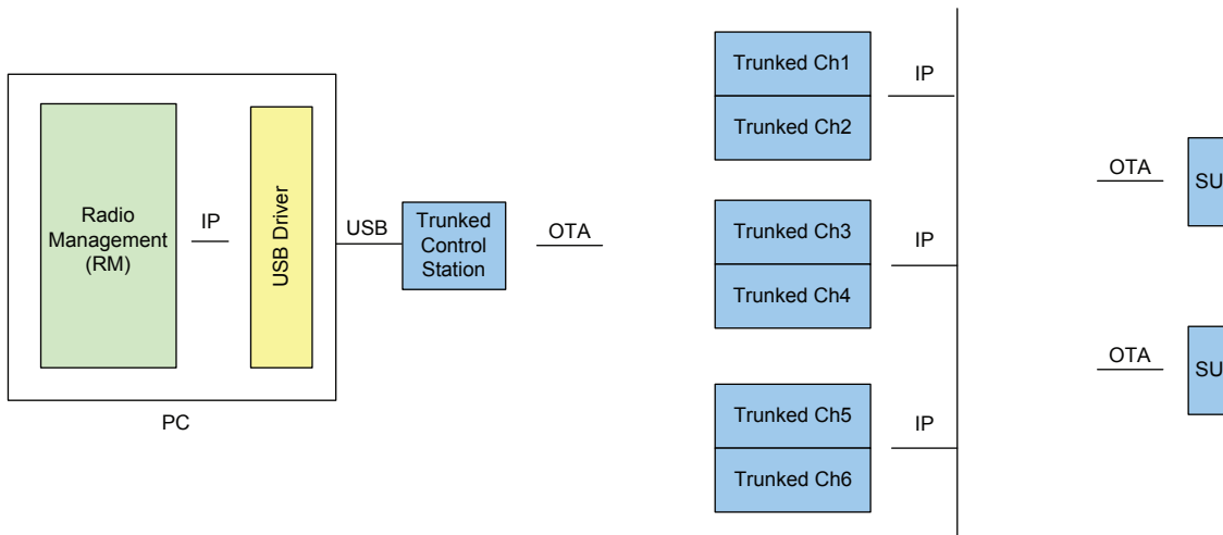
Figure 191: RM Application in a Capacity Plus System with No DDMS and One Trunked Control Station
