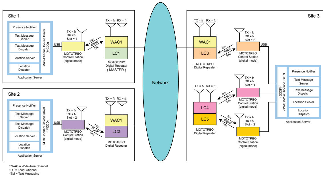
Figure 115: Wide and Local Area System with Distributed Data Application Servers
