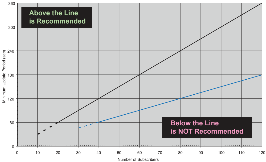
Figure 144: Minimum Location Update Period versus Number of Subscribers
