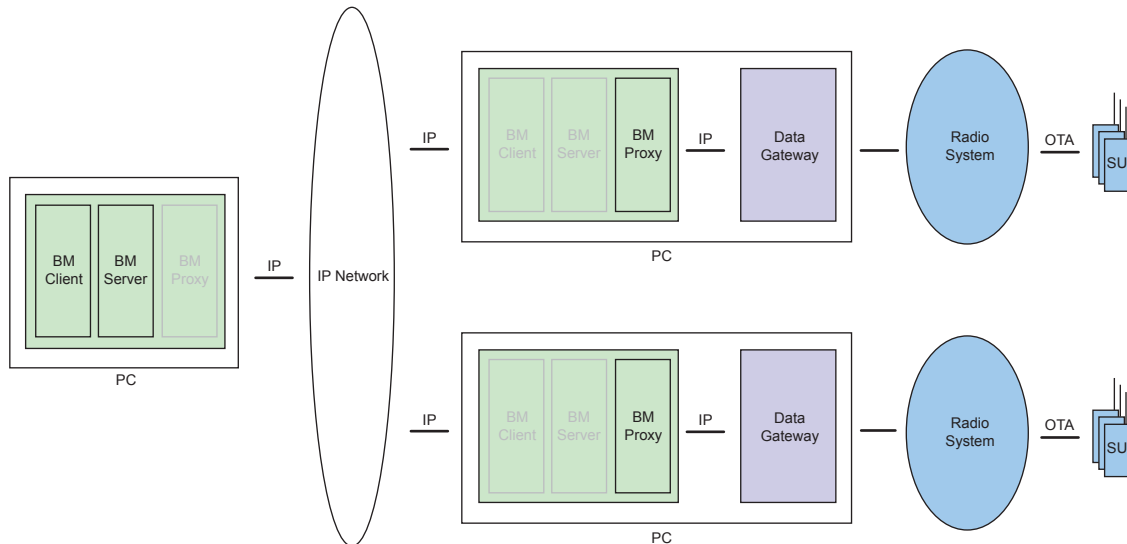
Figure 46: BMA Deployment with Multiple Proxies Remote from Server
