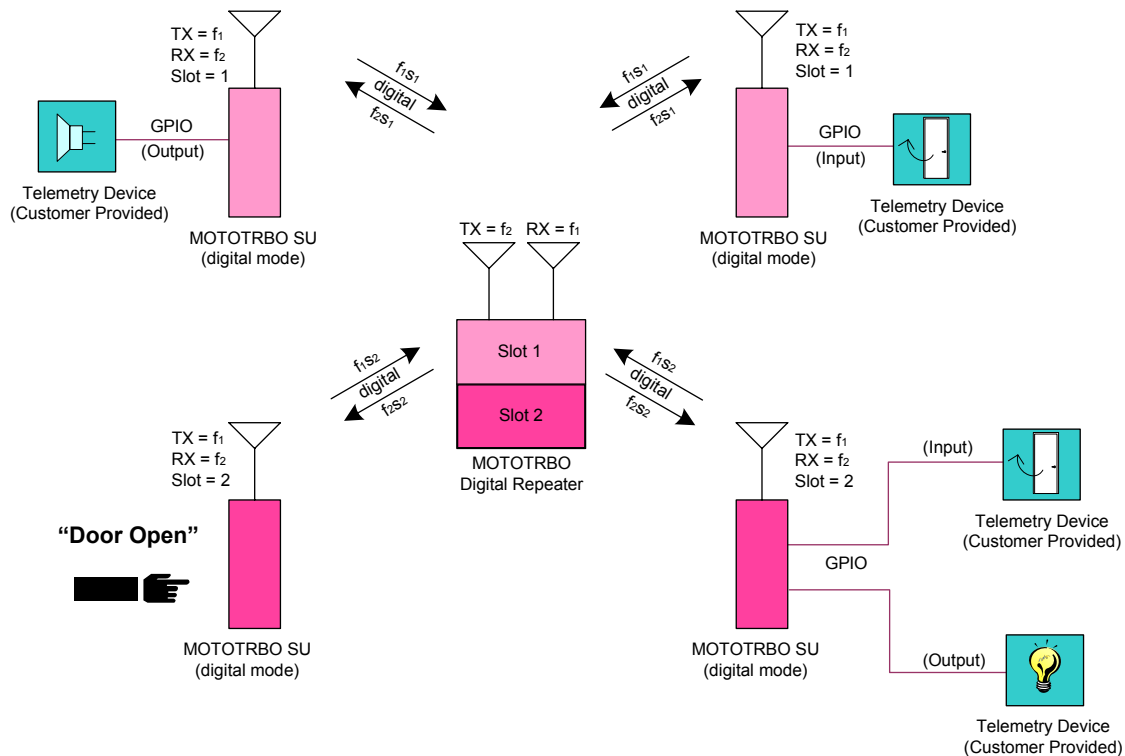
Figure 103: MOTOTRBO Radios in Digital Two-Slot Digital Repeater Mode with Telemetry Functions
