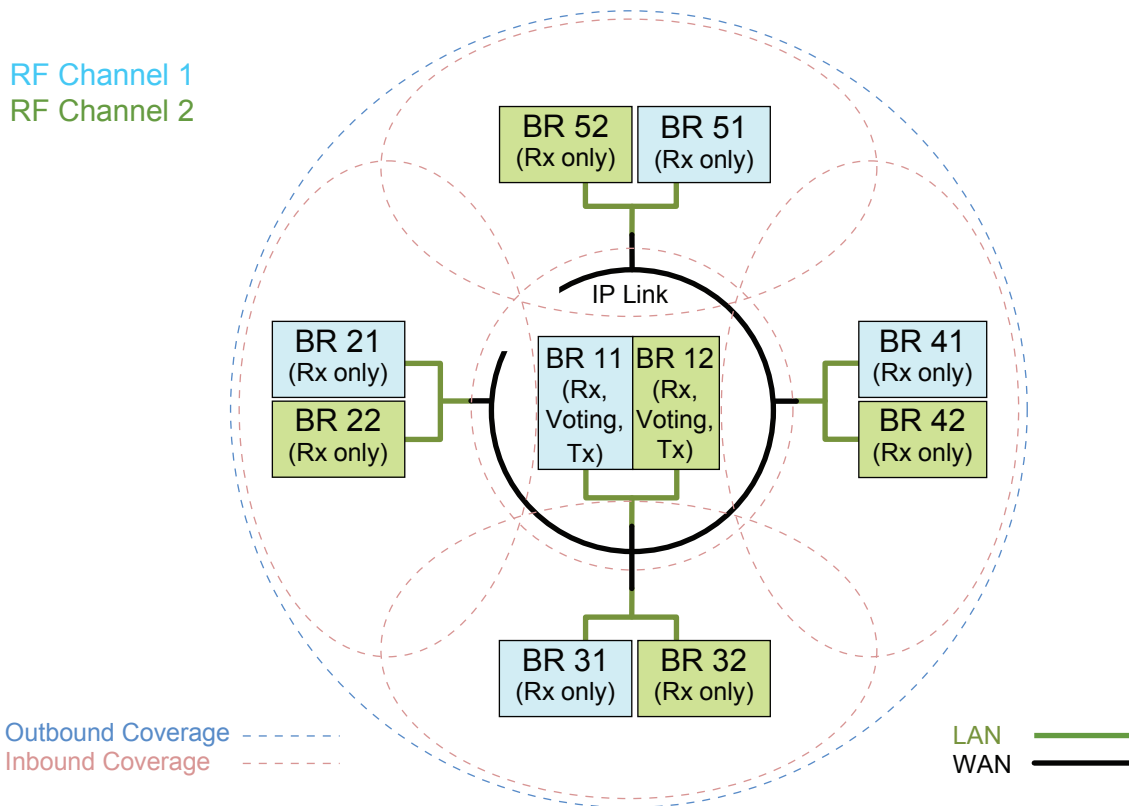
Figure 132: Digital Voting Topology for a Capacity Plus Single Site System
