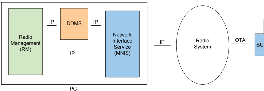
Figure 50: Single Channel Non-Remote RM Application with Presence and MNIS
