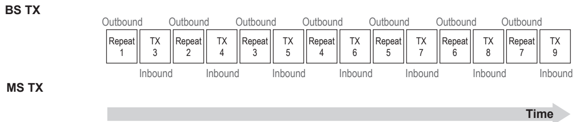
Figure 99: Time Division Duplex Repeater
