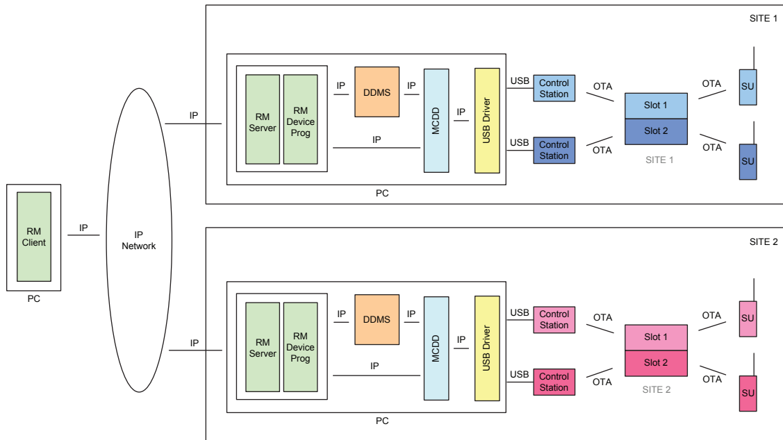
Figure 185: RM Application with Control Stations Covering RF Isolated Single Site Repeaters
