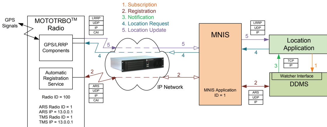
Figure 167: Location Application with MNIS and DDMS in a Single Site Digital System
