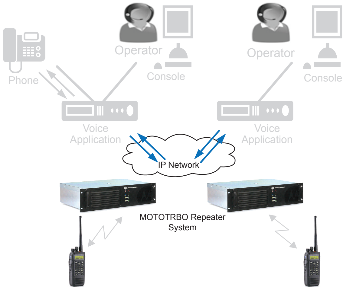
Figure 66: Wireline Telephony with Third-party Telephony Application
