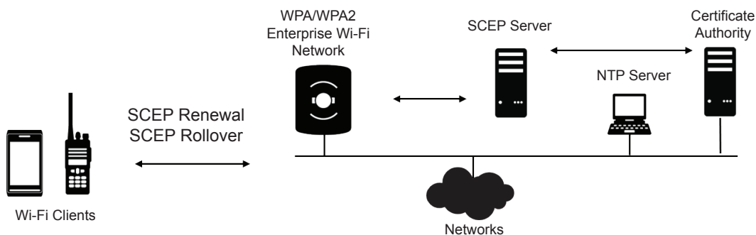
Figure 68: Certificate Renewal and Rollover
