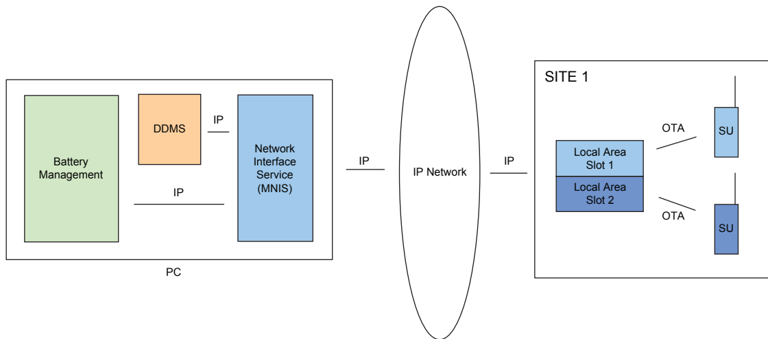
Figure 32: BMA Deployment in Single Site with MNIS
