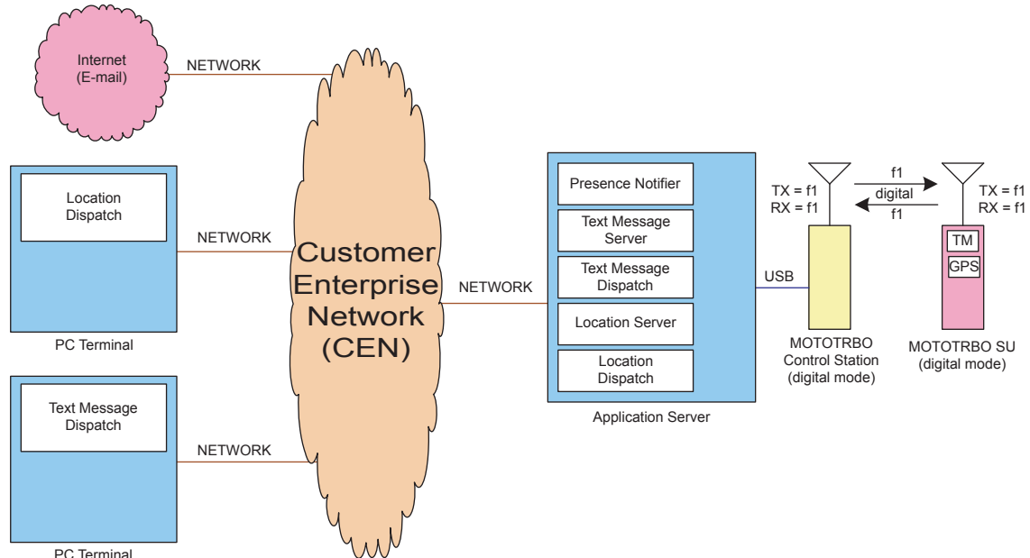
Figure 92: MOTOTRBO Radios In Digital Direct Mode/Dual Capacity Direct Mode Server Based Configuration with Remote Dispatchers
