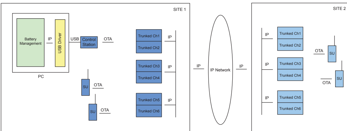
Figure 41: BMA Deployment in Capacity Plus Multi Site with a Control Station
