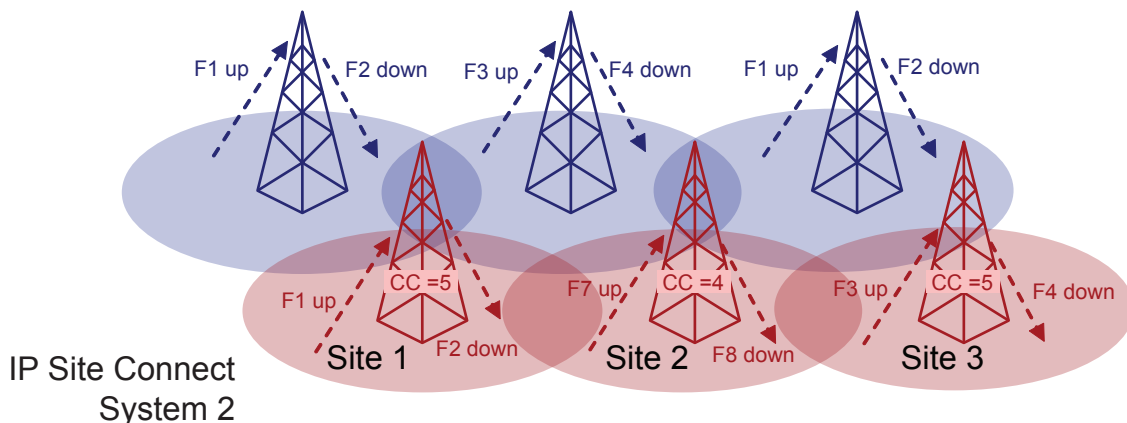
Figure 155: Example of Two IP Site Connect Systems with Overlapping Coverage Areas
