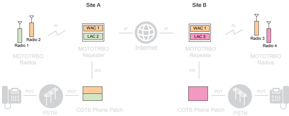
Figure 64: APP Boxes Supporting Wide Area Channels and Local Area Channels in IP Site Connect
