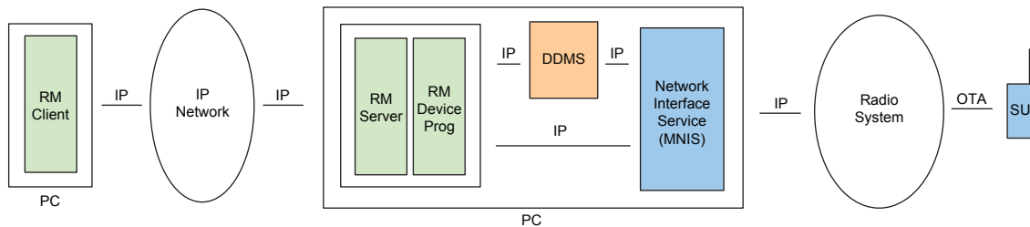
Figure 53: Remote RM Client from RM Server with MNIS
