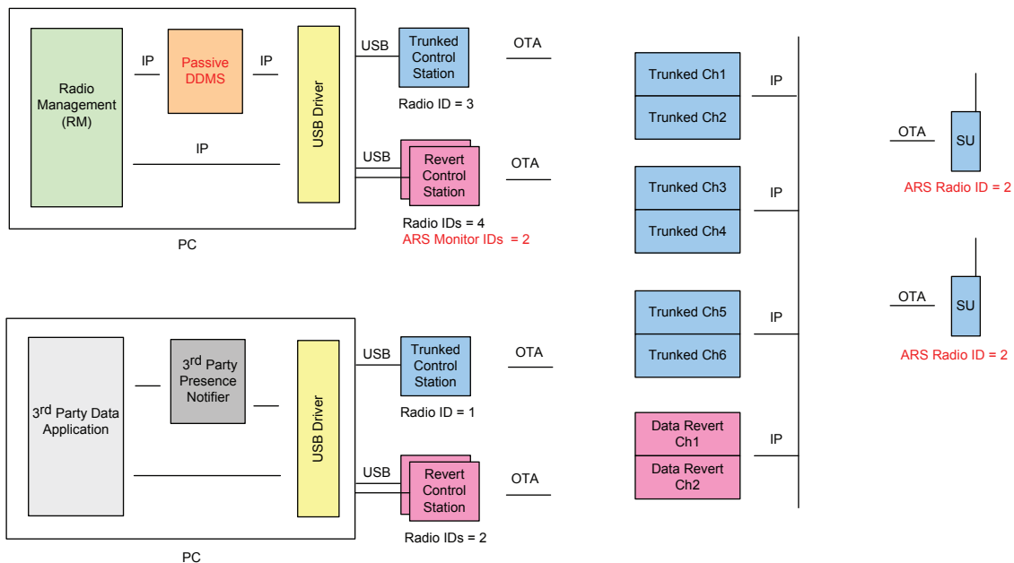
Figure 202: RM Application with Control Stations and Passive Presence Configuration with Third-Party Data Application on a Capacity Plus Single Site Data Revert Configuration
