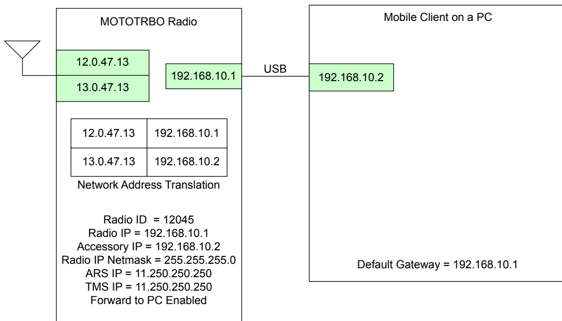
Figure 162: Air Interface Network Connectivity
