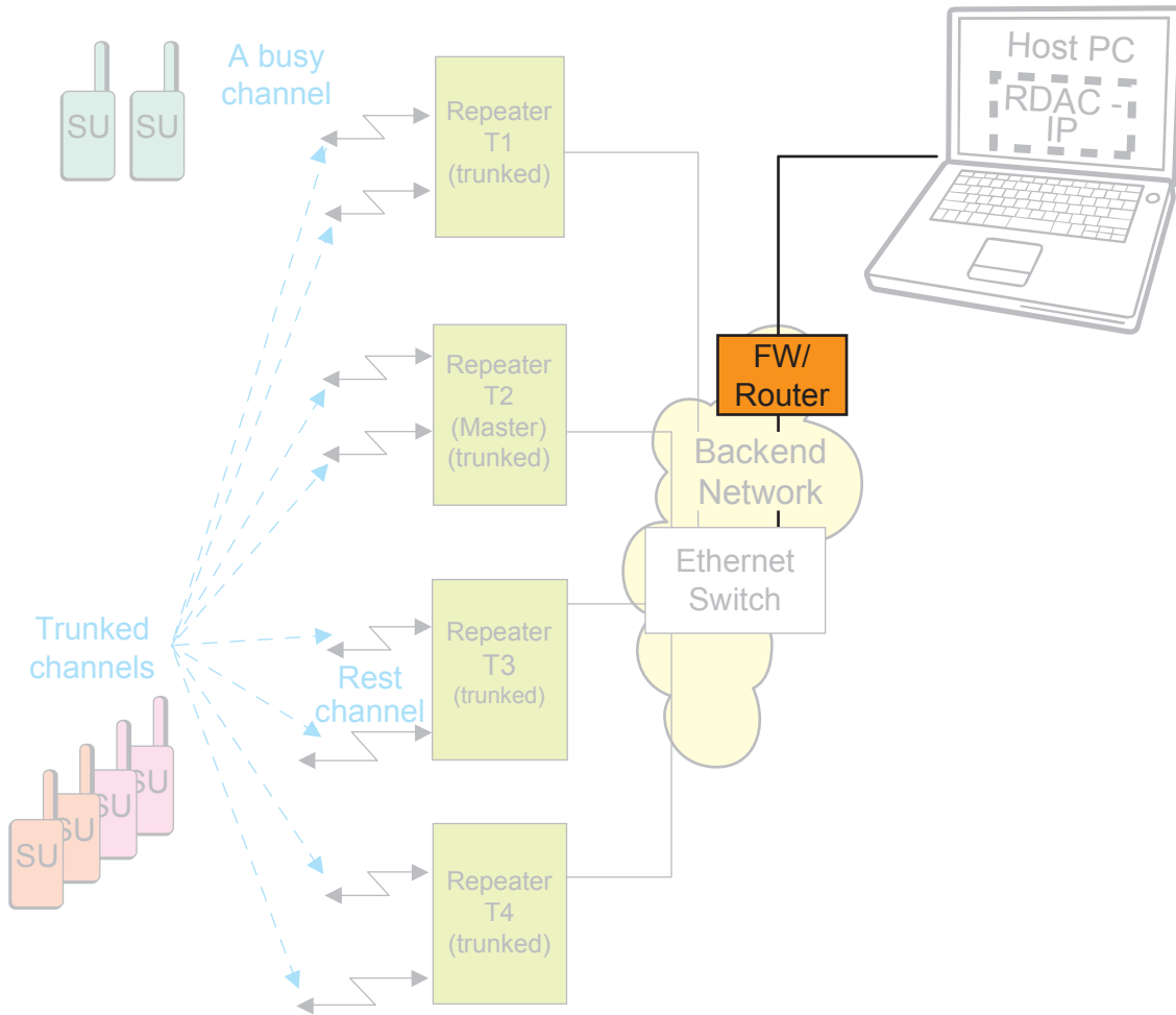
Figure 122: Capacity Plus Single Site Devices with Remote RDAC and no Data Application Server
