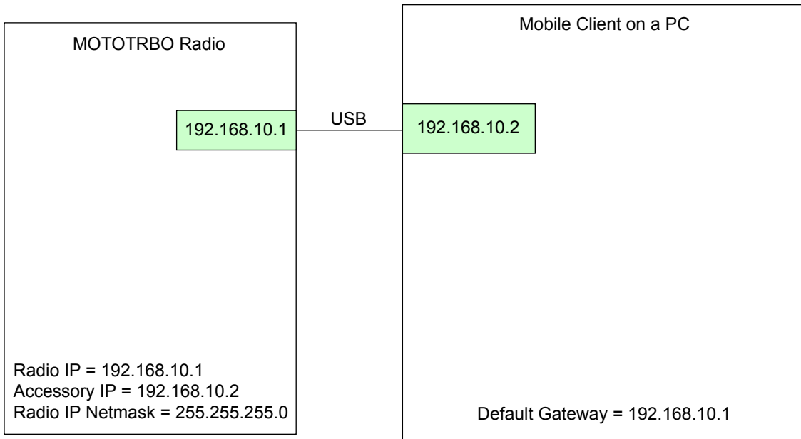
Figure 161: Connectivity between the Mobile Client and the MOTOTRBO Radio
