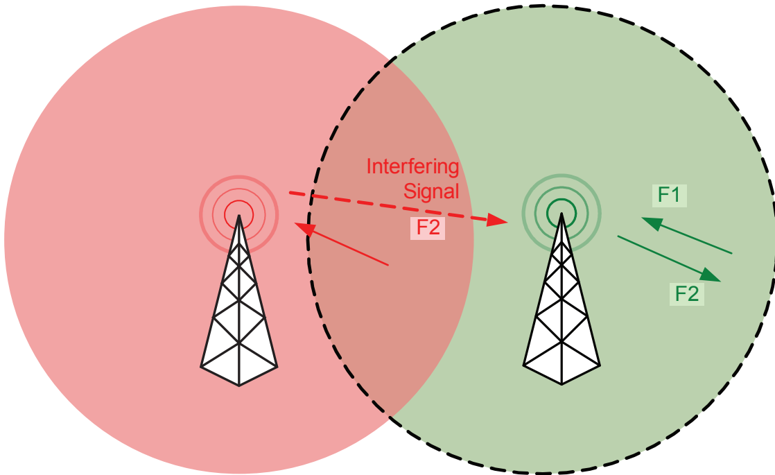
Figure 160: An Example of Interference at Transmit Frequency
