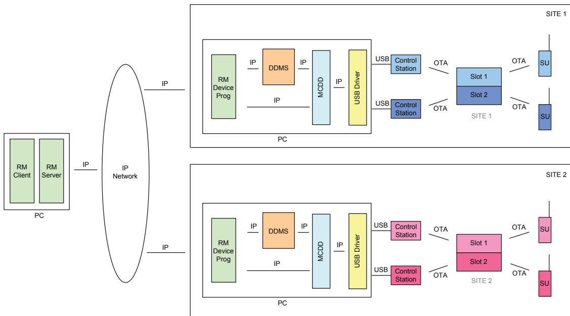
Figure 186: RM Application with Control Stations Covering RF Isolated Single Site Repeaters Using Remote Device Programmers
