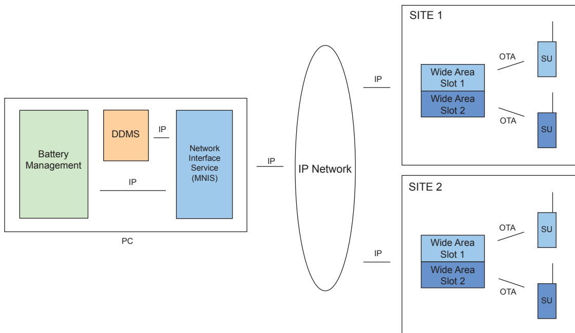
Figure 33: BMA Deployment in IP Site Connect with MNIS
