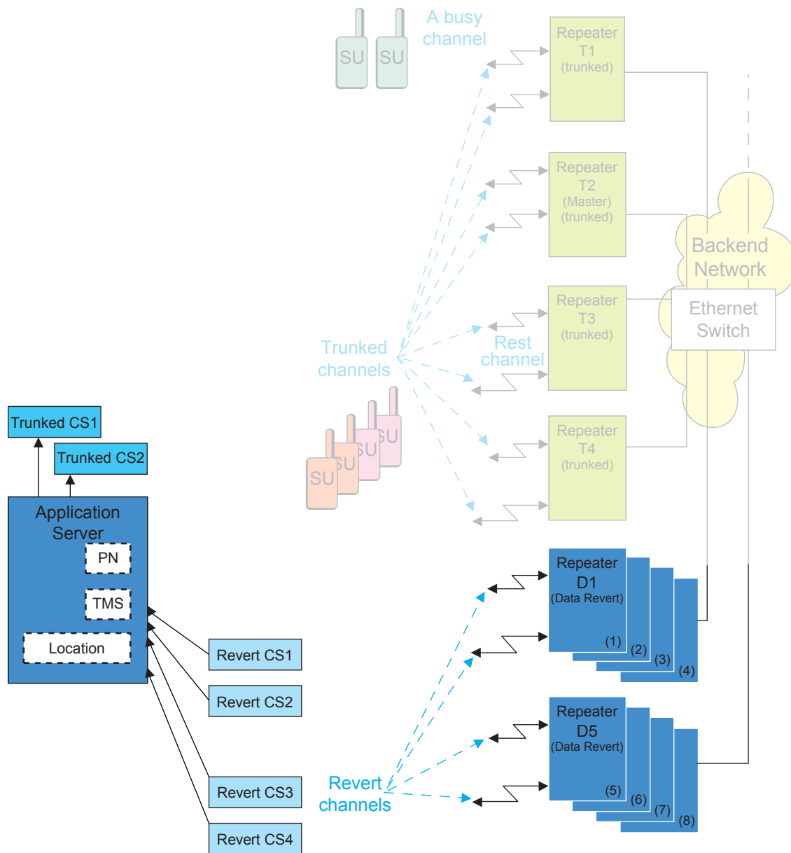
Figure 125: Capacity Plus Single Site Devices with Data over Revert Channels
