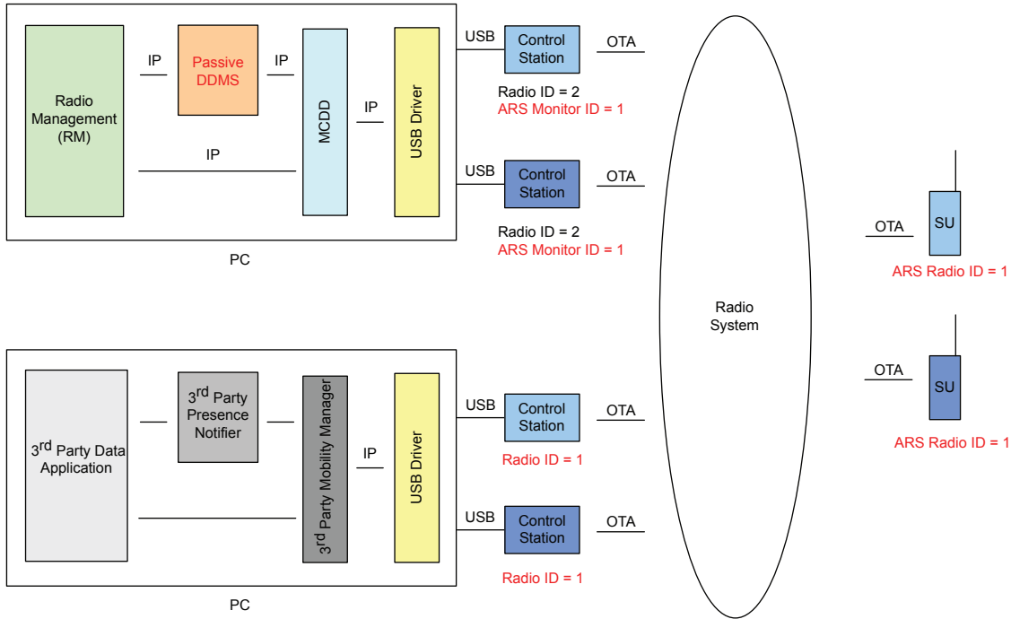
Figure 201: RM Application with Control Stations and Passive Presence Configuration with Third-Party Data Application
