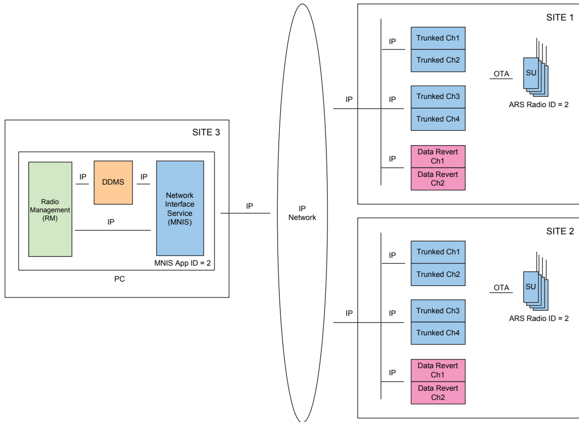
Figure 200: RM Application with MNIS in a Capacity Plus Multi Site System with Presence and Wide or Local Area Data Revert Channels
