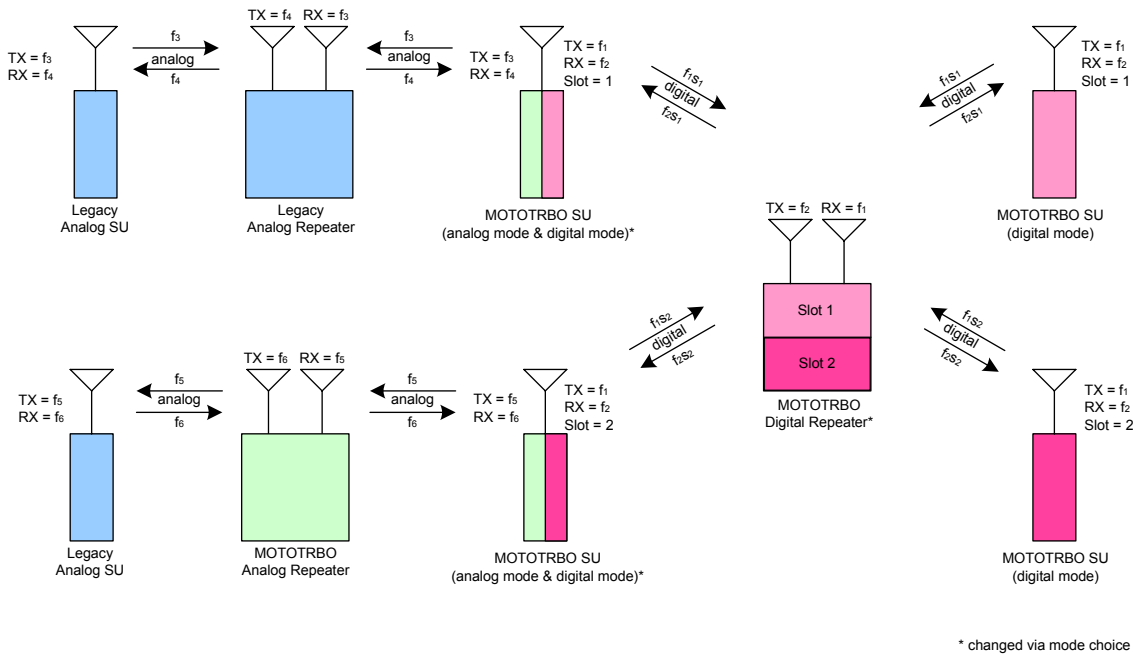
Figure 113: MOTOTRBO Digital Radios on a Two-Slot MOTOTRBO Digital Repeater with Analog Legacy Repeater Support
