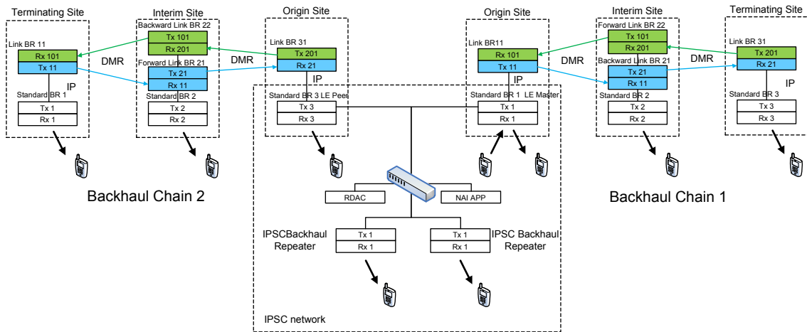
Figure 135: Dedicated Hybrid MOTOTRBO Link System
