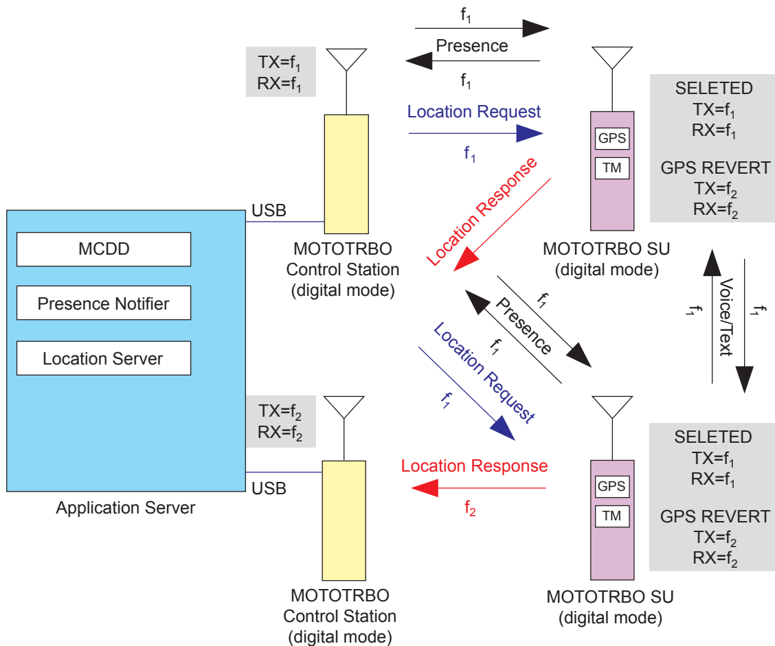
Figure 94: MOTOTRBO Radios in Two Channel Direct Mode GPS Revert Configuration
