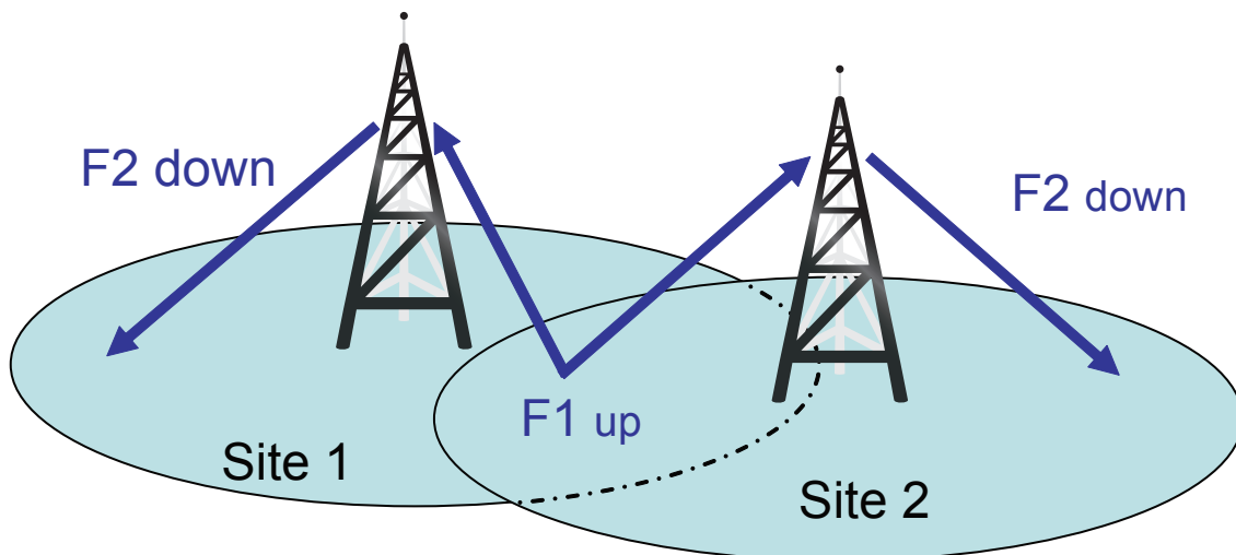
Figure 152: Multiple Repeaters with Overlap and Common Frequencies
