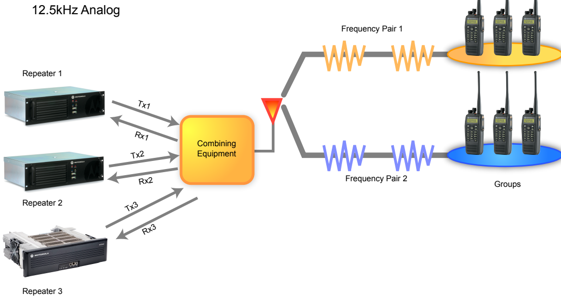
Figure 5: MOTOTRBO 2-Channel System
