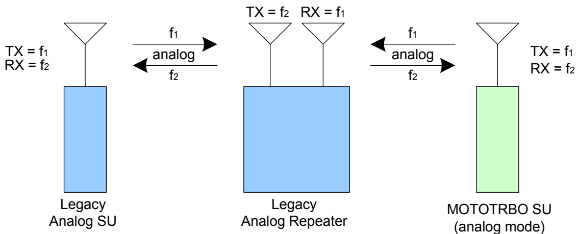
Figure 111: MOTOTRBO Analog and Legacy Analog Radios on Legacy Analog Repeater
