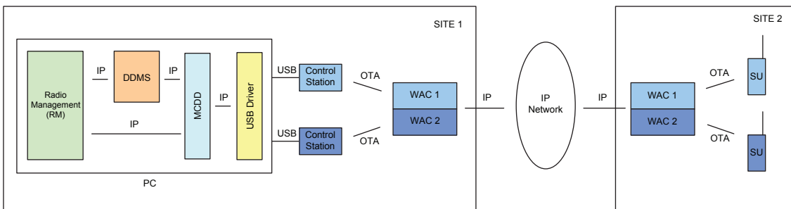
Figure 183: Multi-Channel RM Application with Control Stations in IP Site Connect Mode
