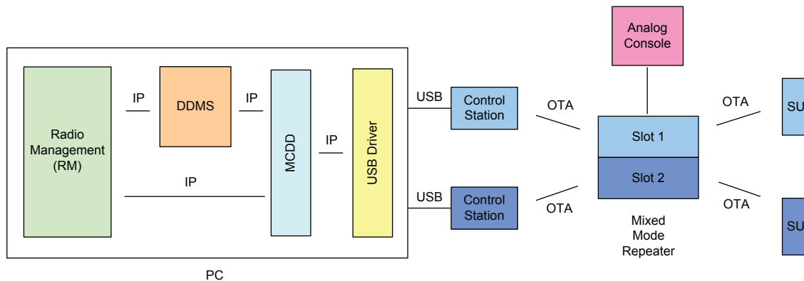
Figure 190: RM Application in Dynamic Mixed Mode
