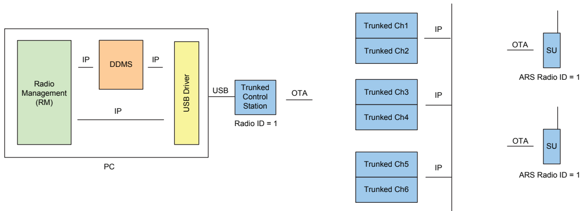
Figure 192: RM Application in a Capacity Plus System with a DDMS and One Trunked Control Station
