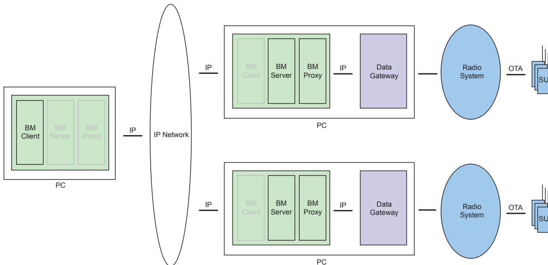
Figure 45: BMA Deployment with Client Remote from Multiple Server and Proxies
