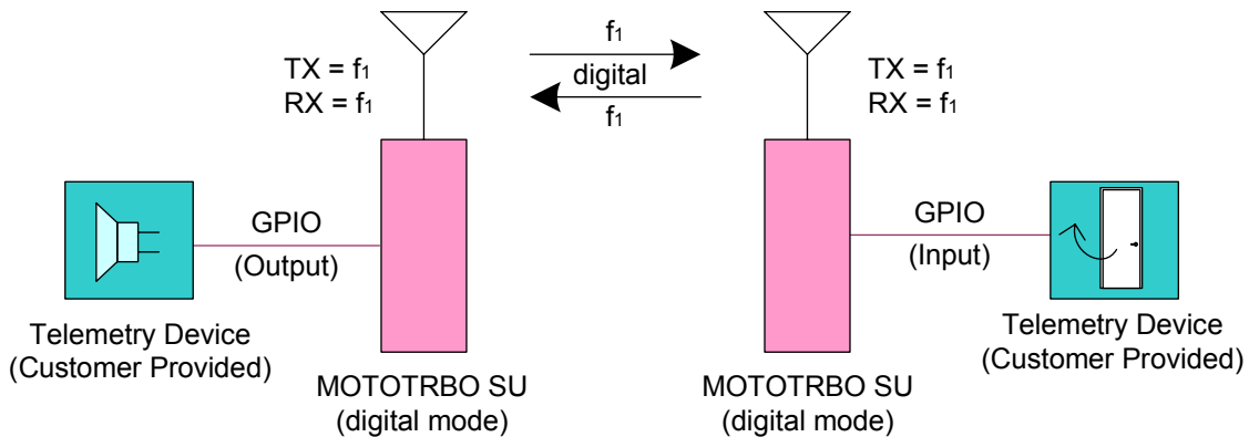
Figure 89: Send Telemetry Command to Toggle an Output Pin from MOTOTRBO Radio to Another MOTOTRBO Radio when Input Pin State Changes
