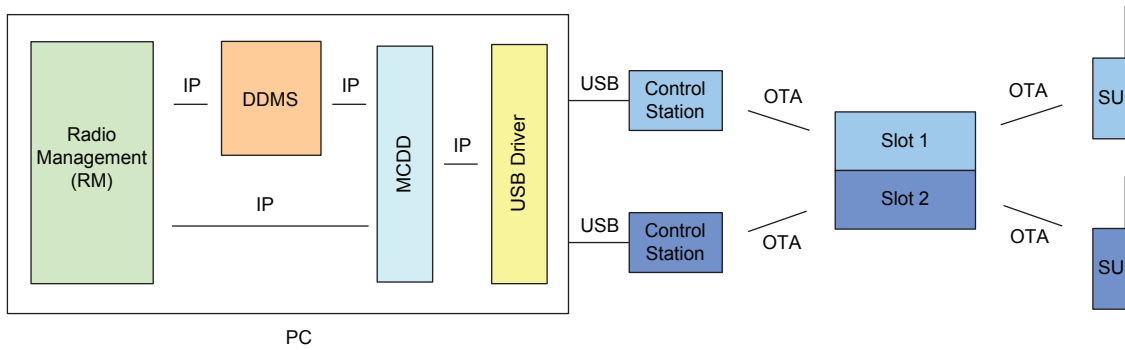
Figure 182: Multi-Channel RM Application with Control Stations in Single Site Repeater Mode
