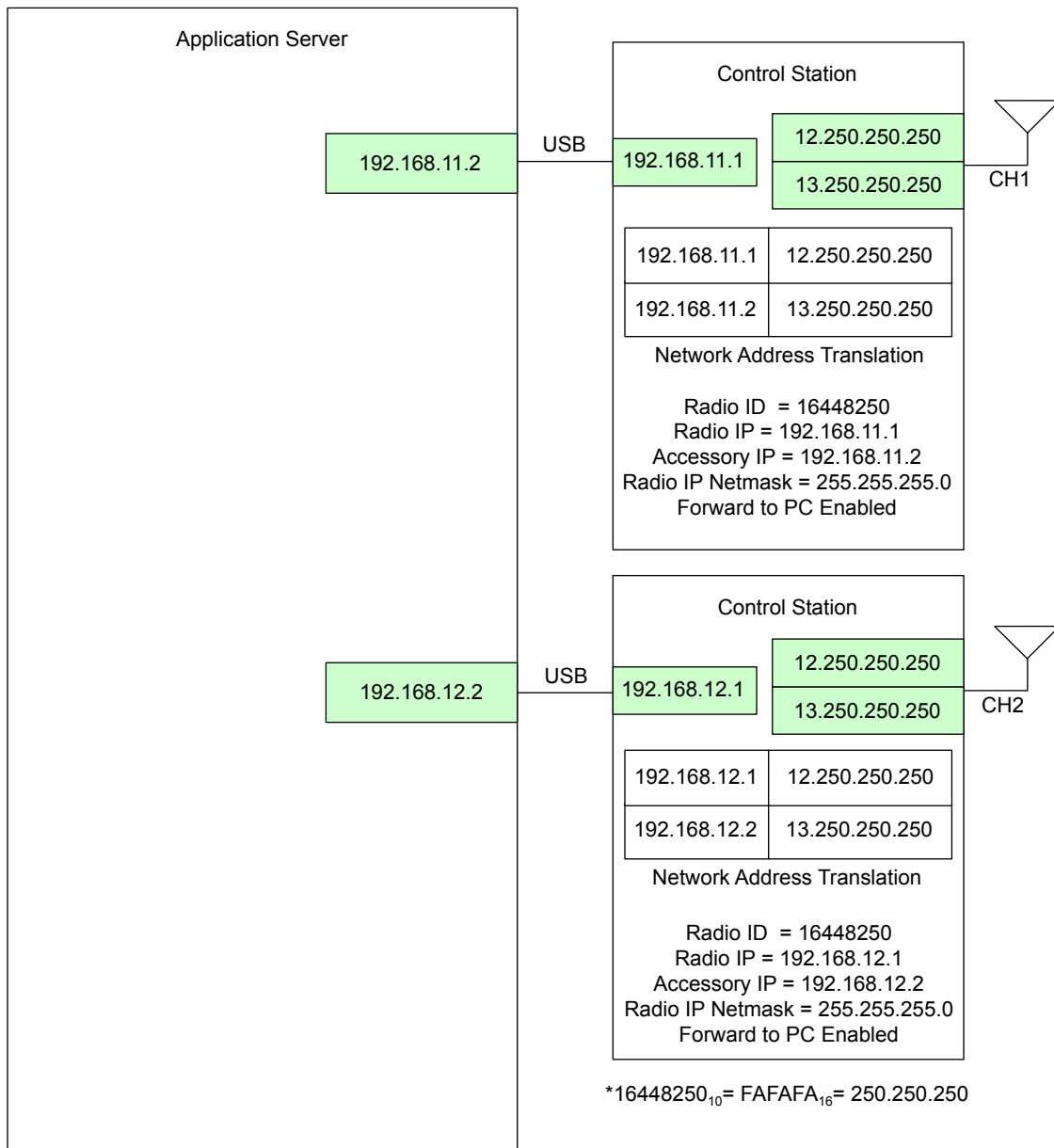
Figure 163: Application Server Control Station Network Connectivity
