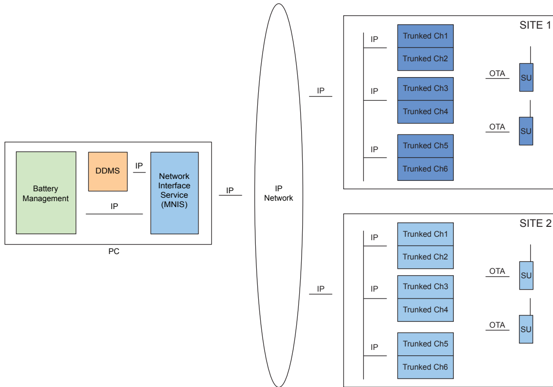
Figure 35: BMA Deployment in Capacity Plus Multi Site with MNIS
