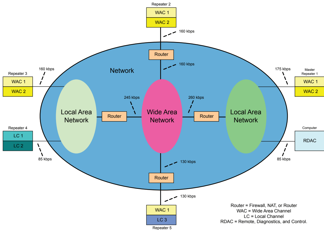
Figure 157: Example System for Calculating Bandwidth Requirements without Secure VPN
