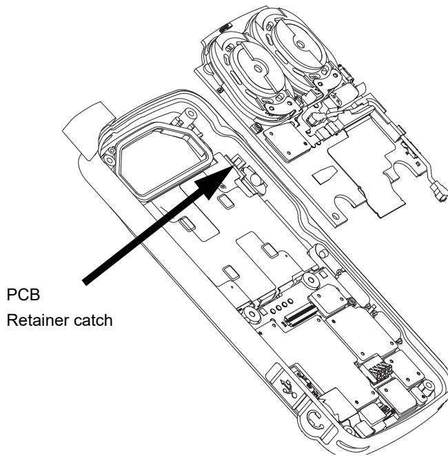
Figure 5-26. Interface board re-assembly
