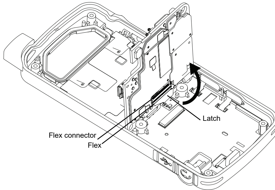
Figure 5-17. PCB board removal
