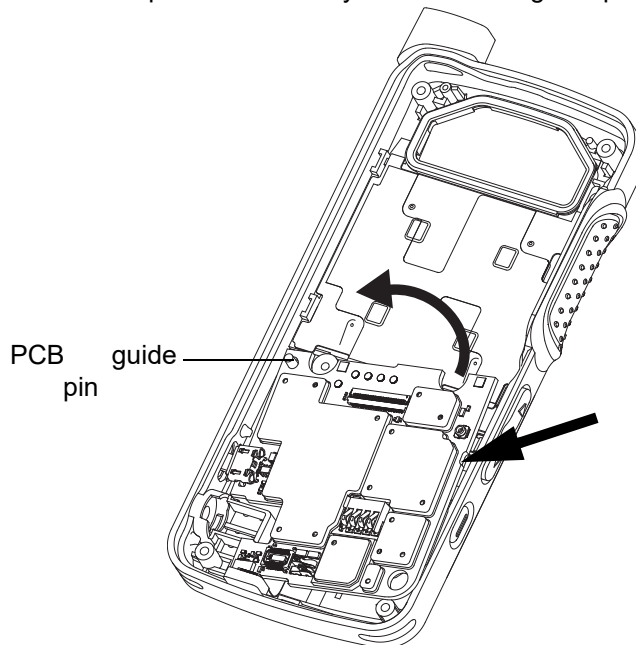
Figure 5-16. Lifting of PCB board
