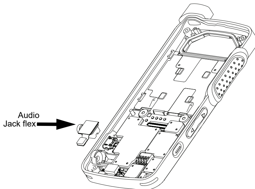
Figure 5-14. Audio jack flex removal
