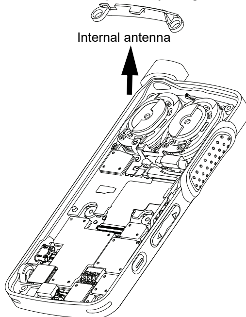
Figure 5-10. Internal antenna removal
