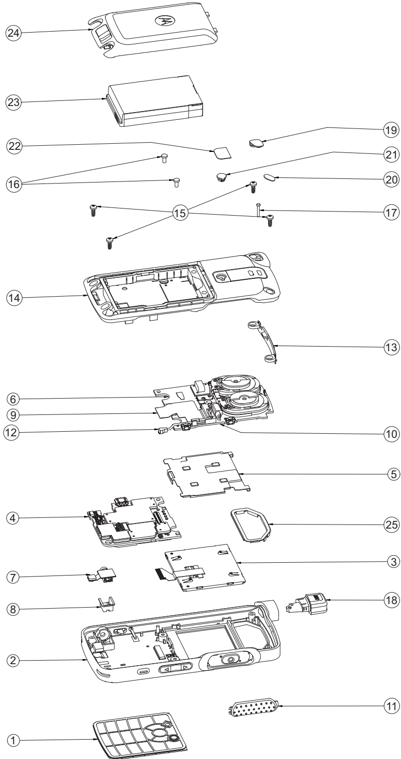
Figure 5-38. 800 MHz Model Exploded View
