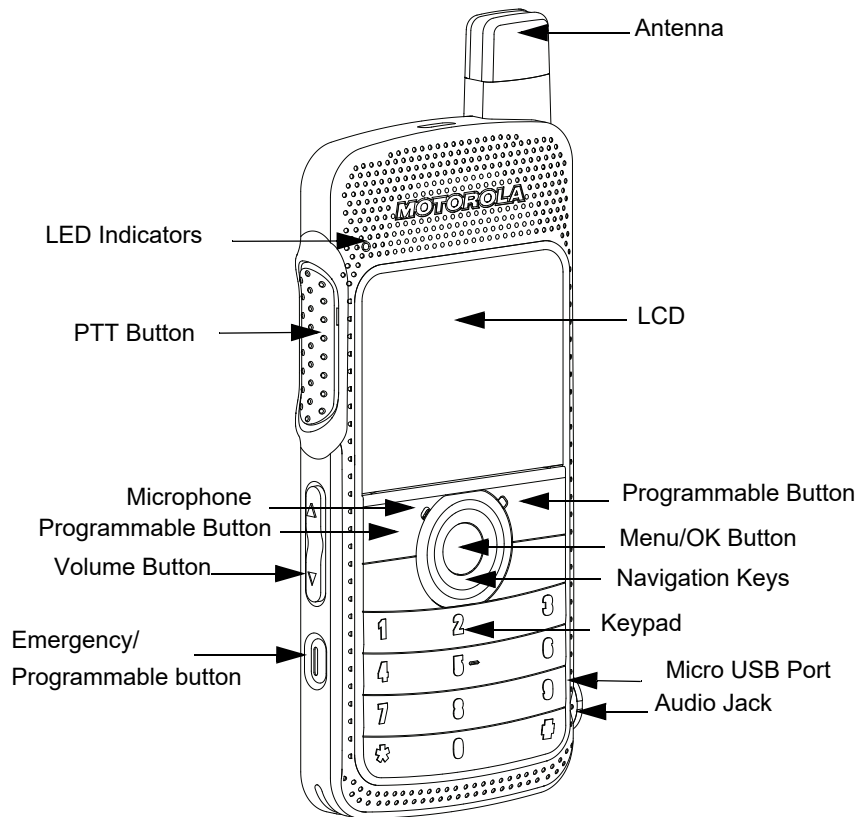
Figure 1-1. Display Model for 800 MHz
