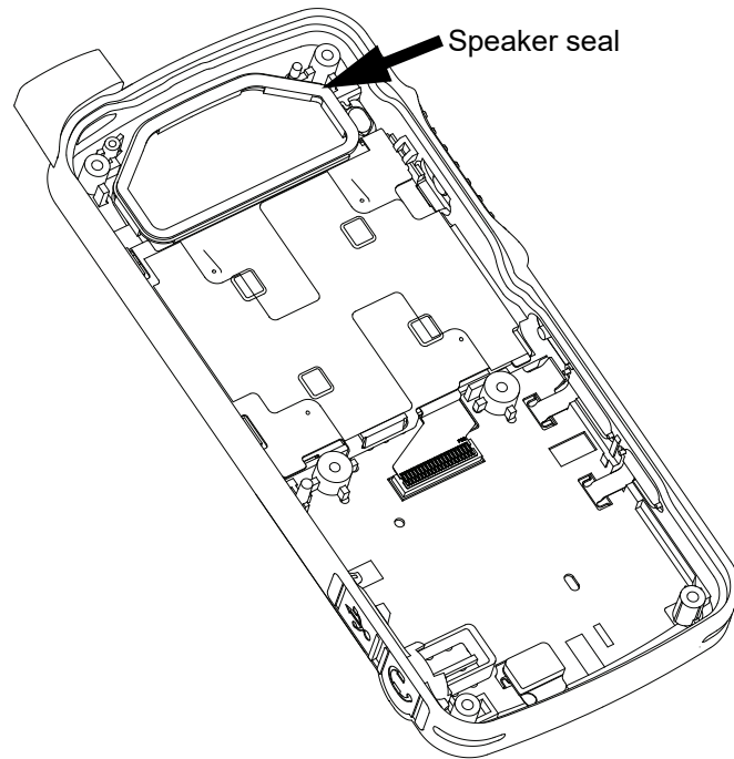
Figure 5-21. Display retainer lock re-assembly
