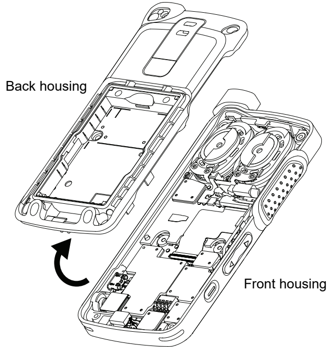
Figure 5-9. Back housing removal
