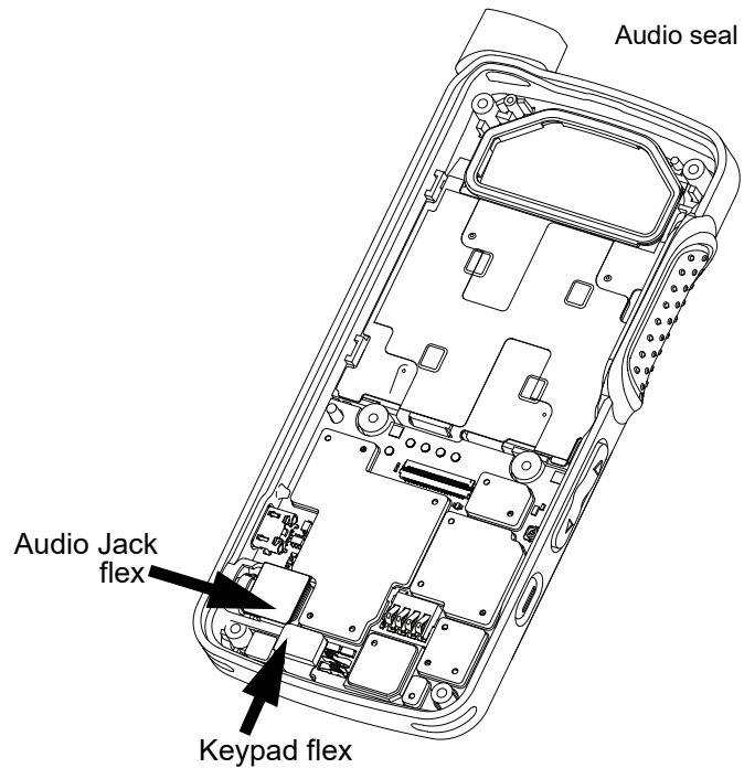
Figure 5-13. Audio jack flex and keypad flex disassembly
