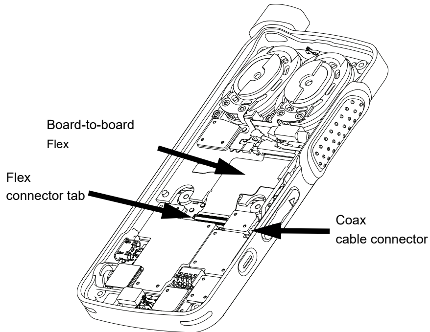
Figure 5-11. Board-to-board flex and coax cable connector disassembly
