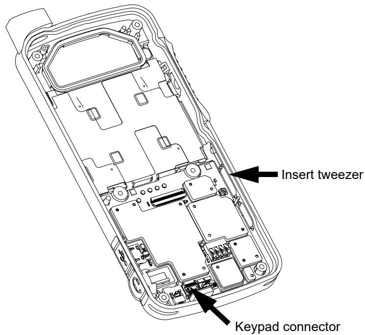
Figure 5-15. LCD display disassembly
