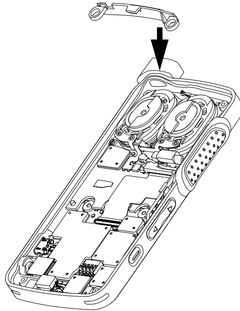
Figure 5-28. Internal antenna re-assembly
