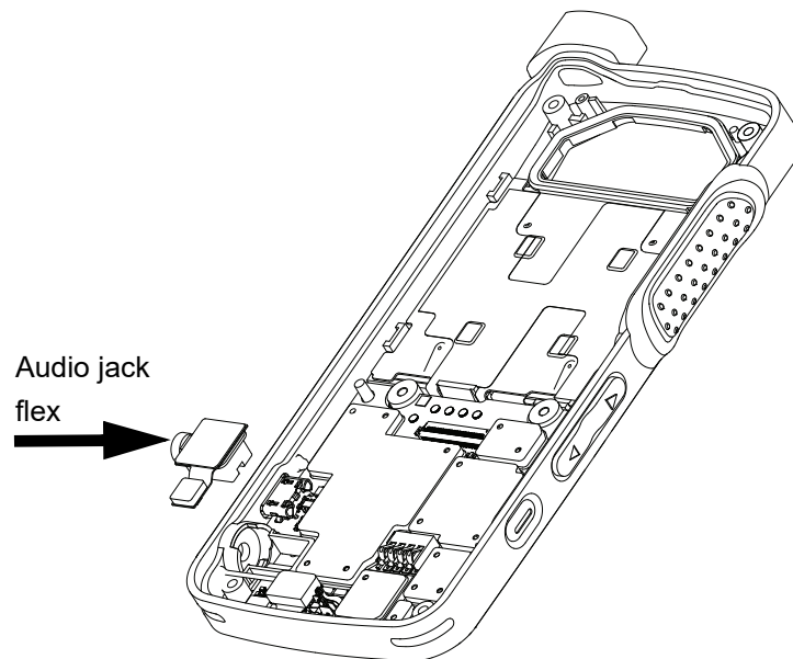
Figure 5-24. Audio jack flex connector re-assembly
