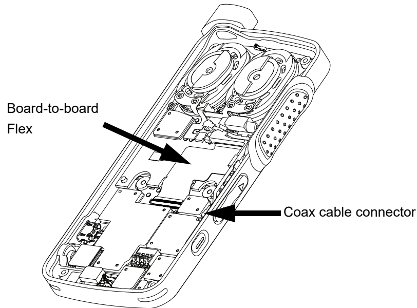
Figure 5-27. Board-to-board flex re-assembly
