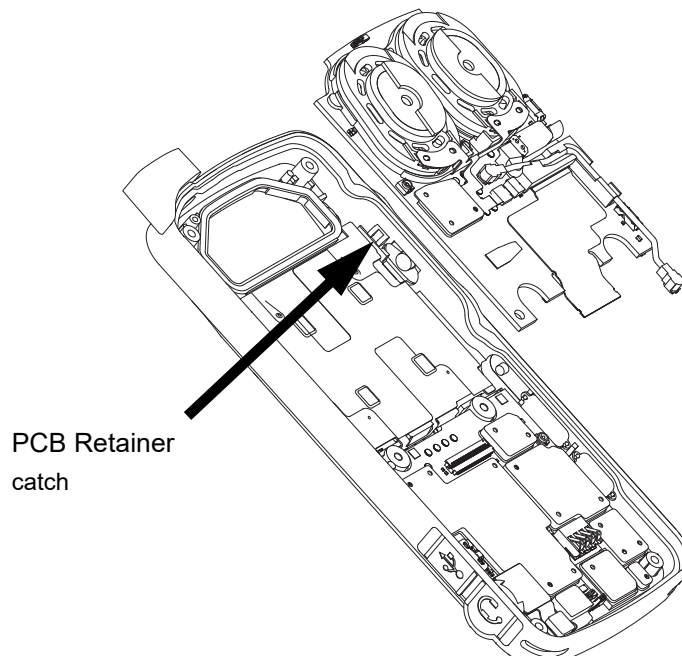
Figure 5-12. Interface board removal
