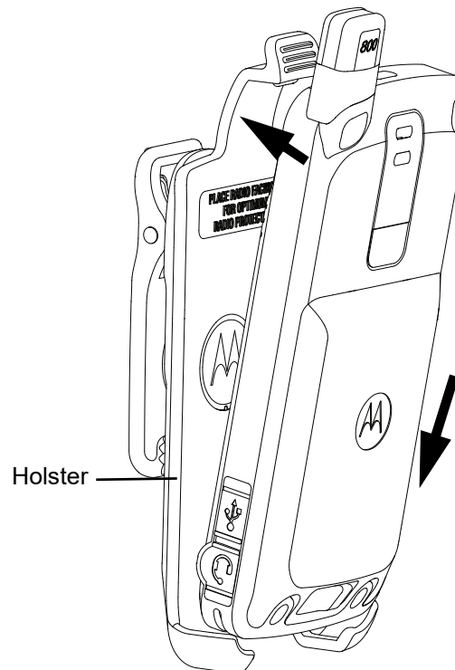
Figure 5-37. Holster re-attachment for 800 MHz
