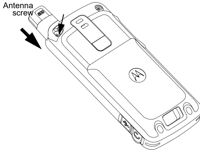
Figure 5-35. Antenna screw re-assembly for 800 MHz
