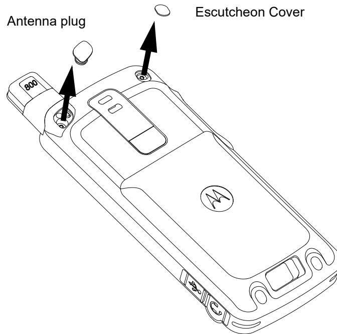
Figure 5-2. Antenna plug and escutcheon cover removal
