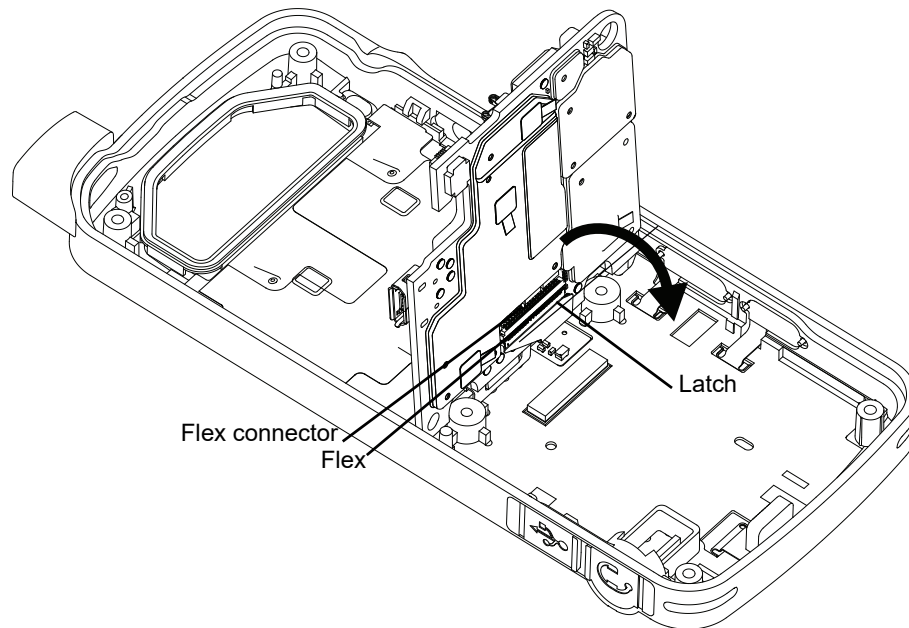
Figure 5-22. Flex connector tab re-assembly
