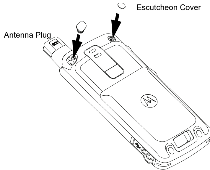
Figure 5-36. Antenna plug and screw plug re-assembly for 800 MHz
