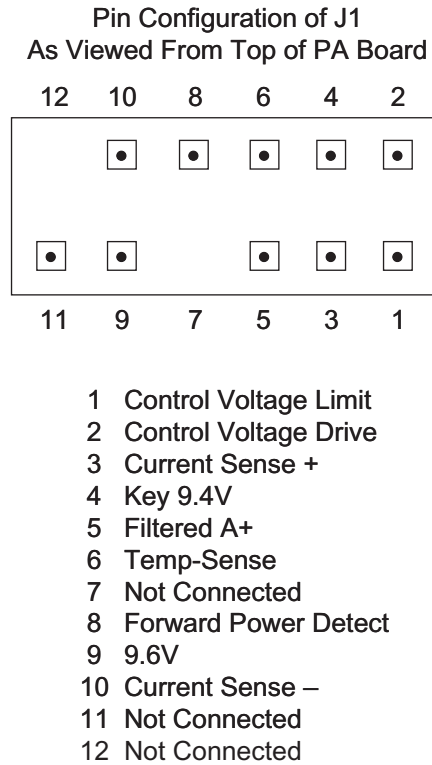
Figure 4-7. Connector Pin-Out—High-Power Amplifier
