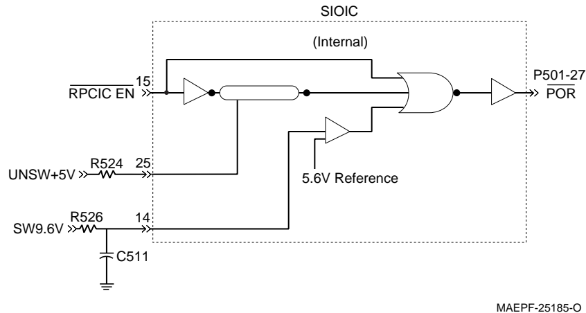
Figure 3-5. Power-on Reset
