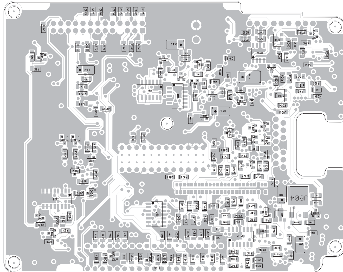
side 1
