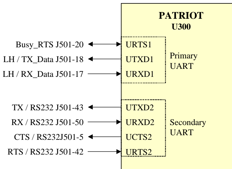
Figure 3-18. ASTRO Spectra Plus Host SB9600 and RS232 Ports
