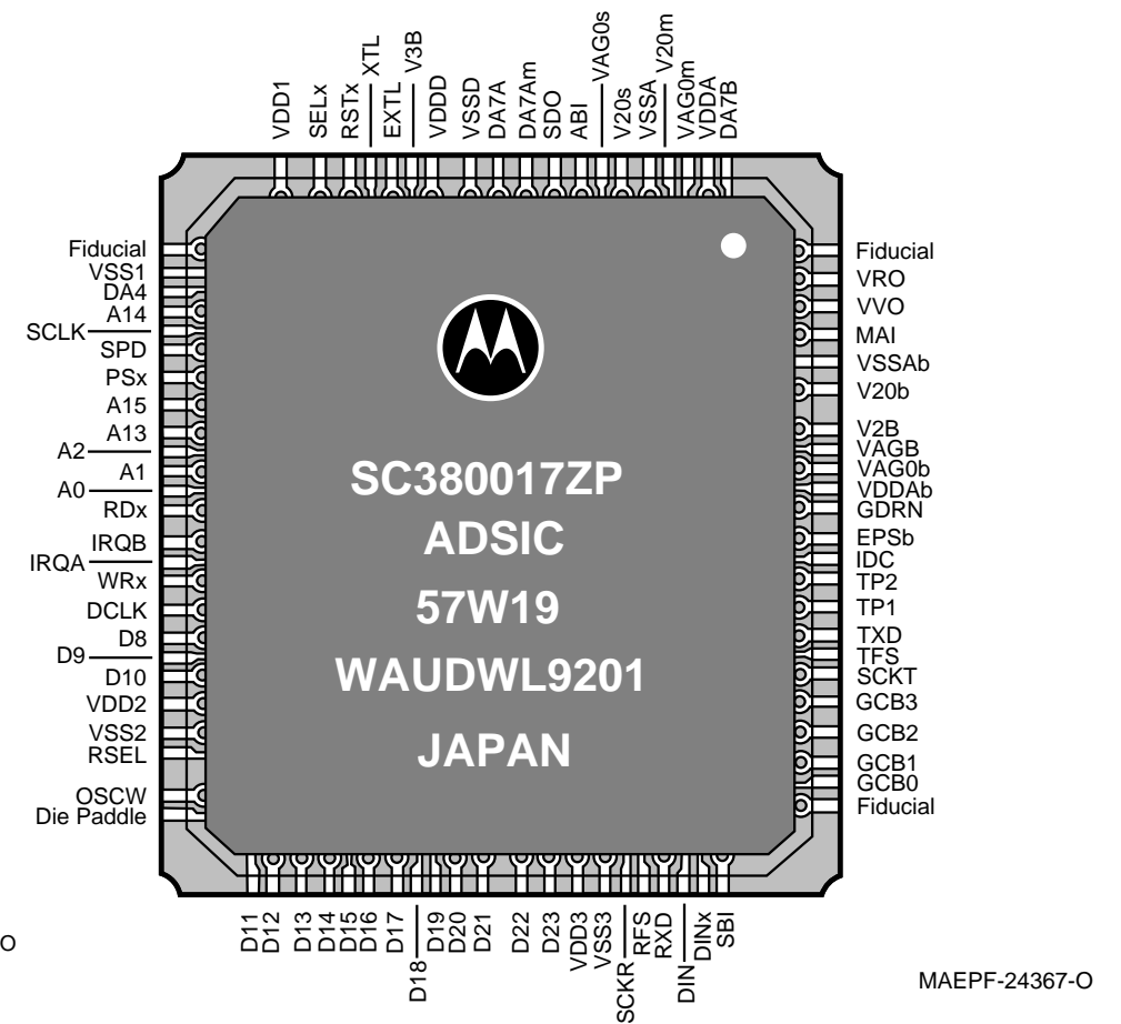
U406 - ADSIC
