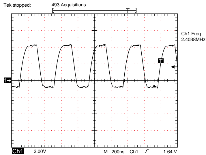
W10 ADSIC 2.4 MHz Reference MAEPF-24385-O Trace 1 - IDC @ U406
