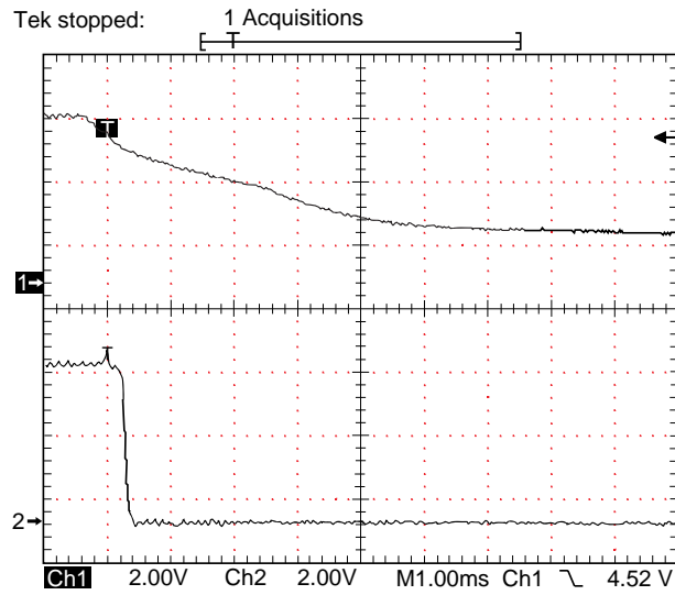
W9: Power Down Reset. MAEPF-24384-O Trace 1 - +5V @ U407 (VDD) Trace 2 - Reset @ U407 (OUT)
