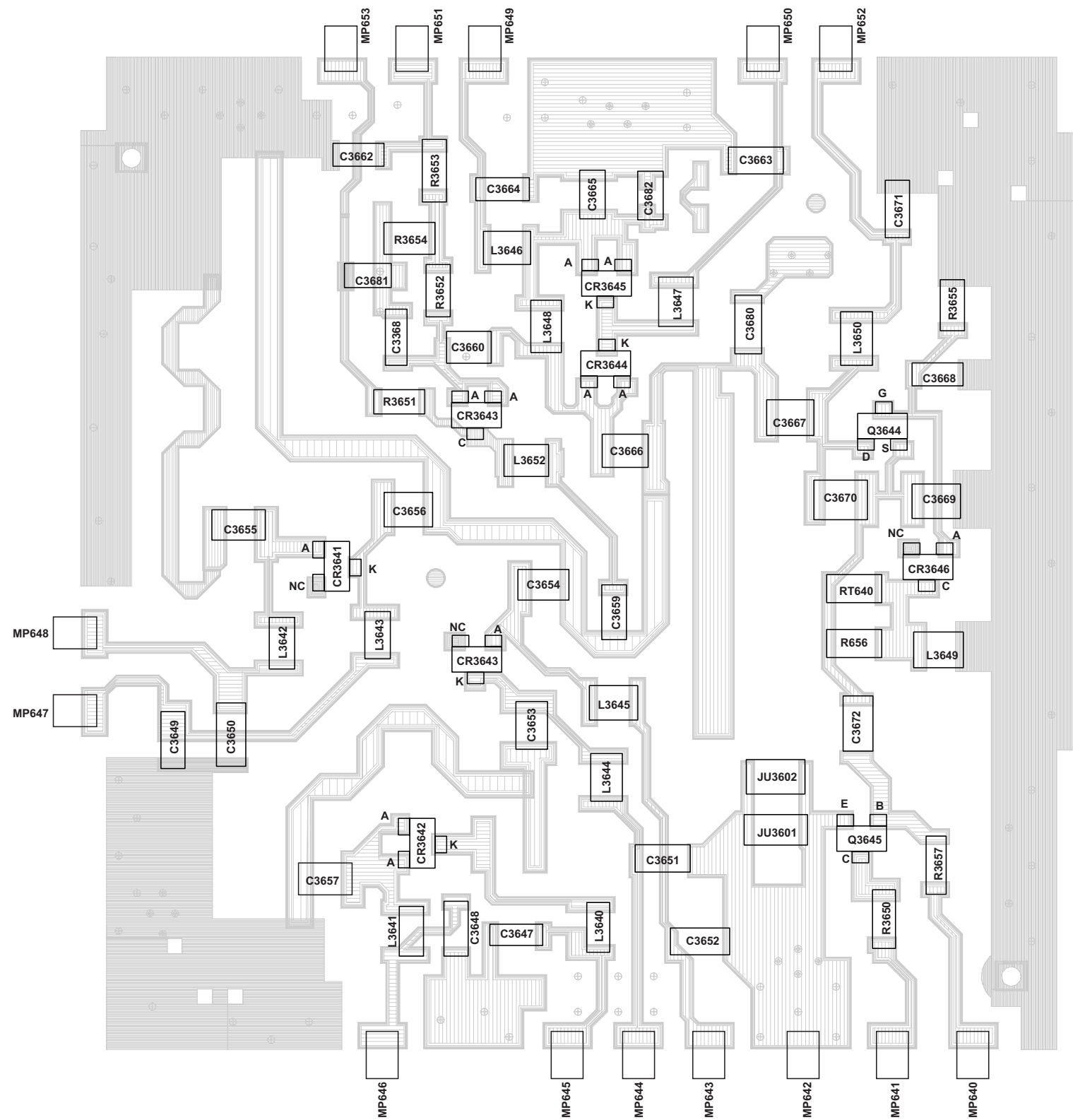
HLD6061D and HLD6062D VHF VCO Hybrid Component Location Diagram
