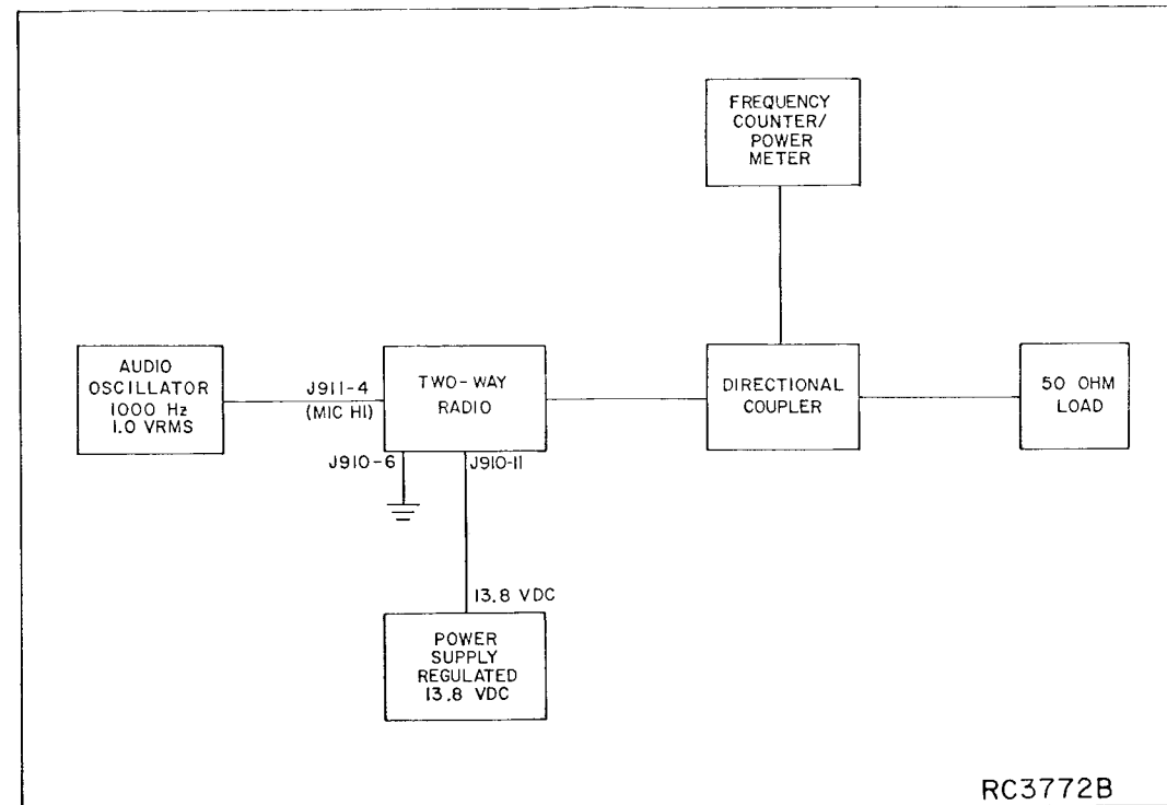
Figure 4 - Transmitter Alignment
