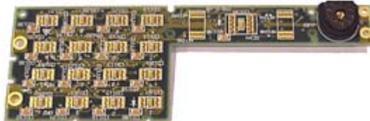
B19/CDF-368MC Switch Board, System System Control Units
