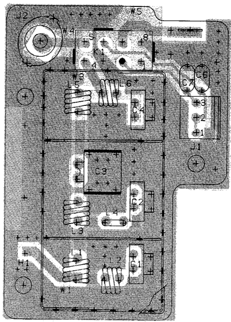
FILTER BOARD
