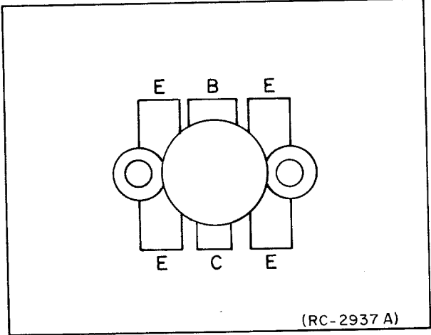
Figure 2 - Lead Identification
